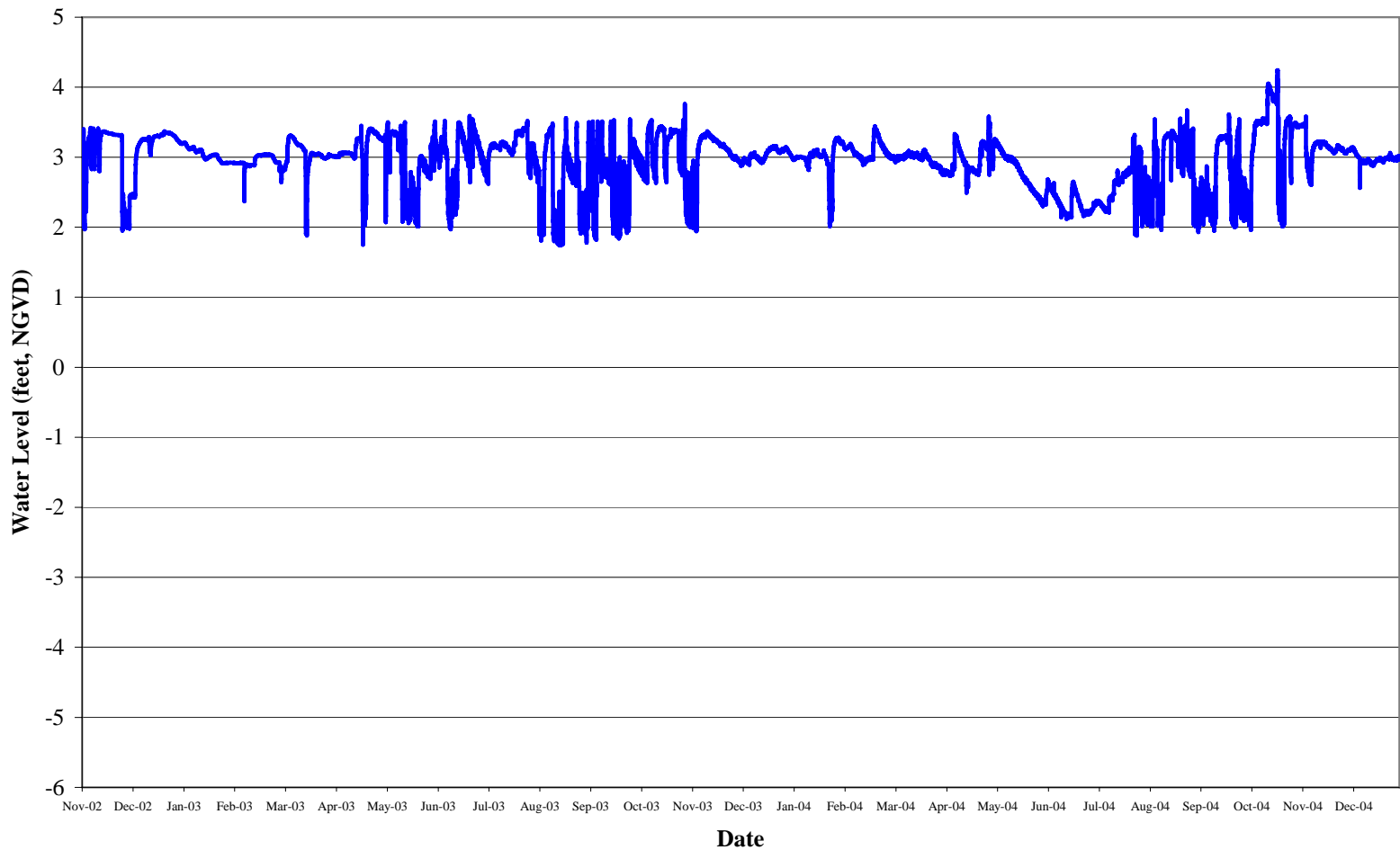
Hydrograph for C2SW2
