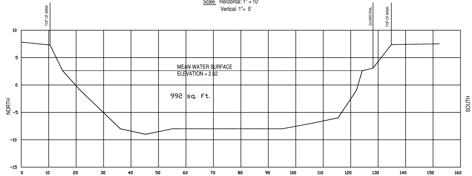
CROSS SECTION # 2 Scale: Horizontal: 1" = 10' Vertical: 1" = 5'
