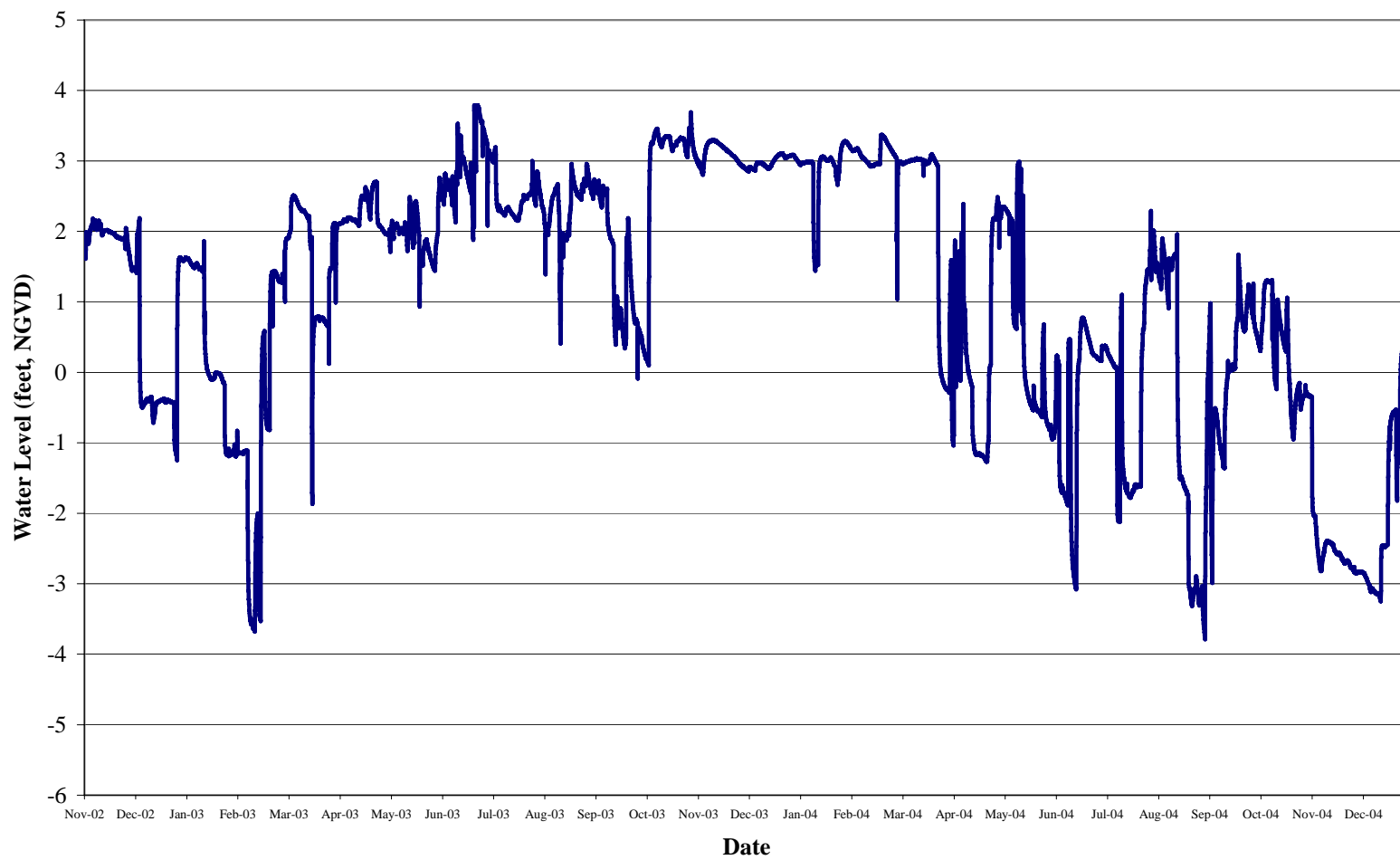
Hydrograph for C2GW1_GW1
