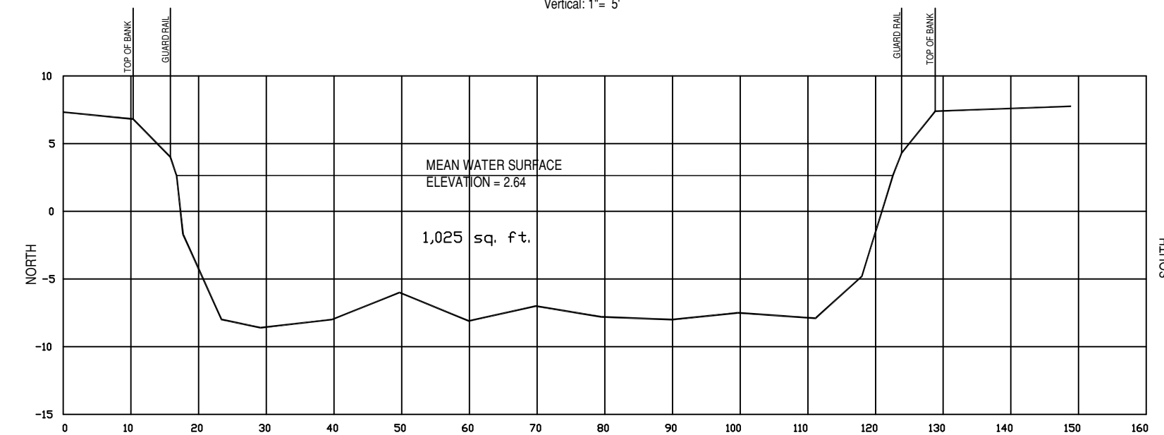
CROSS SECTION # 3 Scale: Horizontal: 1" = 10' Vertical: 1" = 5'
