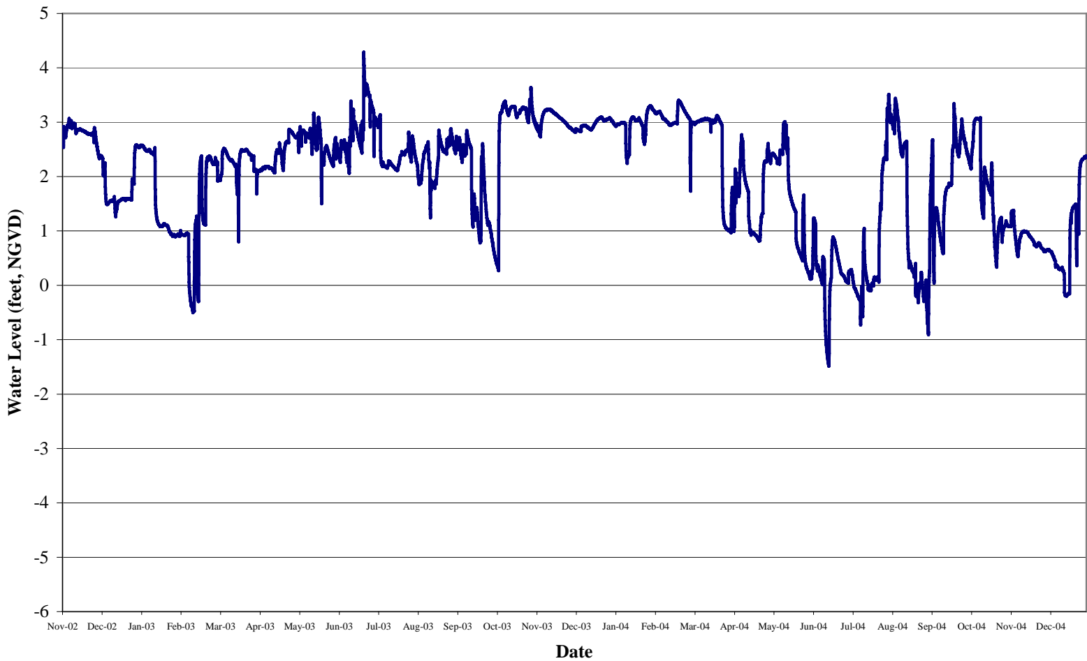
Hydrograph for C2GSW1_GW1
