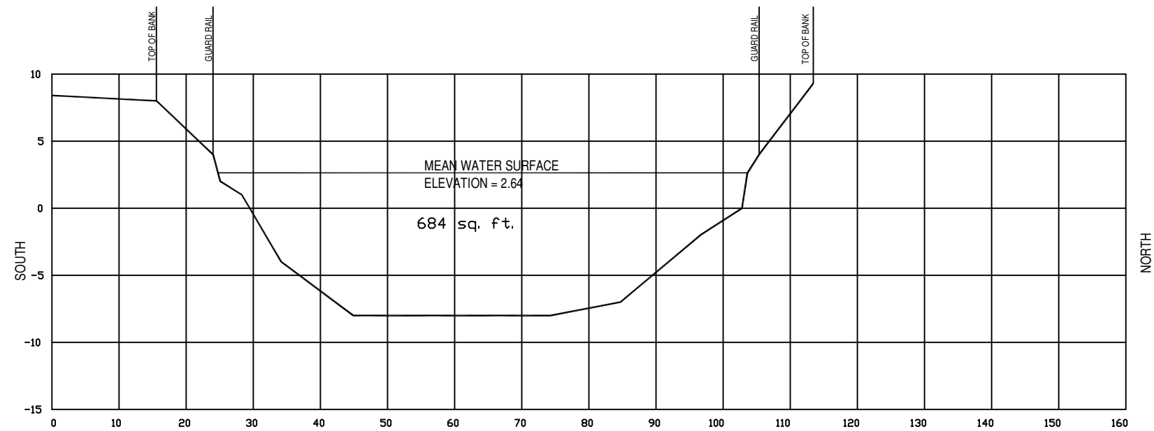
CROSS SECTION # 1 Scale: Horizontal: 1" = 10' Vertical: 1" = 5'
