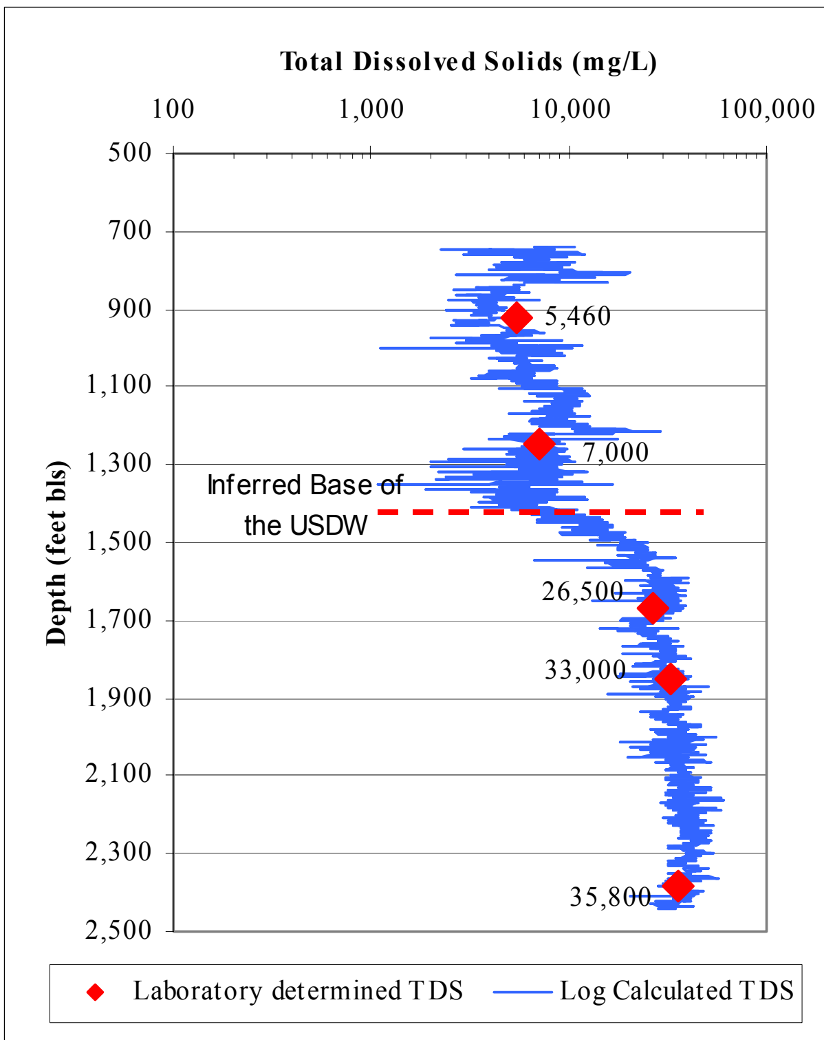
Figure 7. Calculated Formation Water Resistivity Log – BICY-TW (830-2,450 feet bls).
