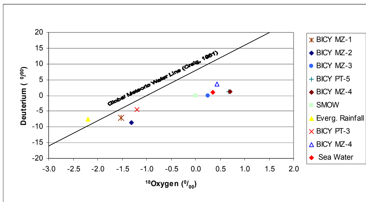
Figure 9. Cross-Plot of Deuterium and ^{18}\text{O} xygen – Stable Isotopes.
