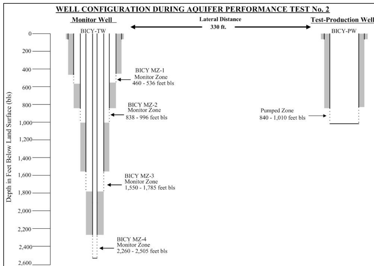
Figure 17. Aquifer Performance Test – Well Configuration APT No. 2.
