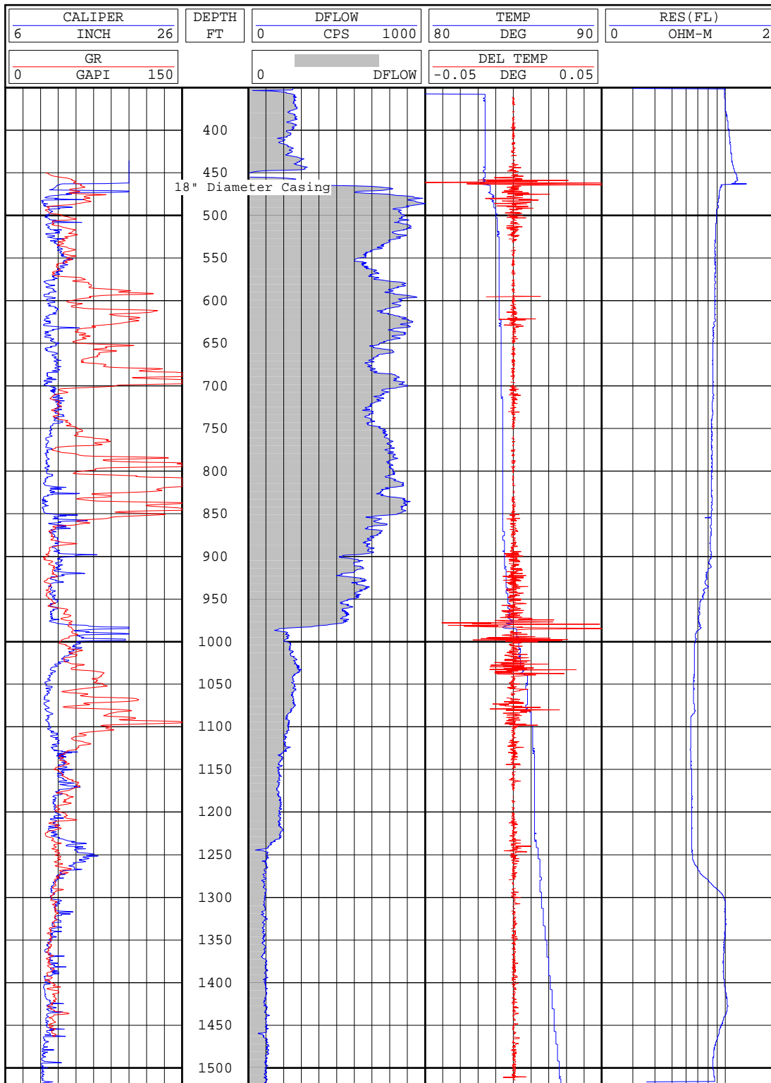
Production Log Data – Geophysical Run No. 1
