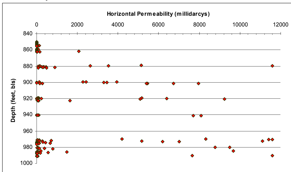
Figure 11. Laboratory Permeability Distribution of Upper Floridan Production Zone.
