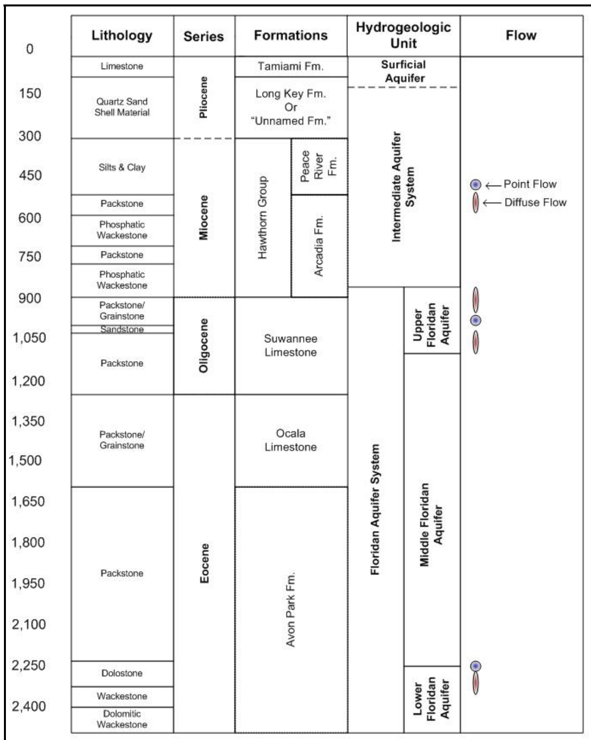
Figure 6. Generalized Hydrogeologic Section.
