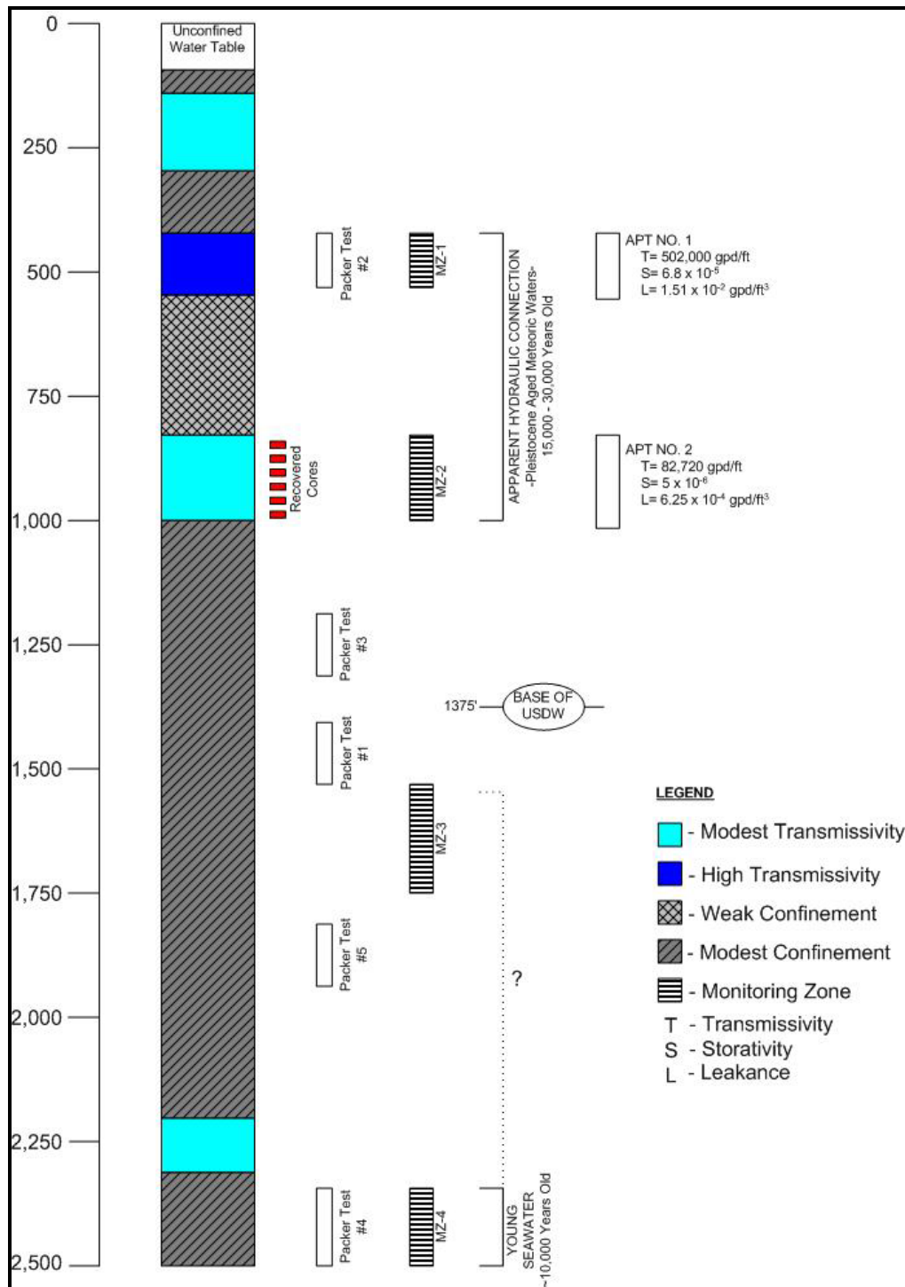
Figure 12. Hydrogeologic Testing – Data Summary Diagram.
