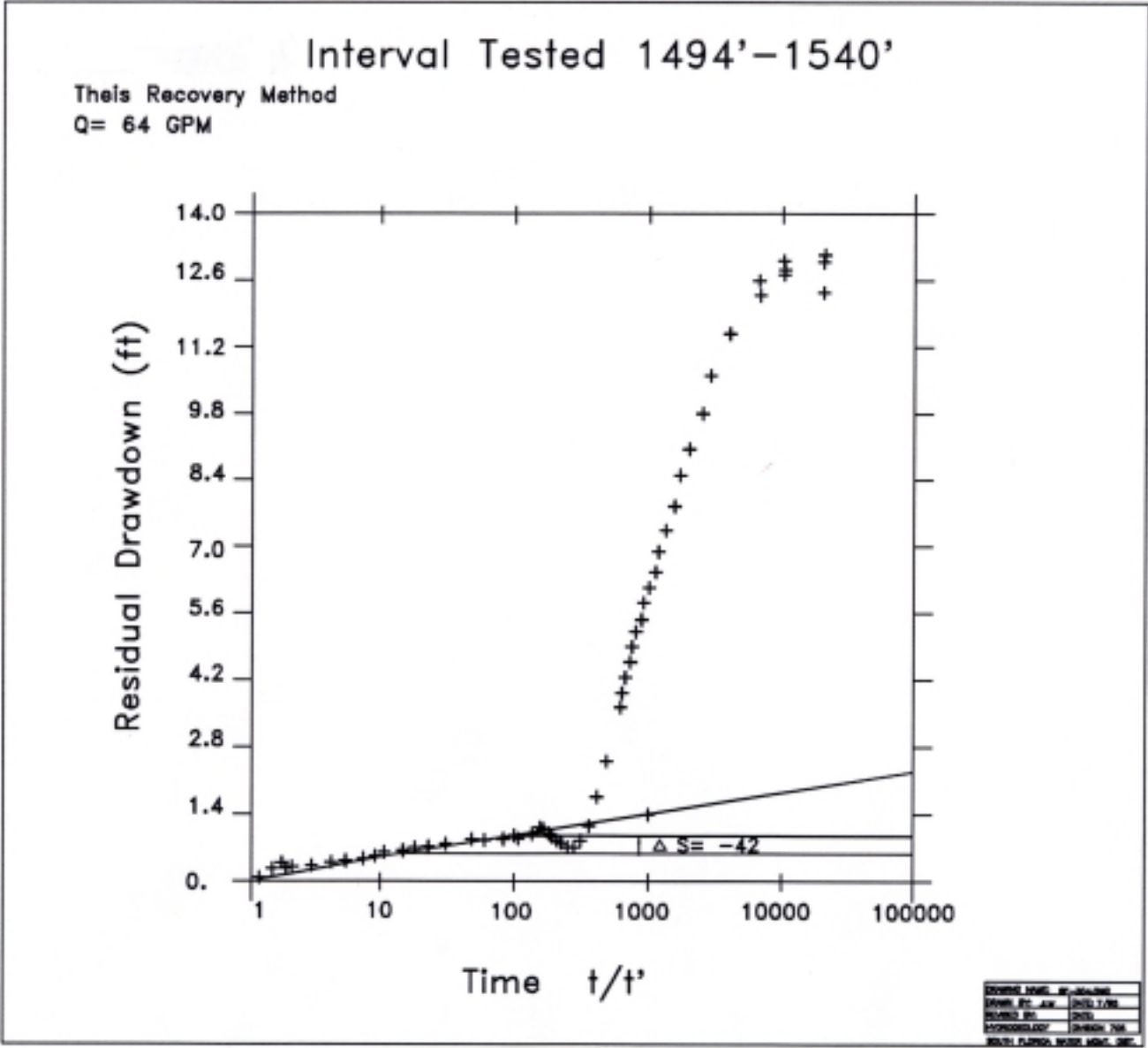
Figure C.5 – Straddle-Packer Test No. 5 – (1,494-1,540' bis)
