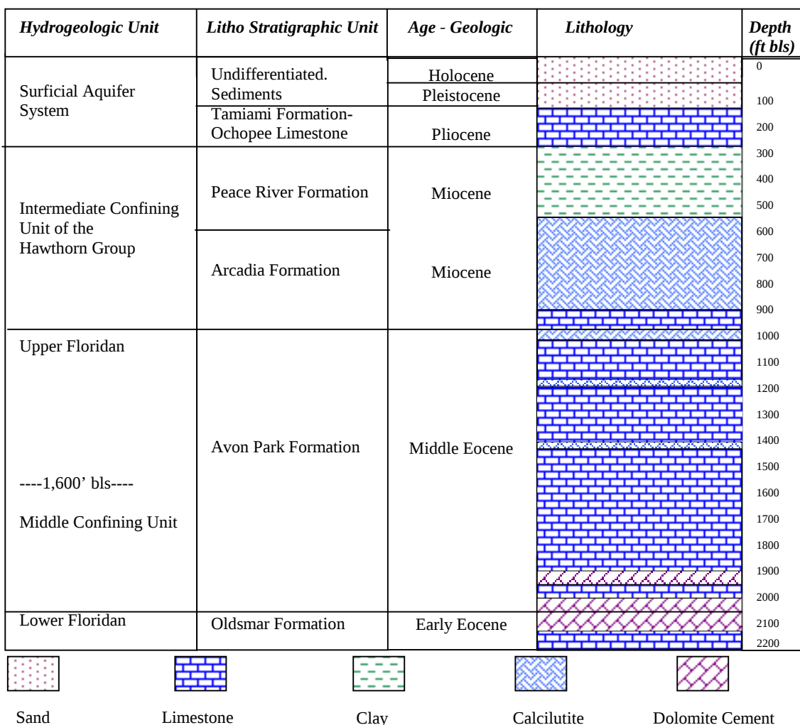
Figure 4. Hydrostratigraphic Summary Diagram.
