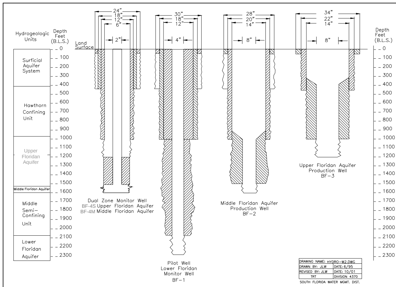
Figure 3. Well Construction Designs.
