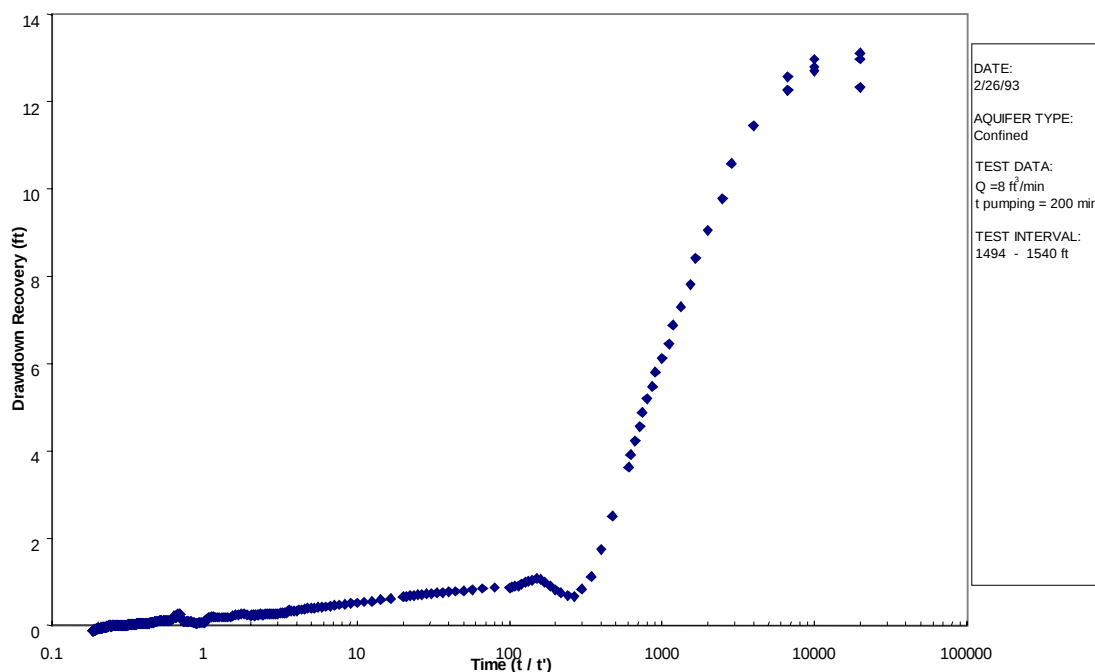
Figure 12. Packer Test Number 5, Recovery Data (1,494-1,540 feet bls).
