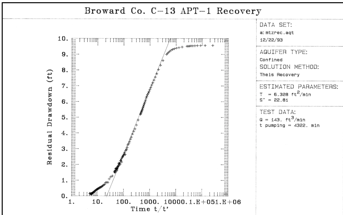
Figure 16. APT-1, Semi-Log Plot of Time Drawdown During Recovery Phase (Middle Flow Zone).
