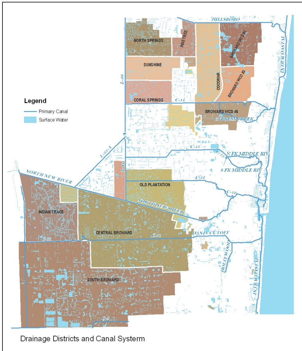
Figure 1: Primary Canals and Drainage/Water Control Districts in Broward County
