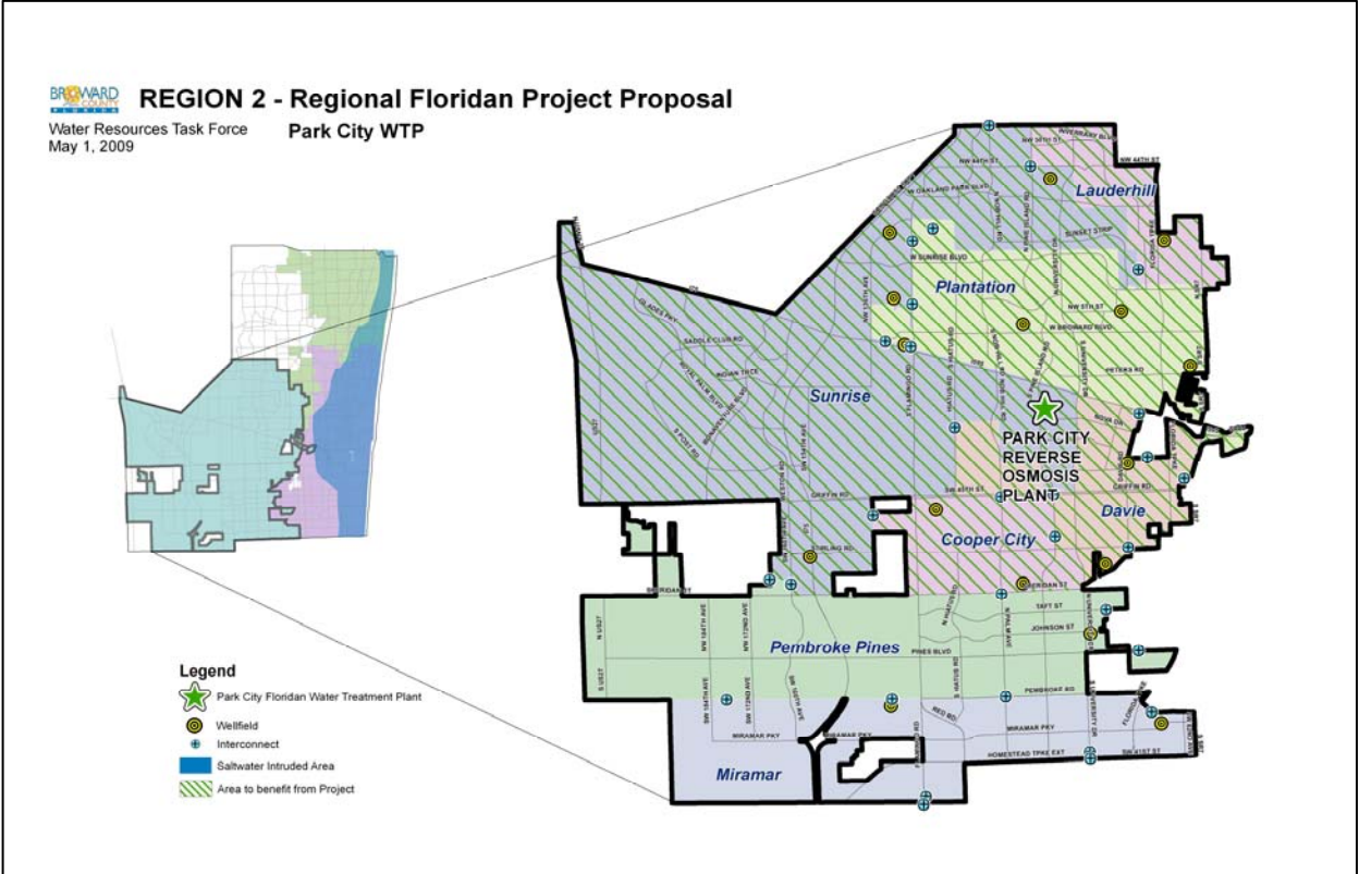
Figure 12: Region 2 Regional Floridan Project
