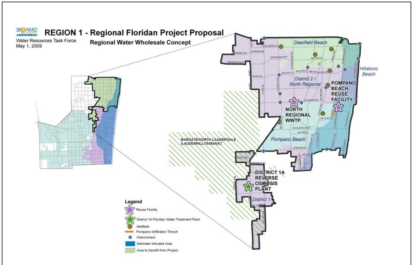
Figure 9: Region 1 Floridan Project
