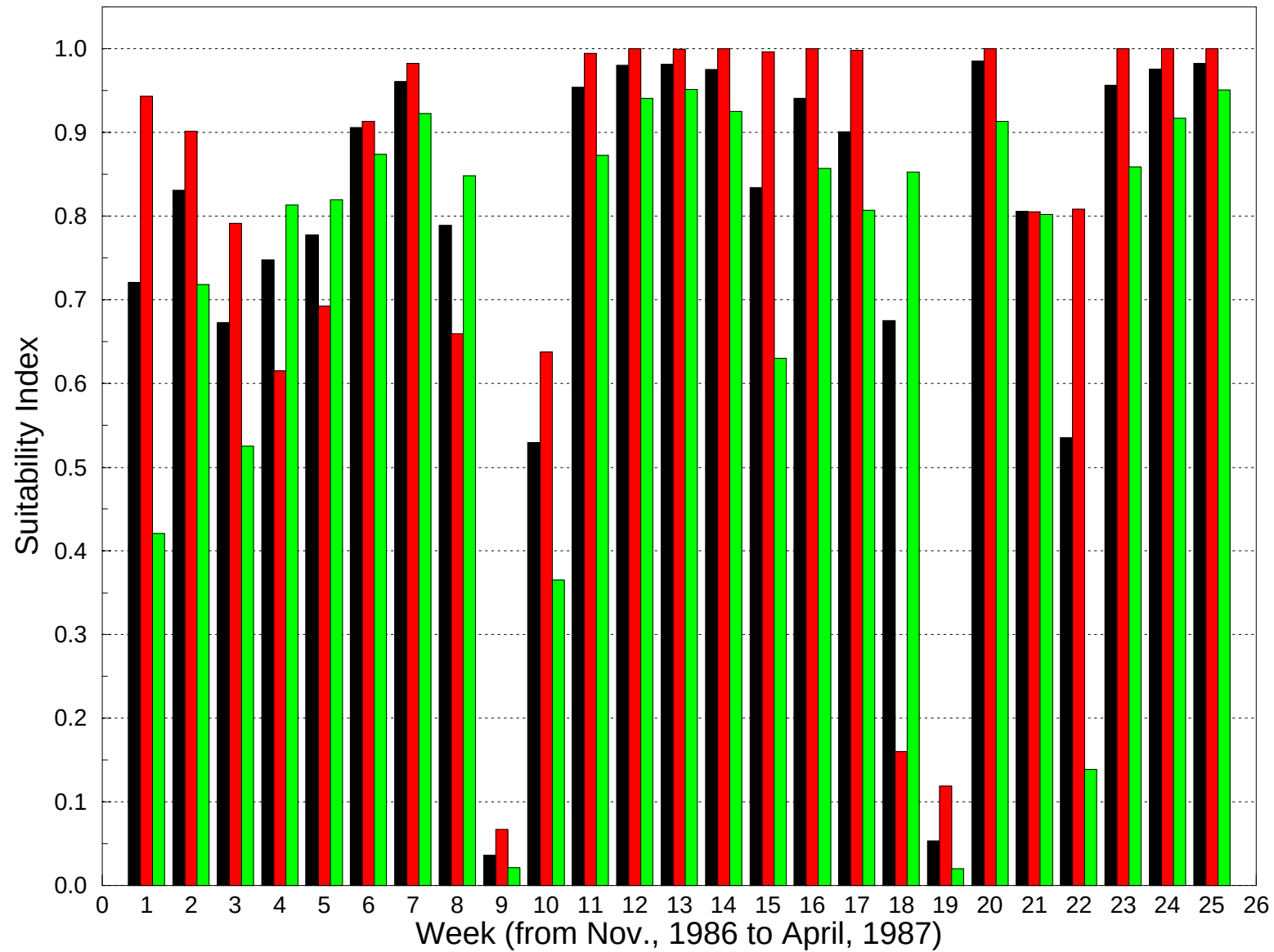
Overall Suitability Index: Area Suitability in the Remnant Everglades
