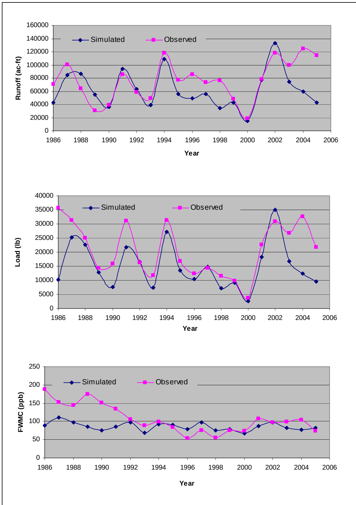
Figure 4-2: Shingle Creek Basin Simulated and Observed Annual Runoff, Load and TP FPMC
