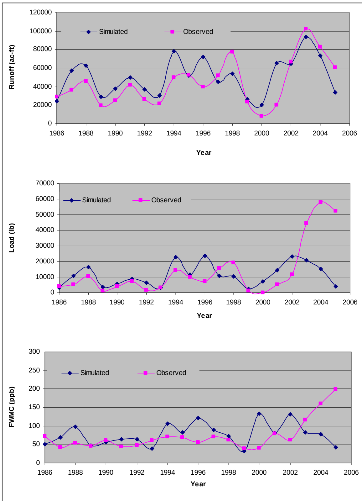
Figure 4-1: Upper Reedy Creek Basin Simulated and Observed Annual Runoff, Load and TP FPMC
