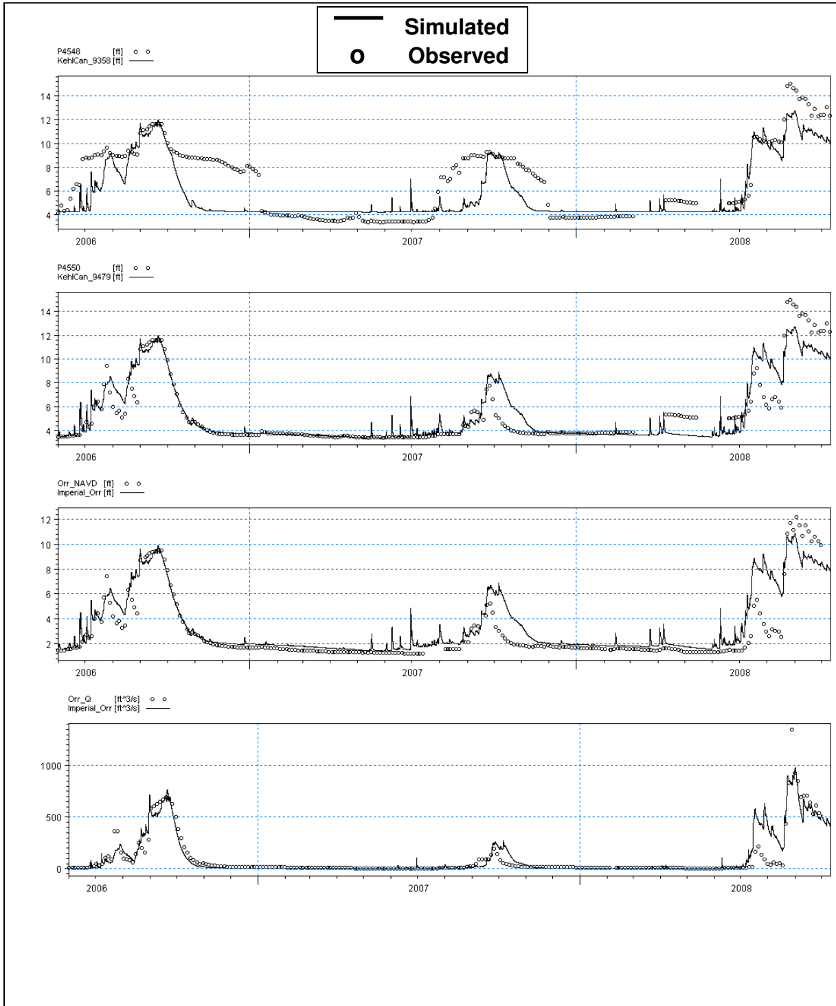
Figure 2-19: Calibration Plots for the Imperial River
