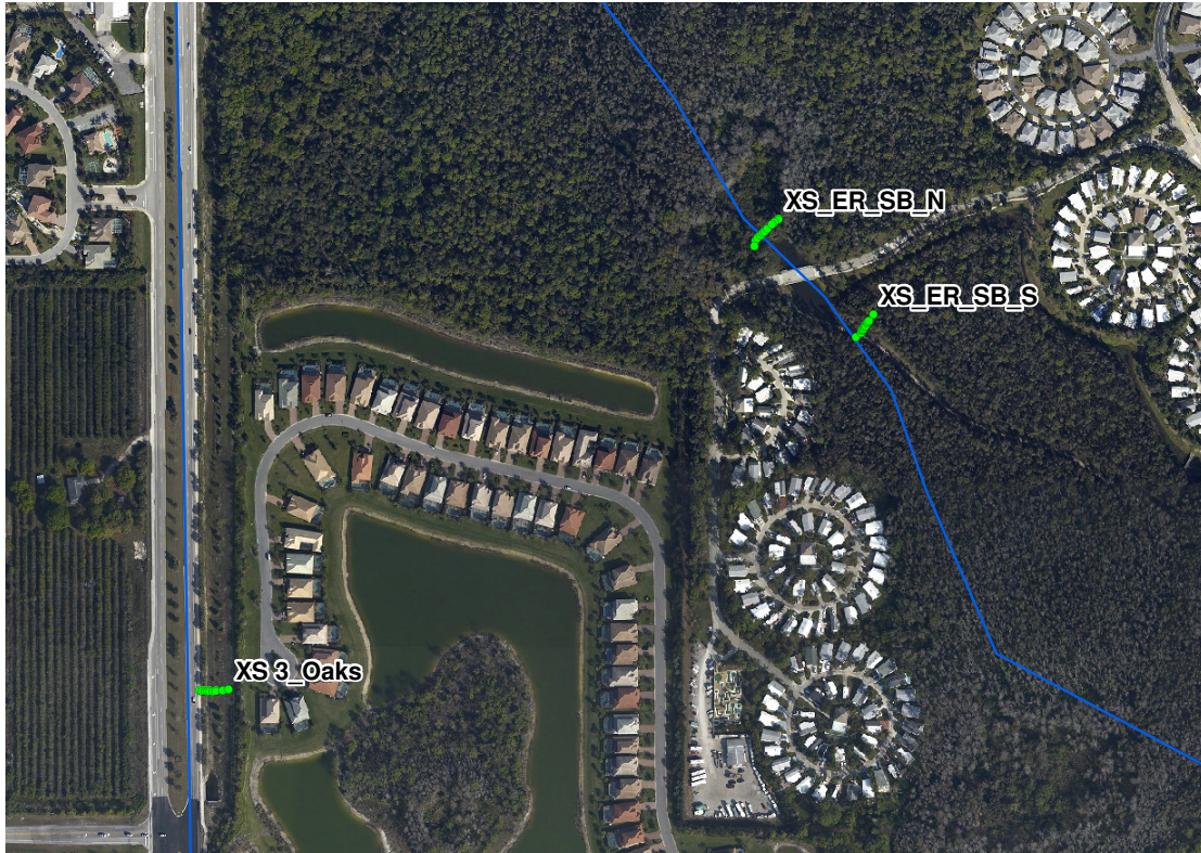
Figure 1-11b: Map of Cross Sections Surveyed by Boyle Engineering
