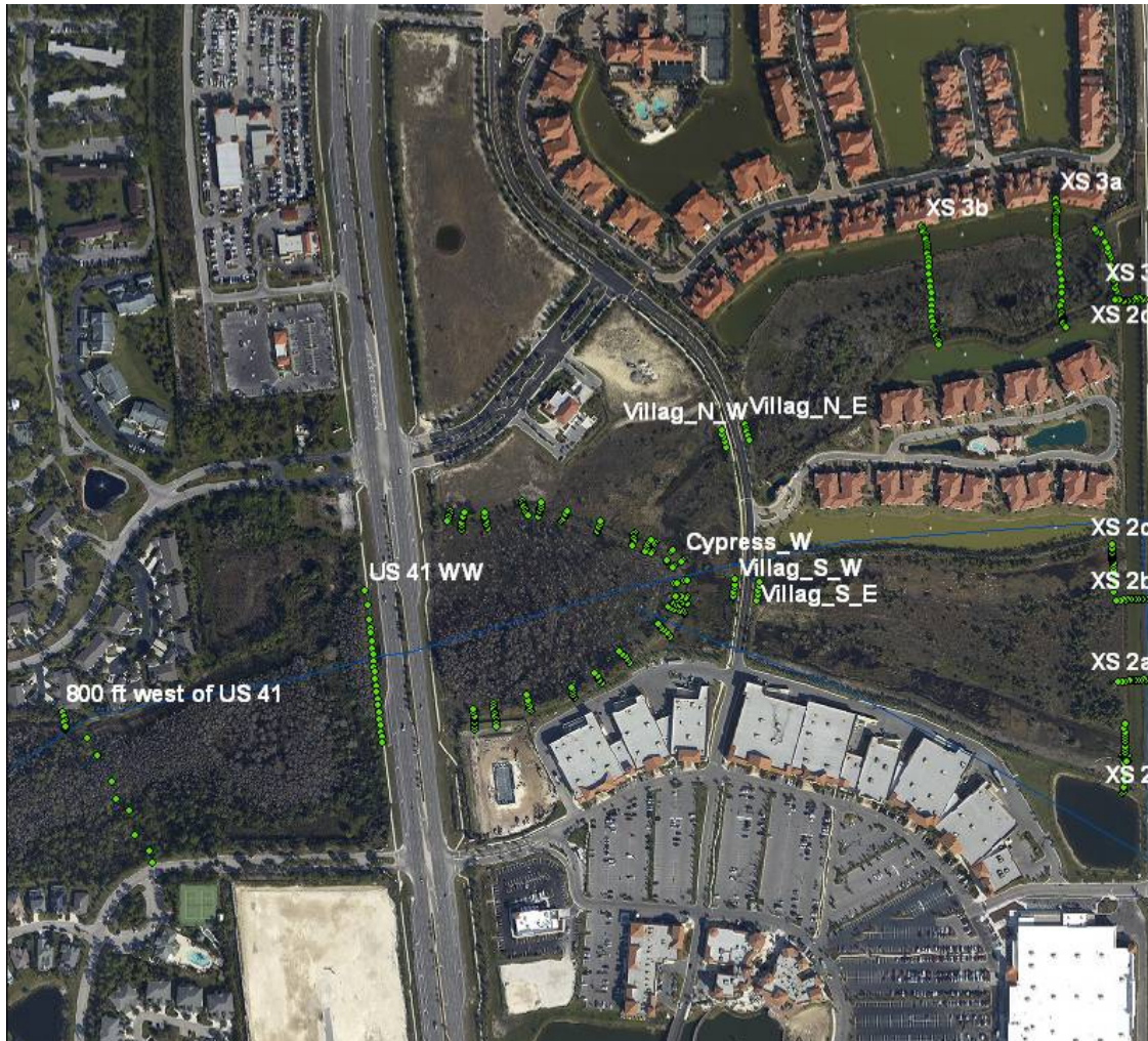
Figure 1-11a: Map of Cross Sections Surveyed by Boyle Engineering
