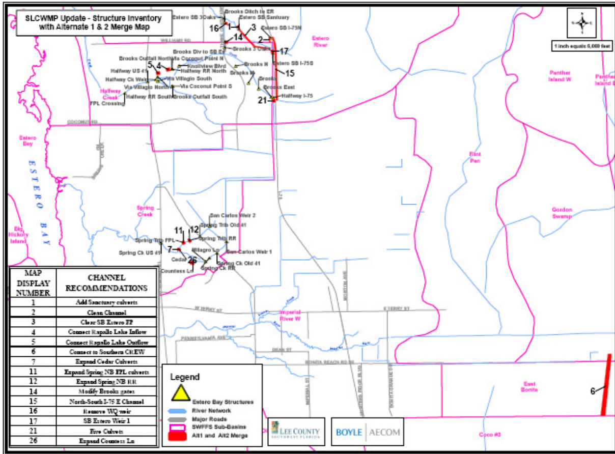
Figure 5-15: Alternatives 1 and 2 Map
