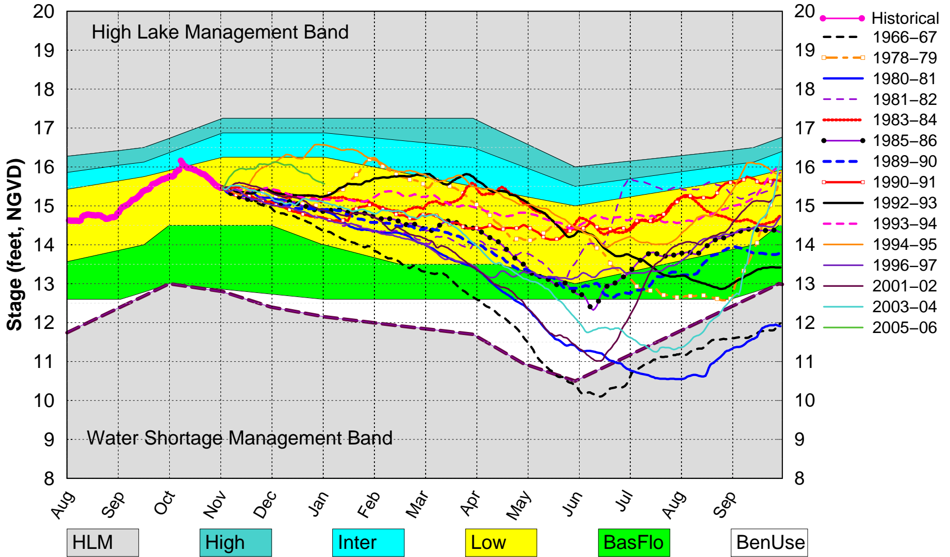
All ENSO Neutral Years Plot PA_DPA
