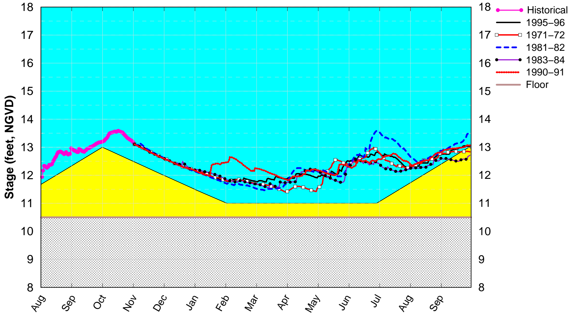
Wet Years Plot PA_DPA
