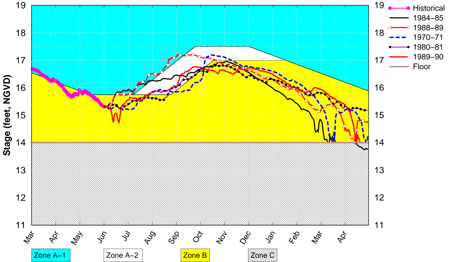
PA_DPA2 Dry Years Plot
