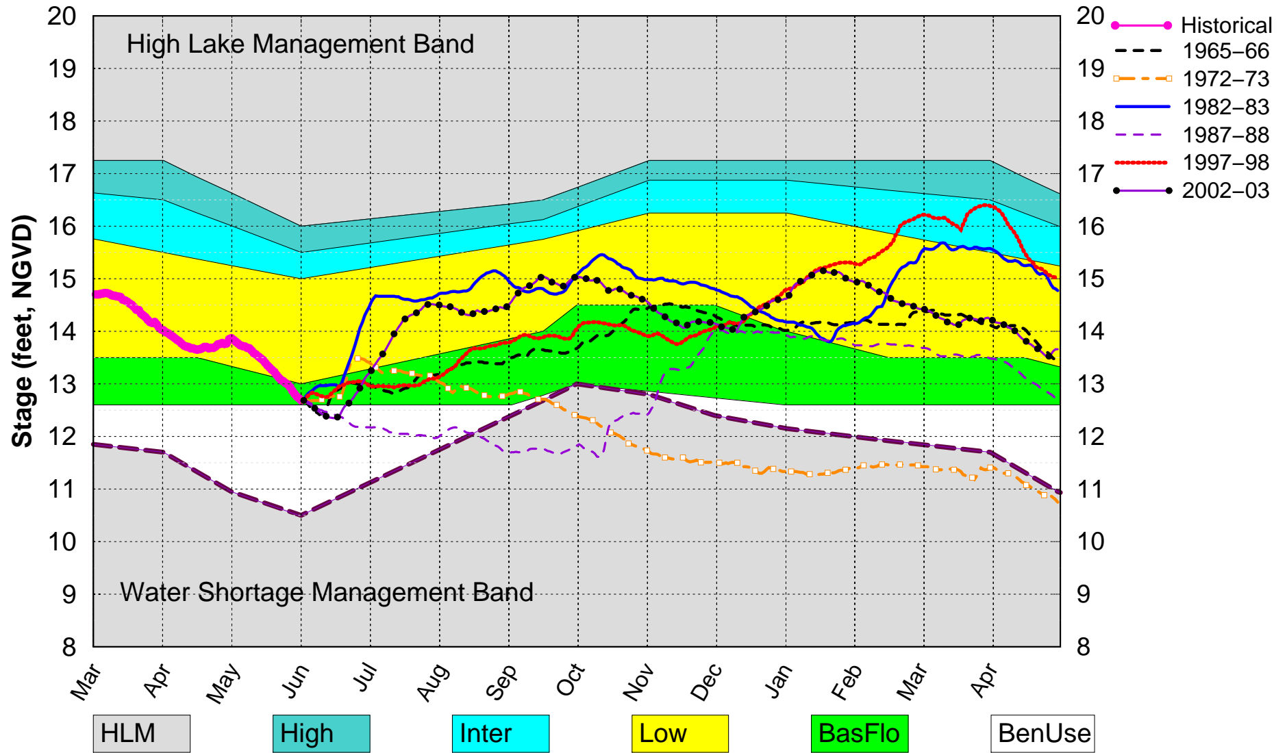
All El Nino Years Plot PA_DPA2
