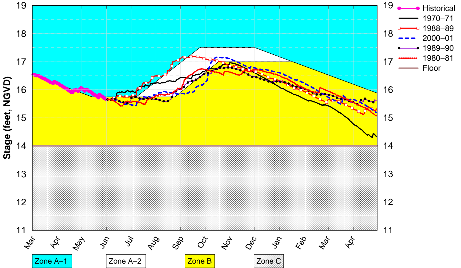
Dry Years Plot PA_DPA2
