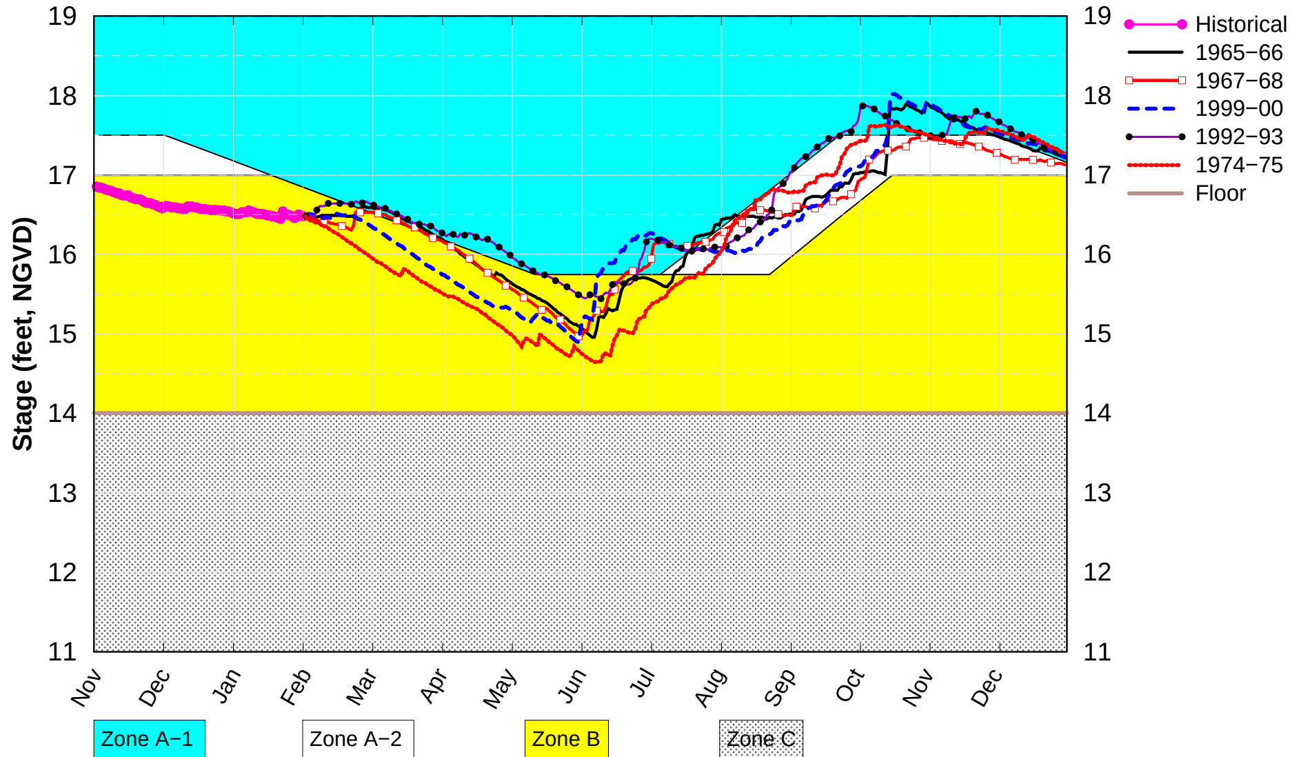
Dry Years Plot PA_SLP1
