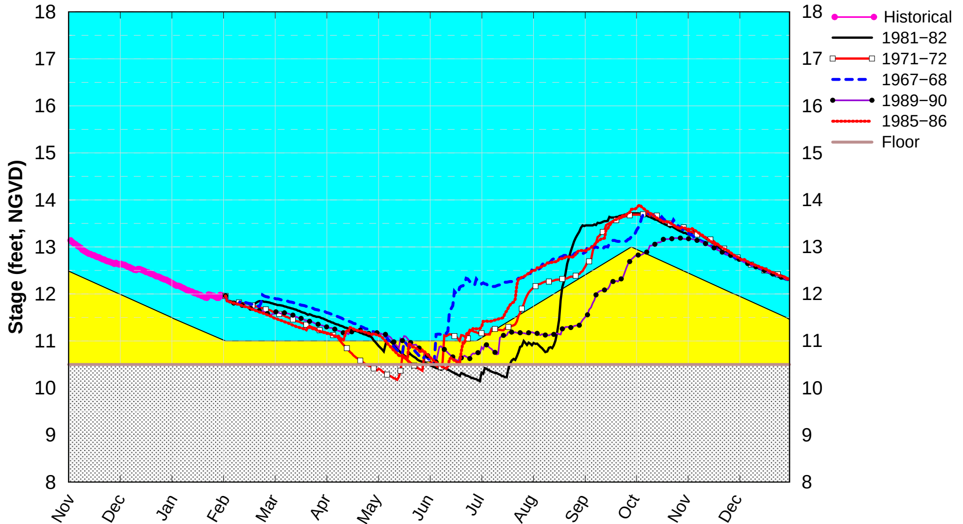
Dry Years Plot PA_SLP1
