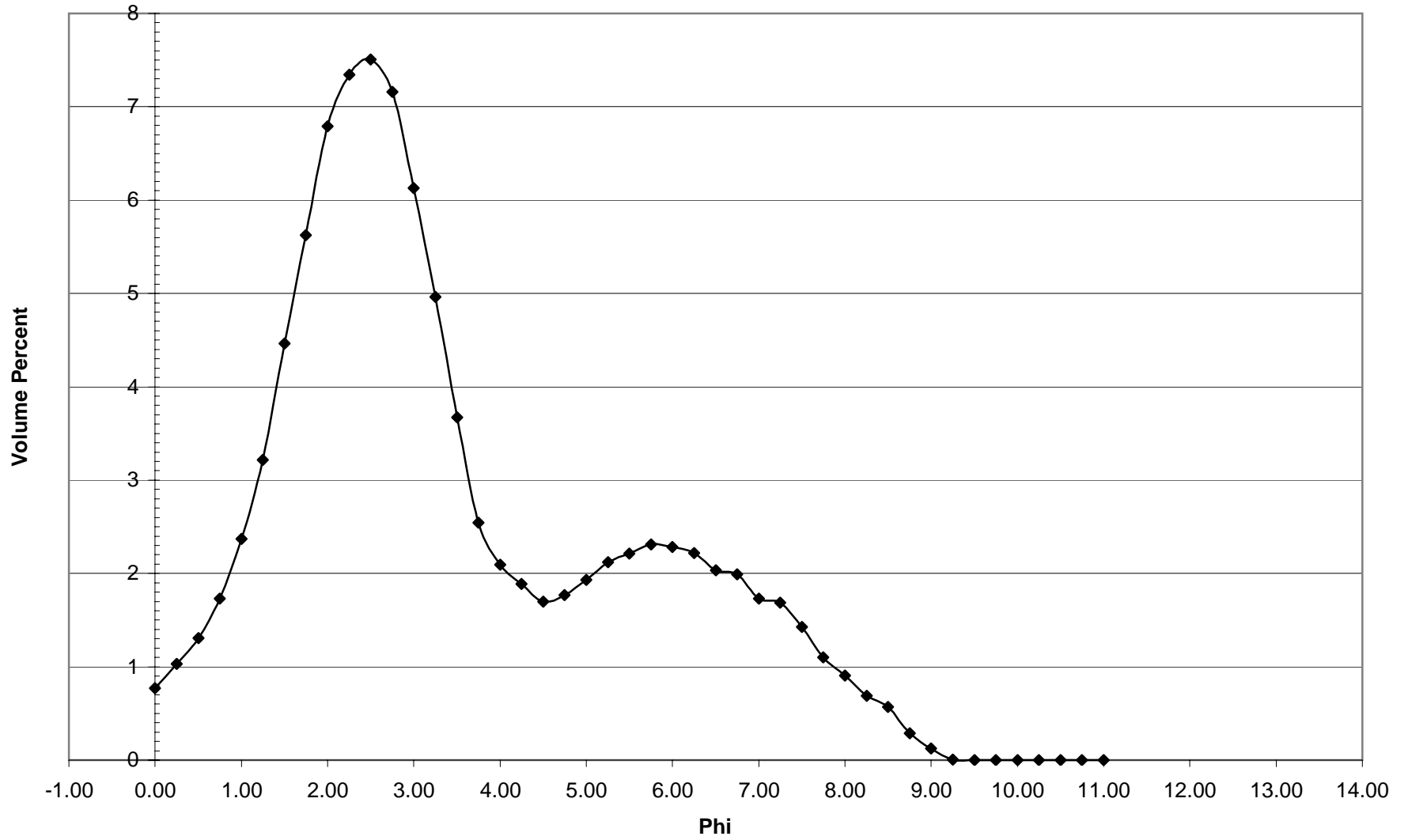
DB-57 Histogram
