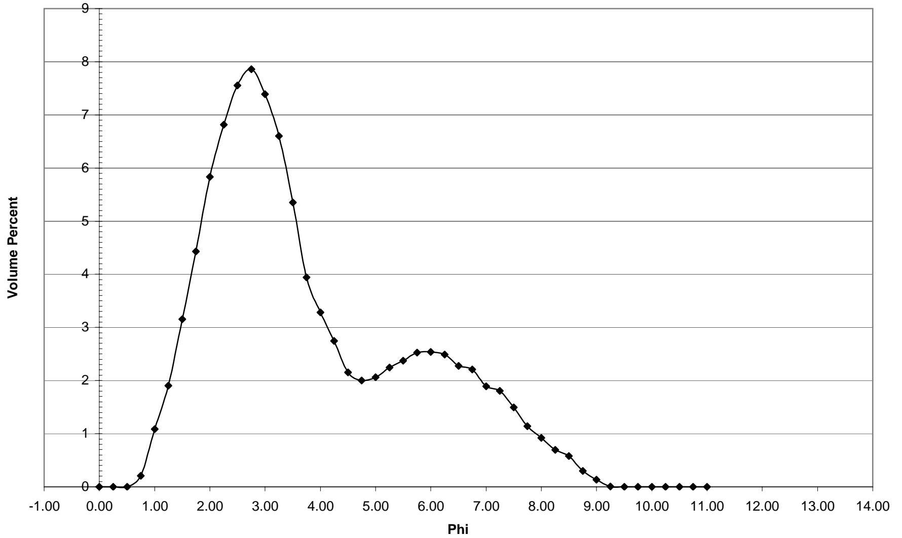
DB-55 Histogram
