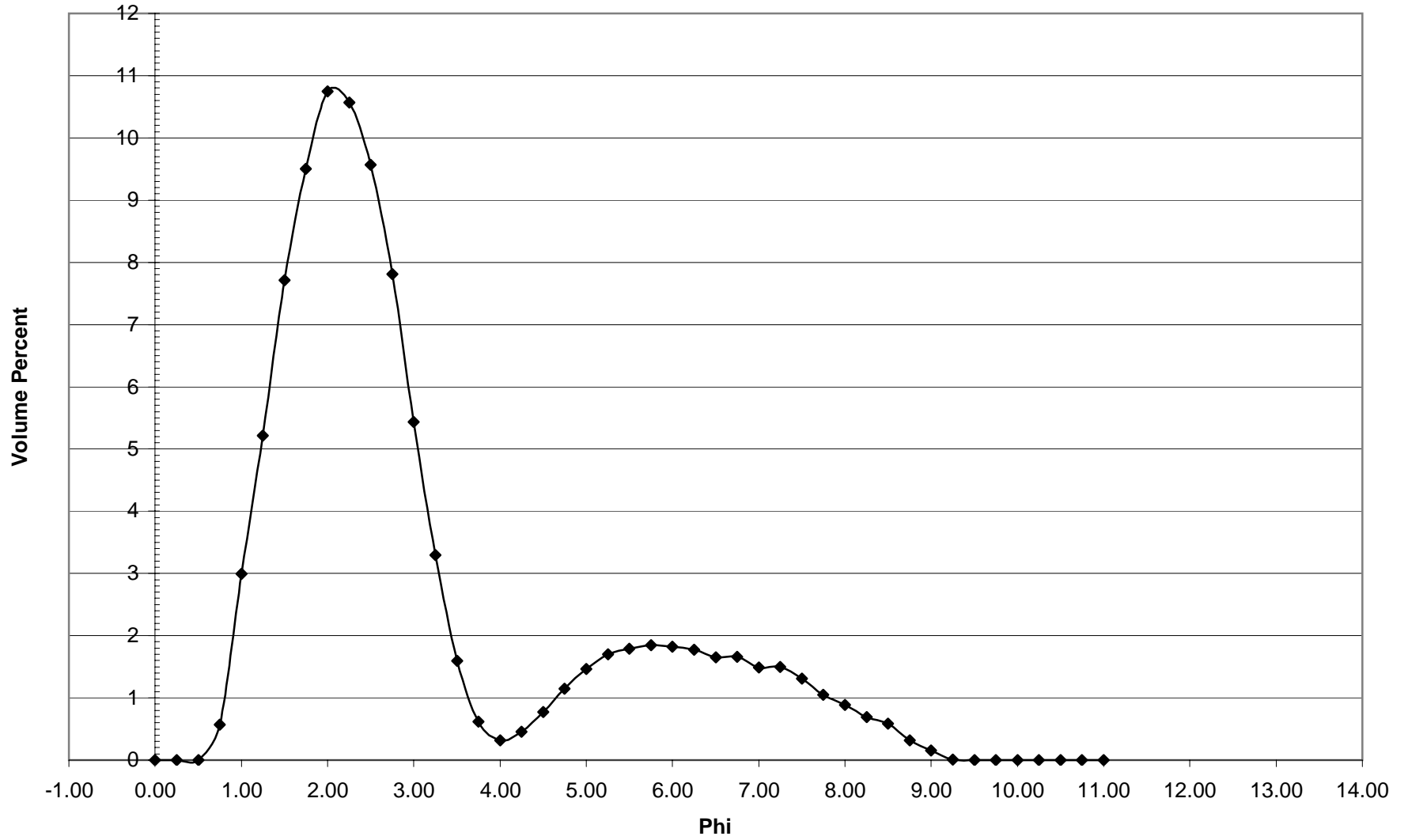
NB-08 Histogram
