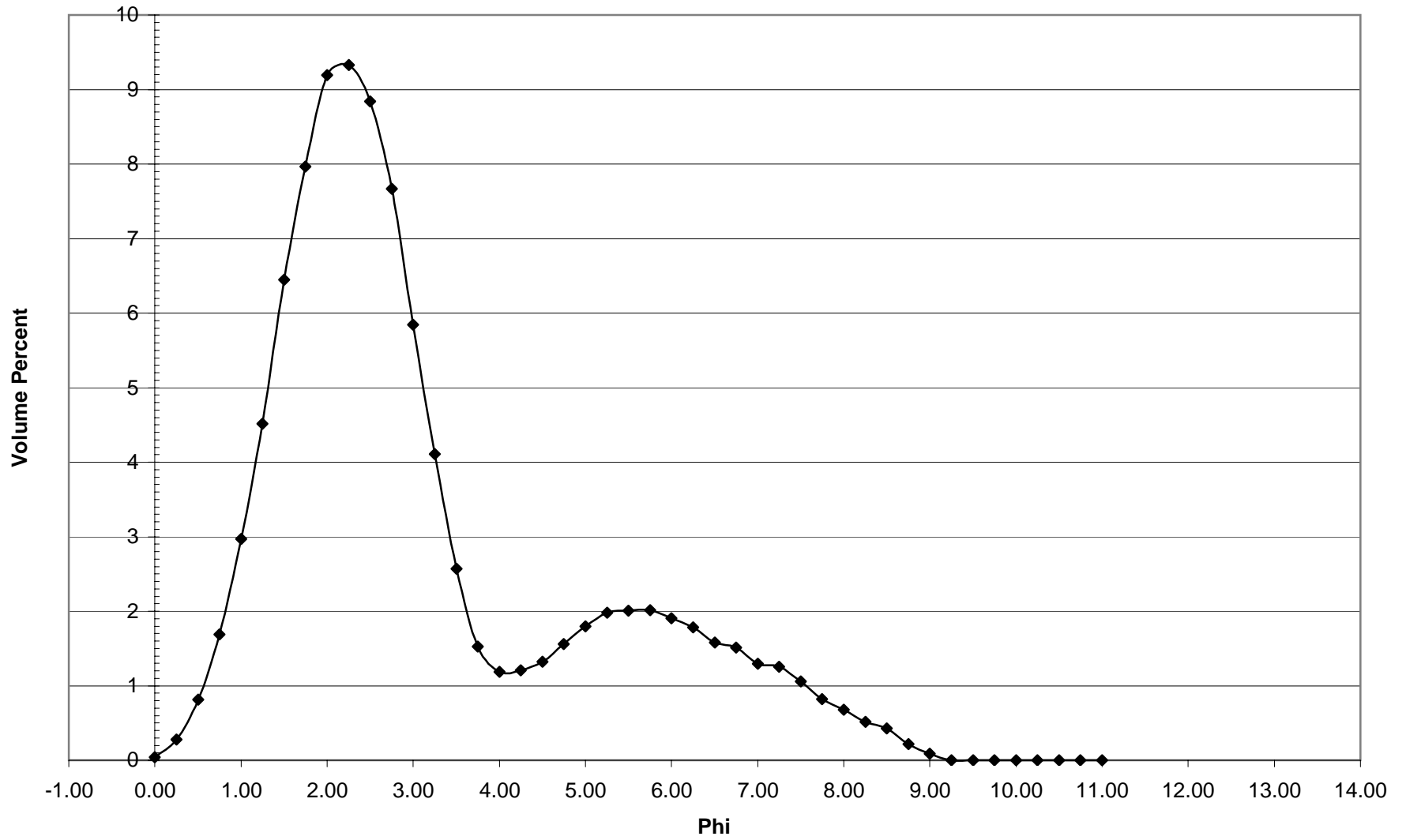
HC-37 Histogram
