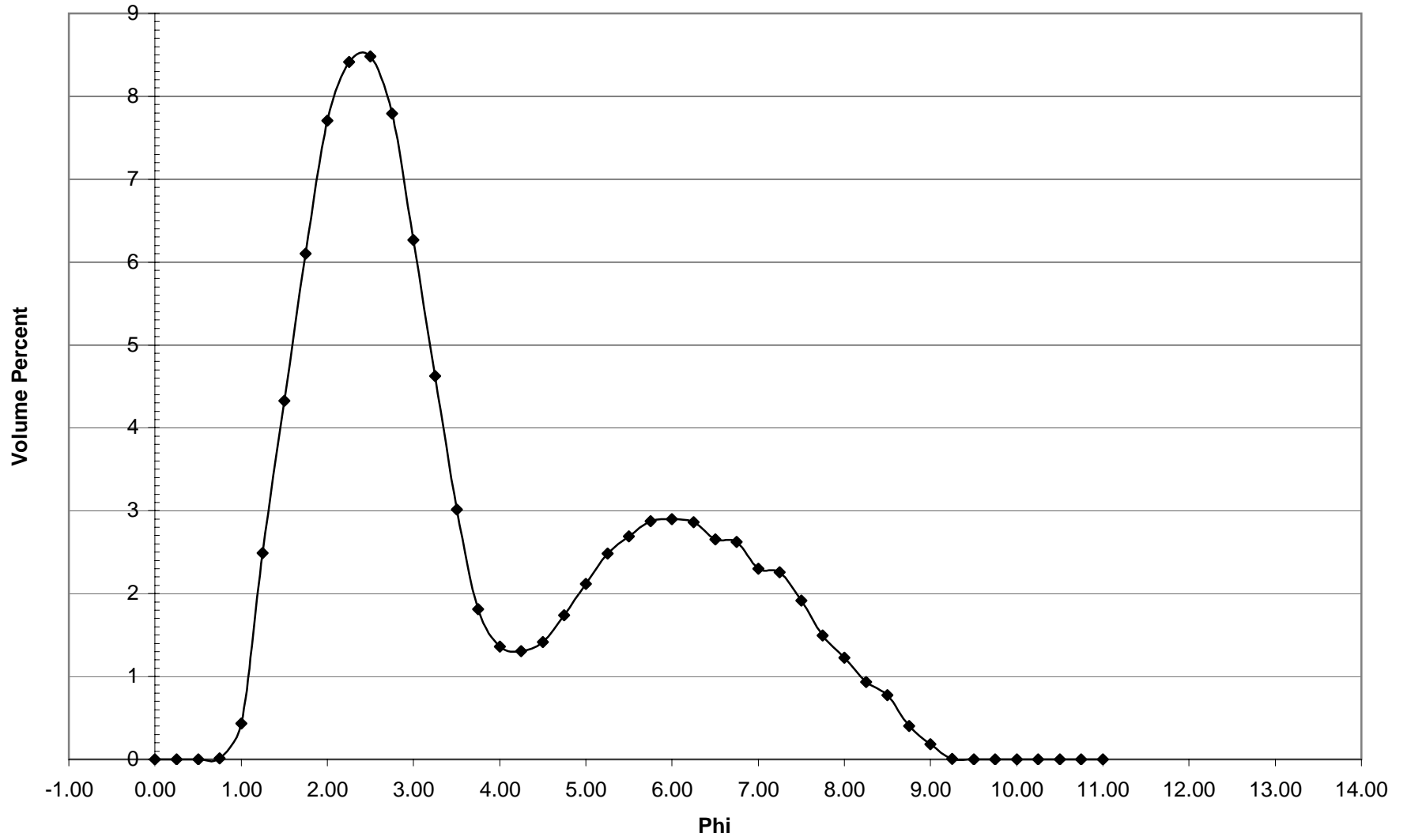
NB-12 Histogram
