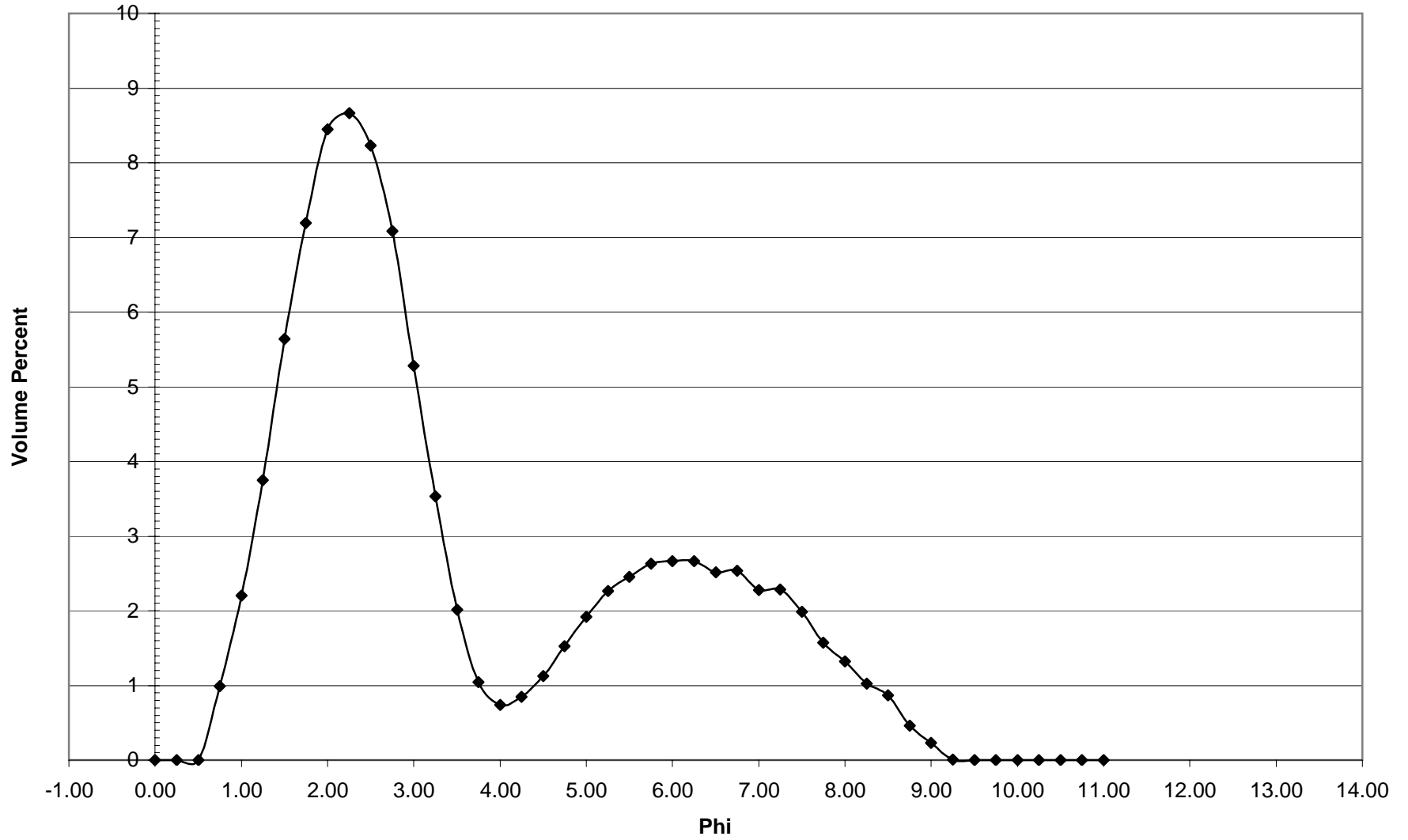
NB-06 Histogram
