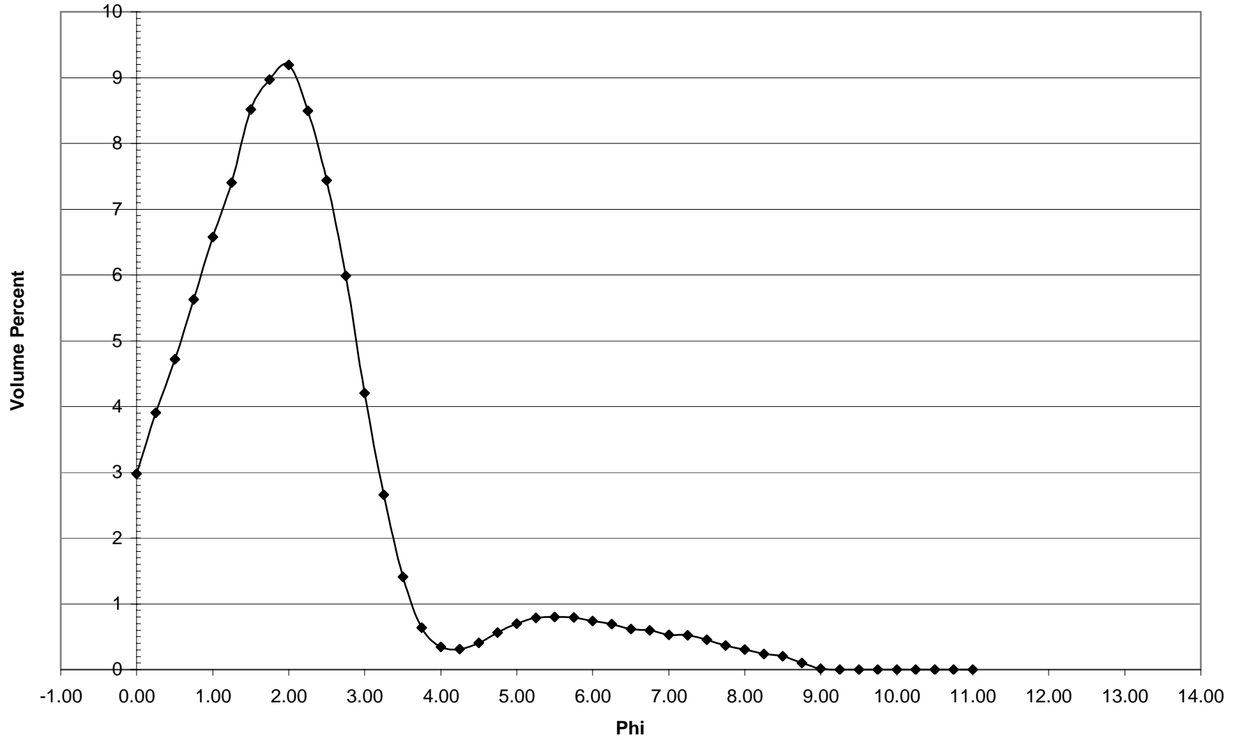
NB-35 Histogram
