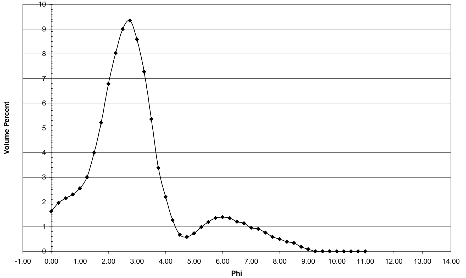
NB-46 Histogram
