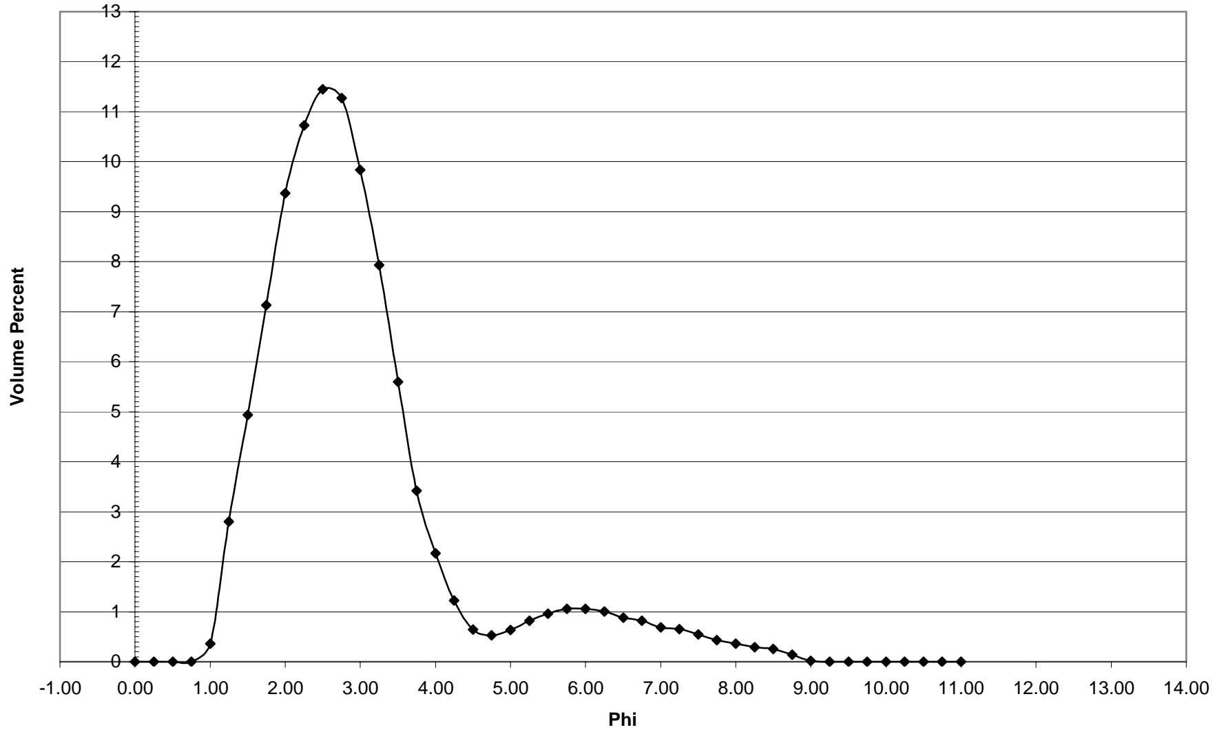
NB-40 Histogram
