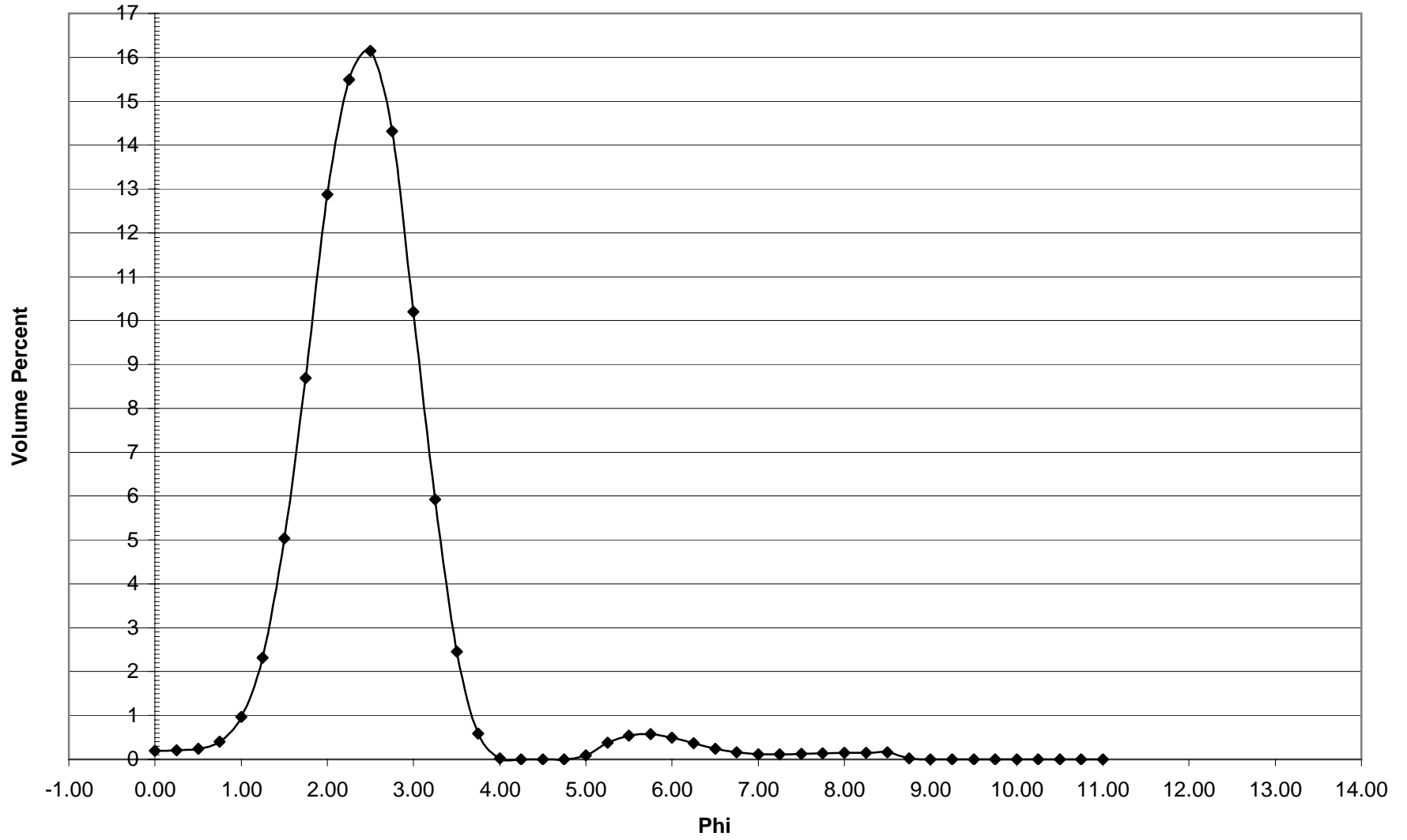
NB-50 Histogram
