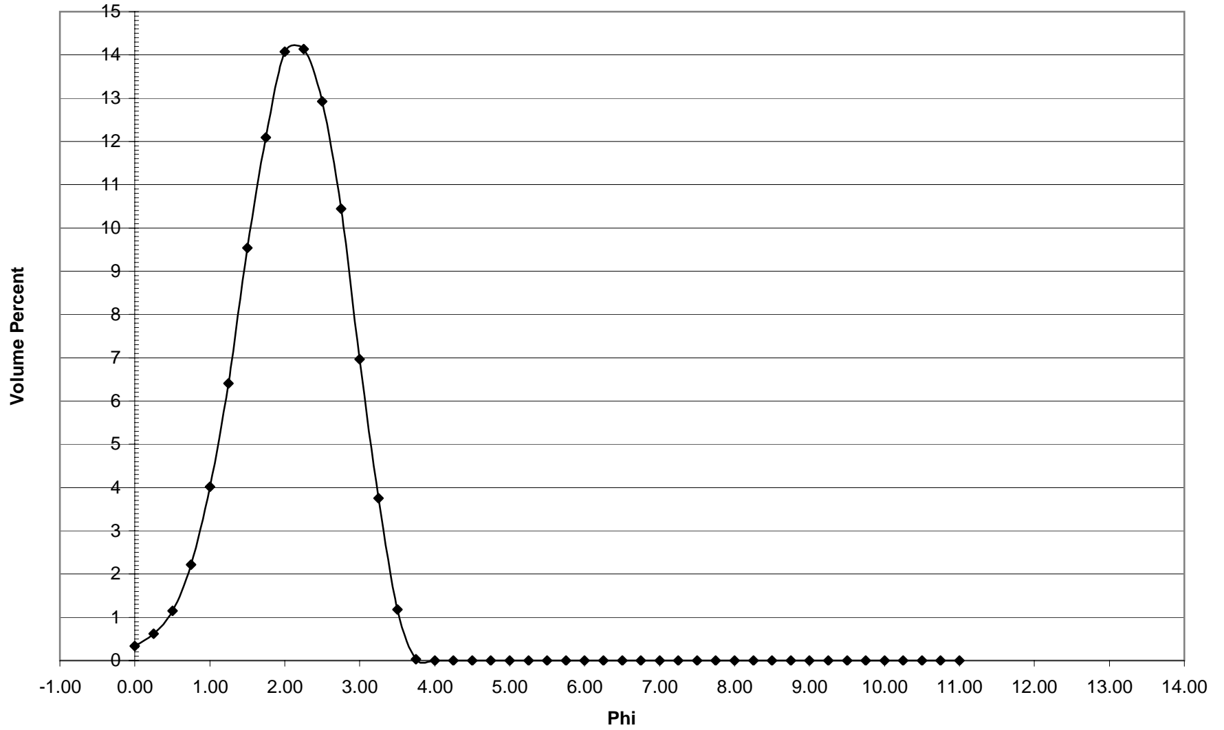
DB-52 Histogram
