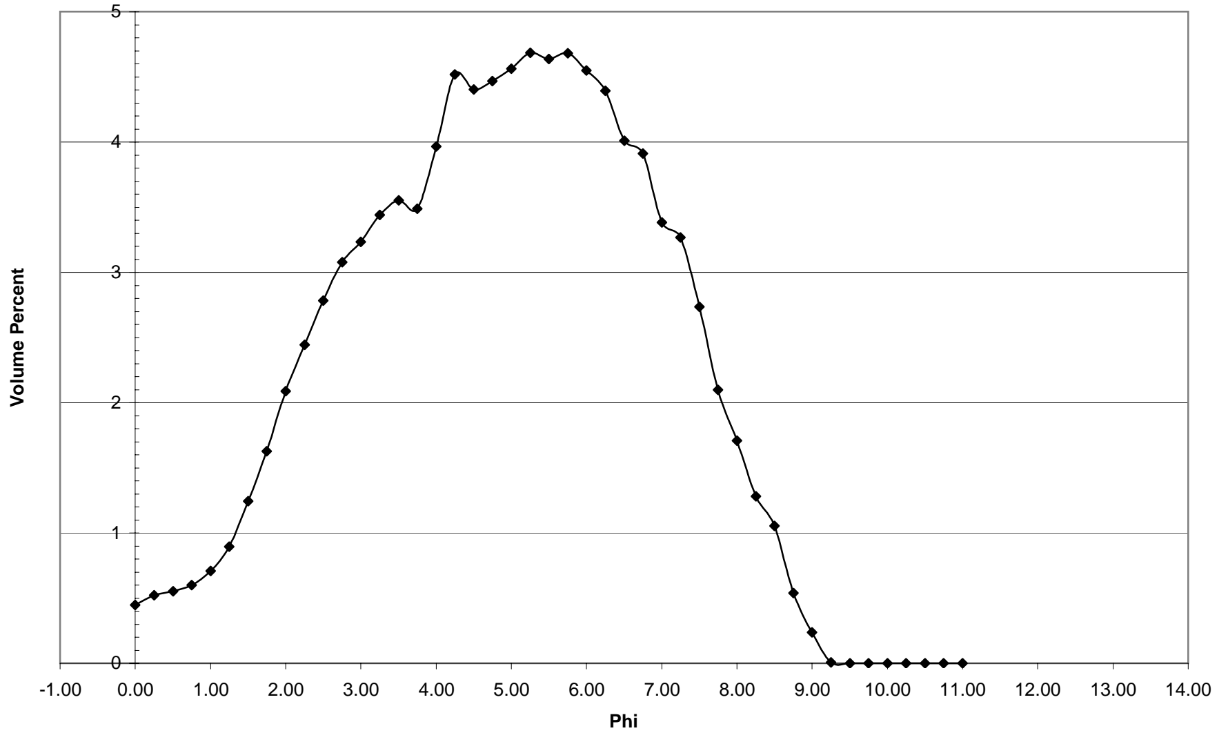
NB-25 Histogram
