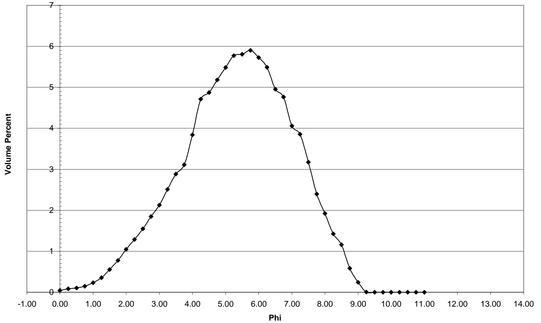
NB-11 Histogram
