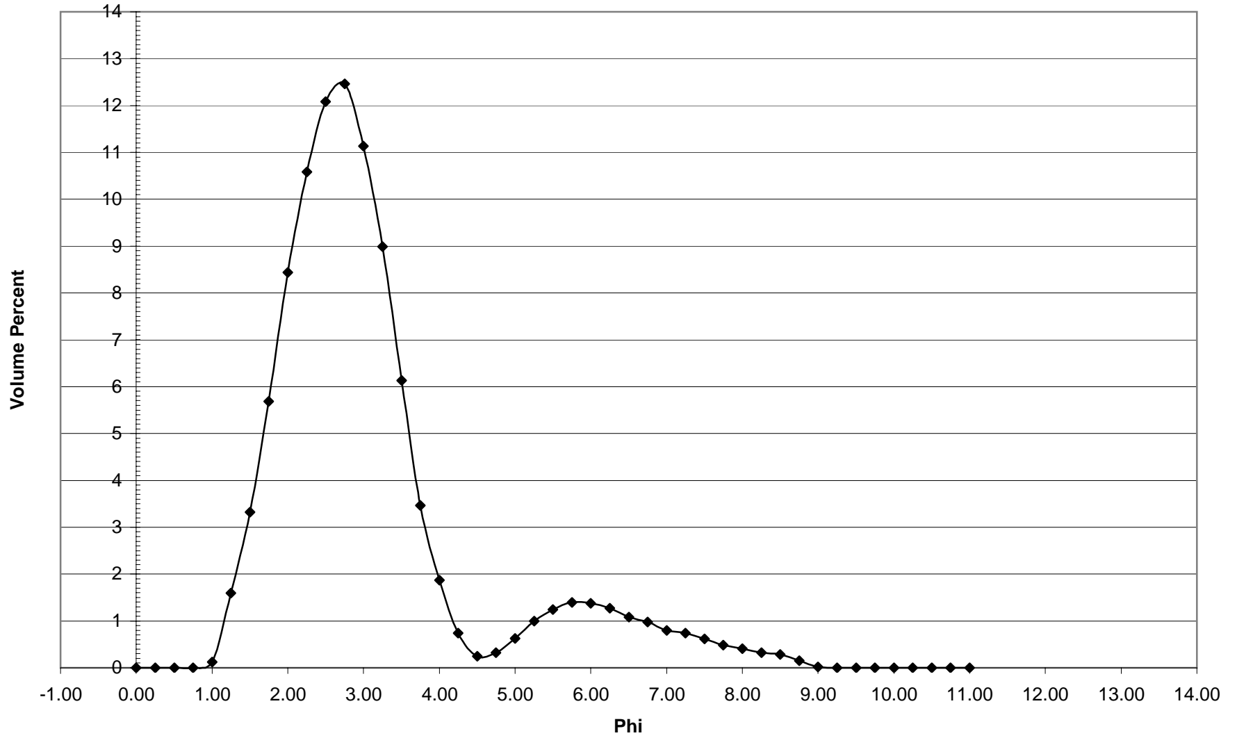
NB-49 Histogram
