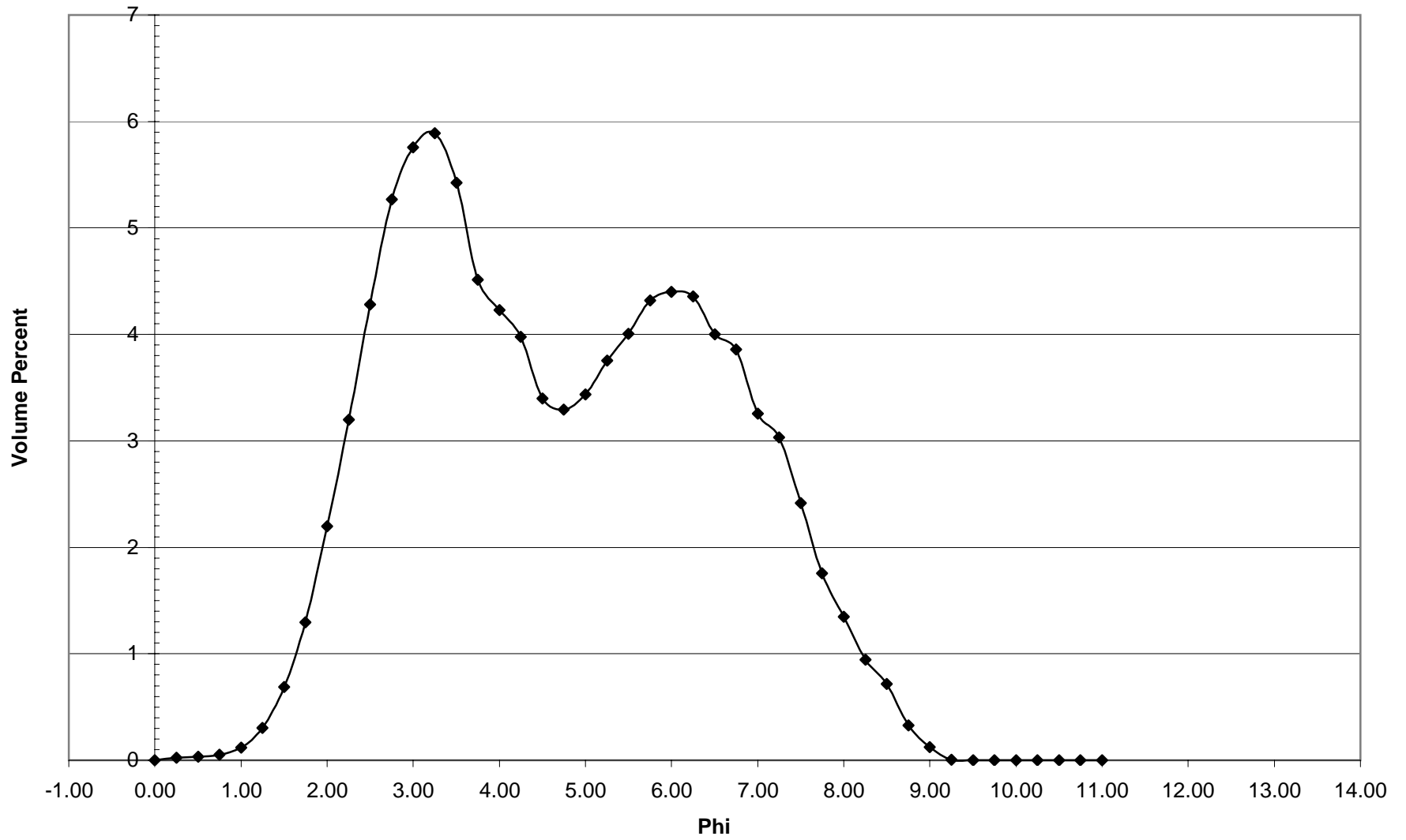
NB-34 Histogram
