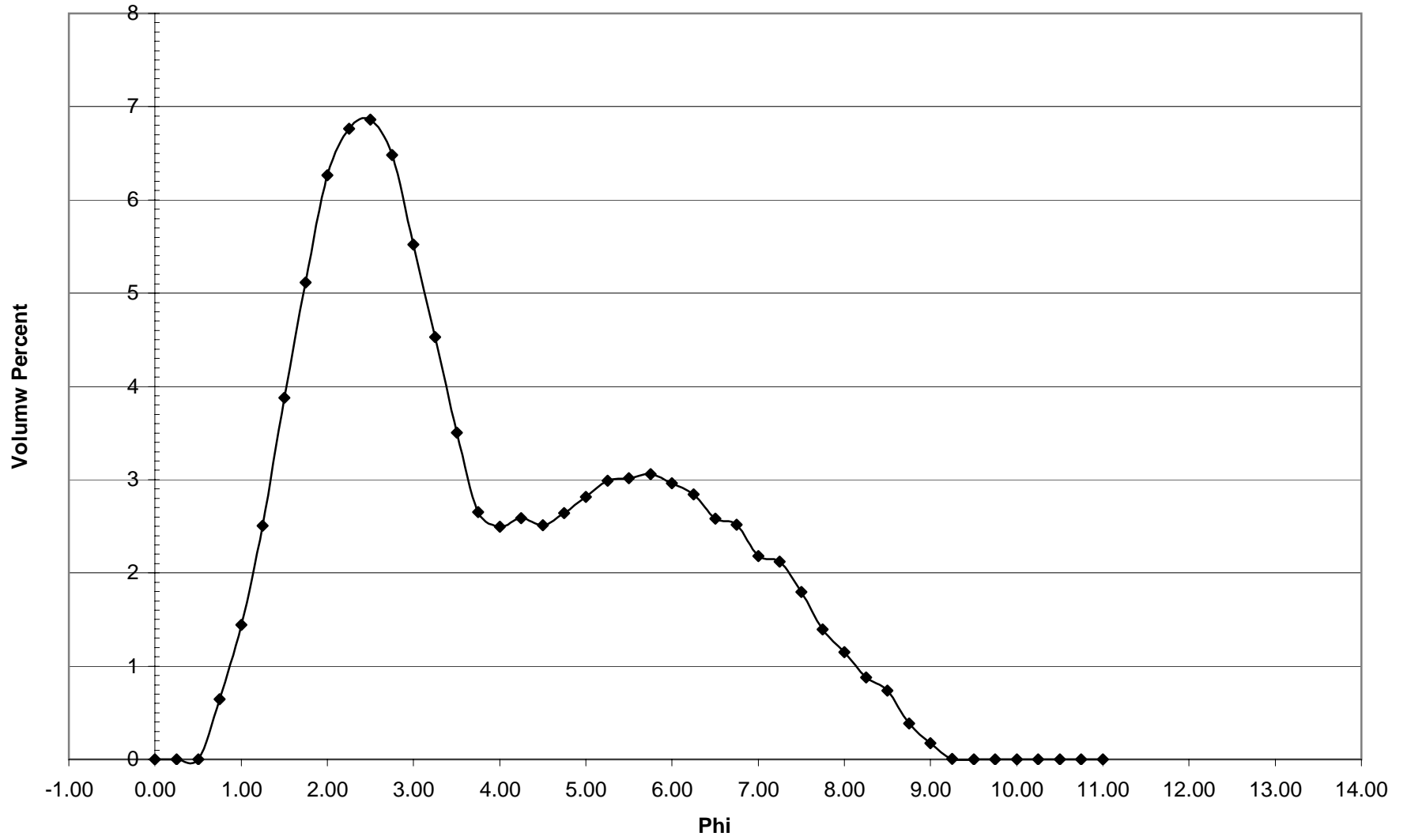
NB-01 Histogram
