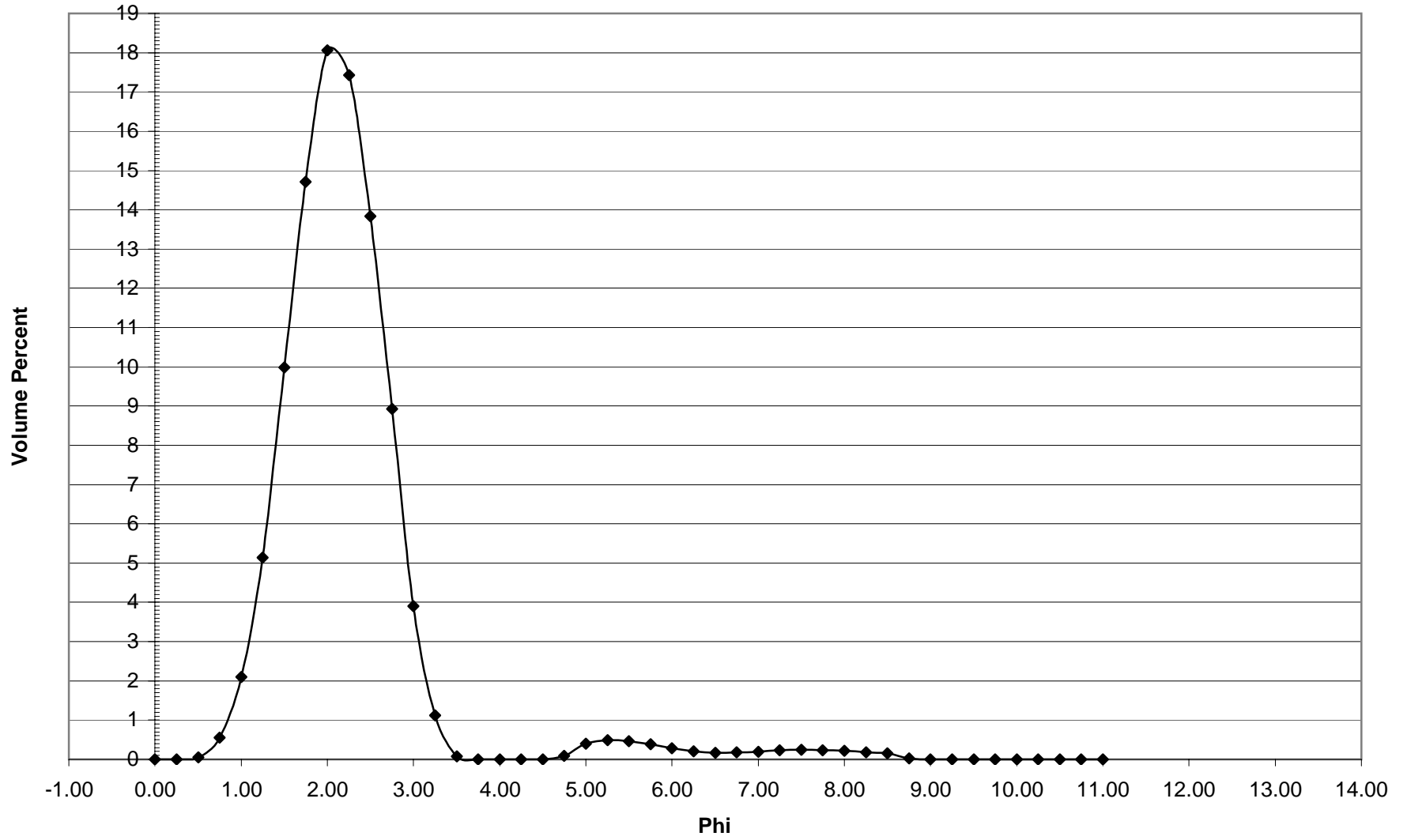
DB-65 Histogram
