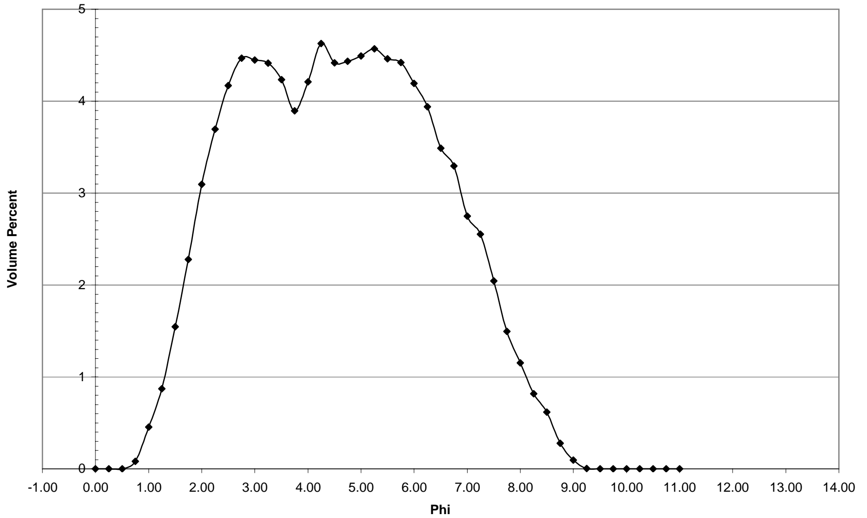
NB-05 Histogram
