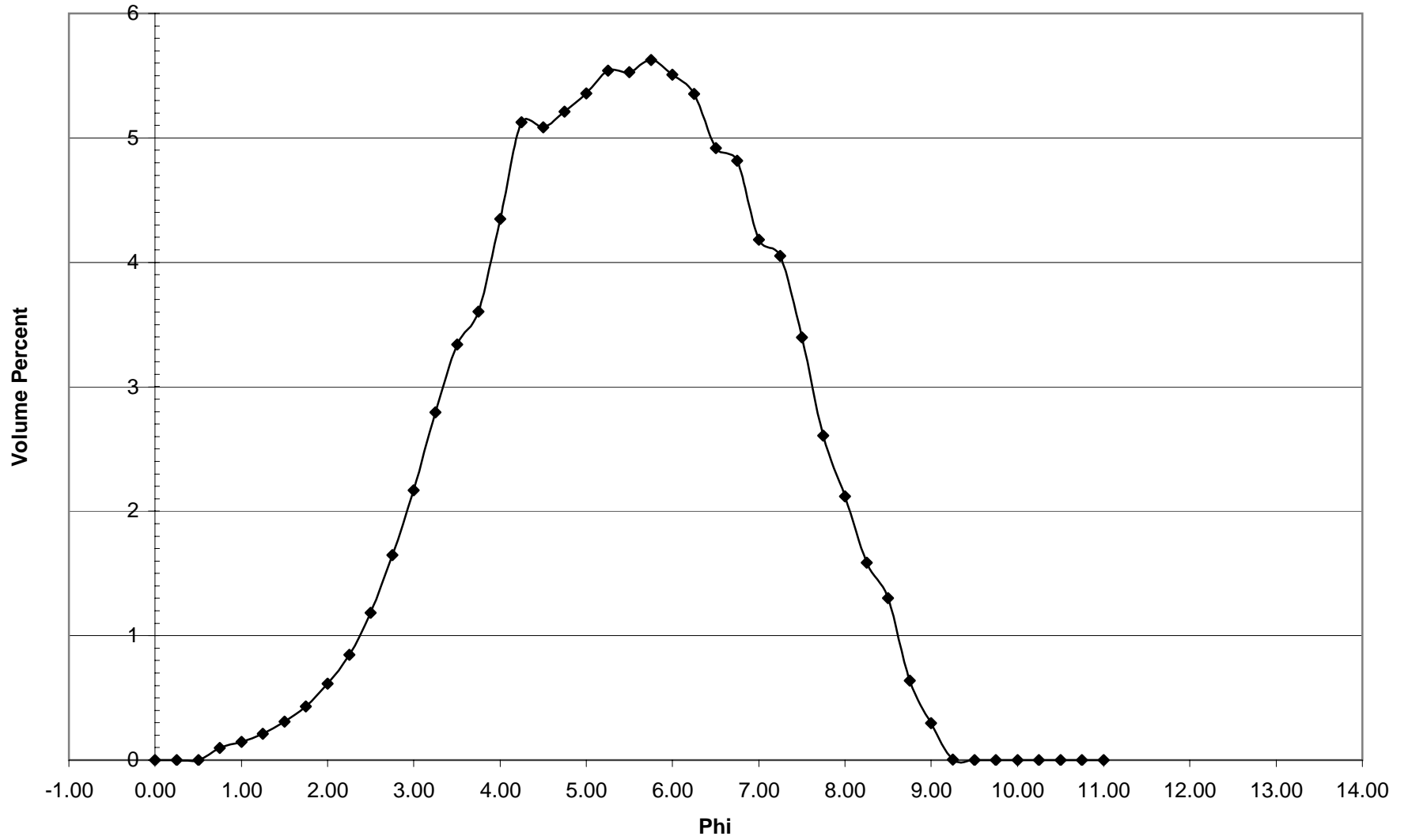
NB-14 Histogram
