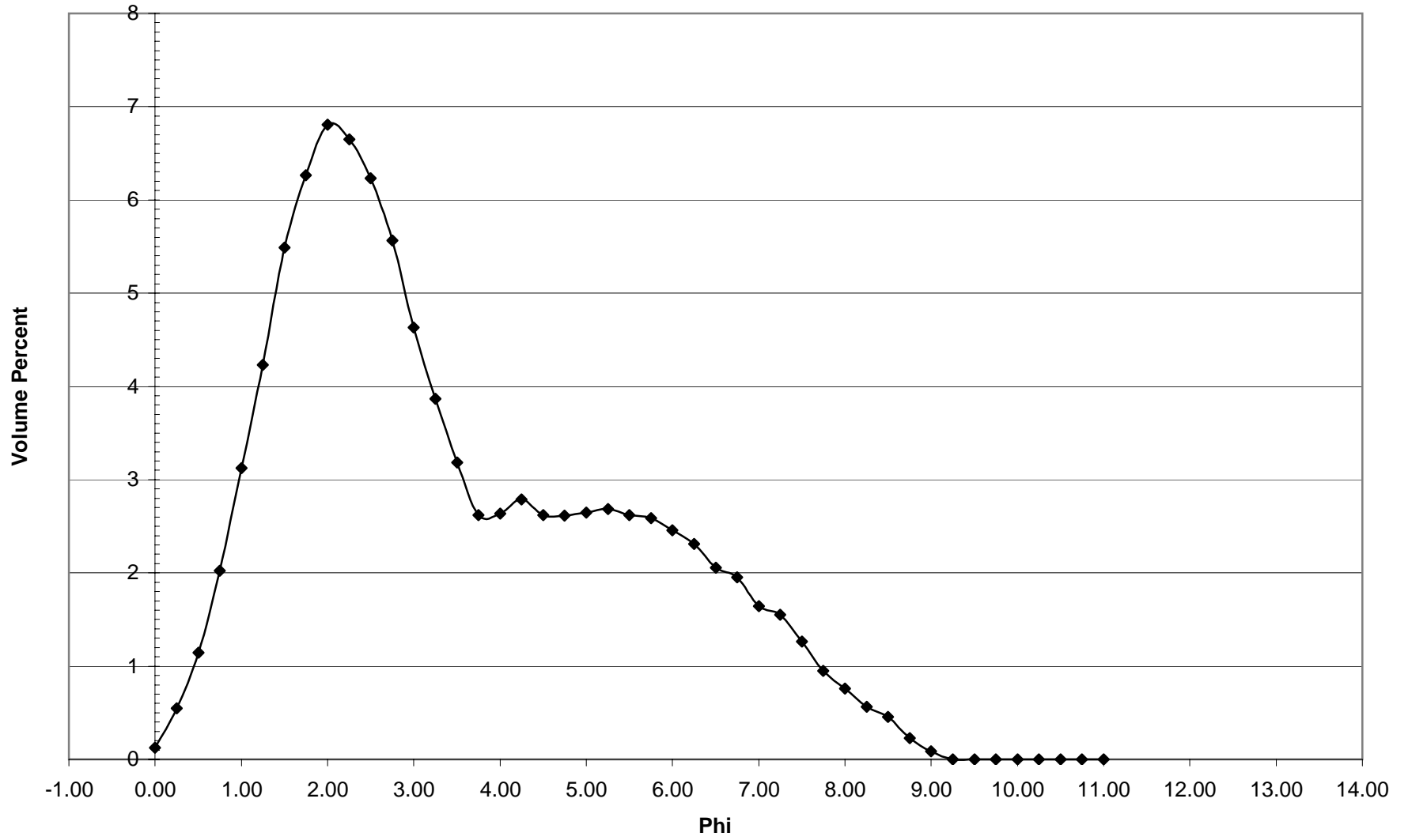
GR-67 Histogram
