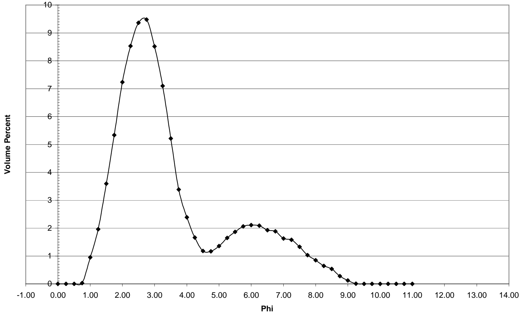
NB-41 Histogram
