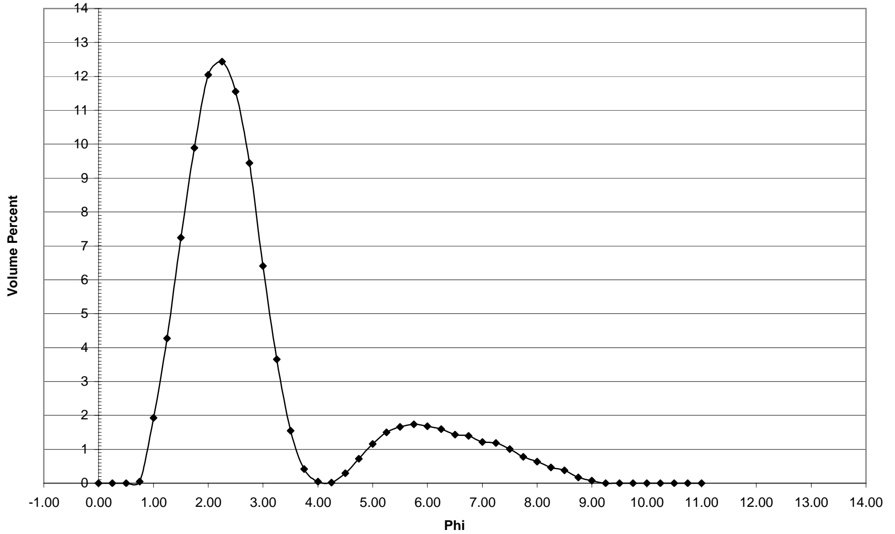
NB-03 Histogram
