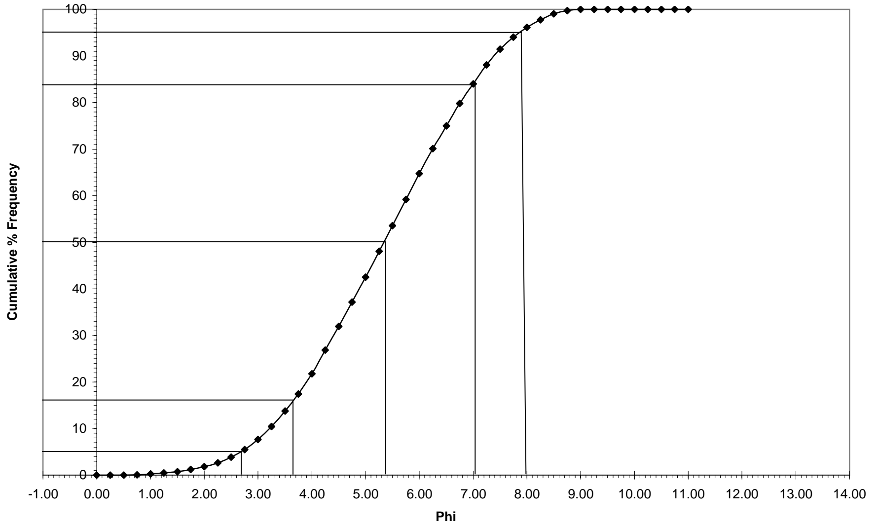
NB-14 Frequency
