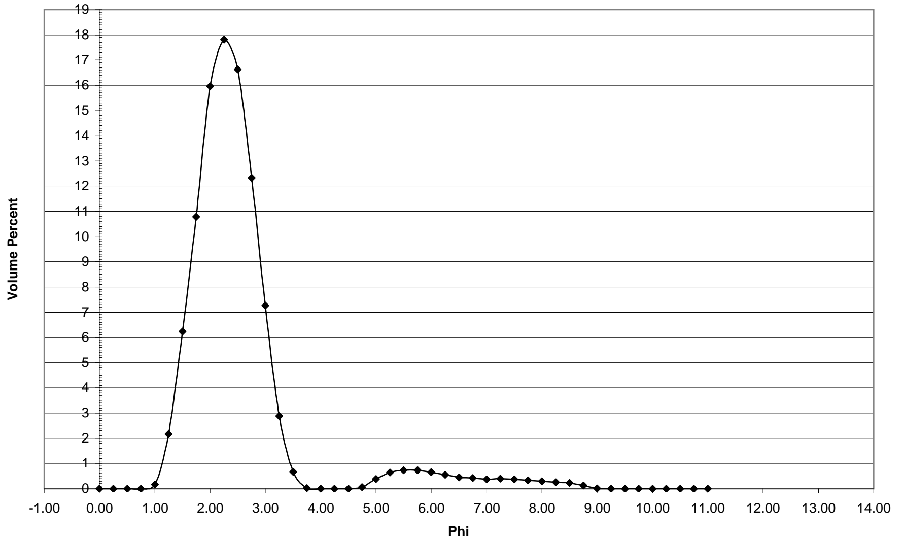
DB-66 Histogram
