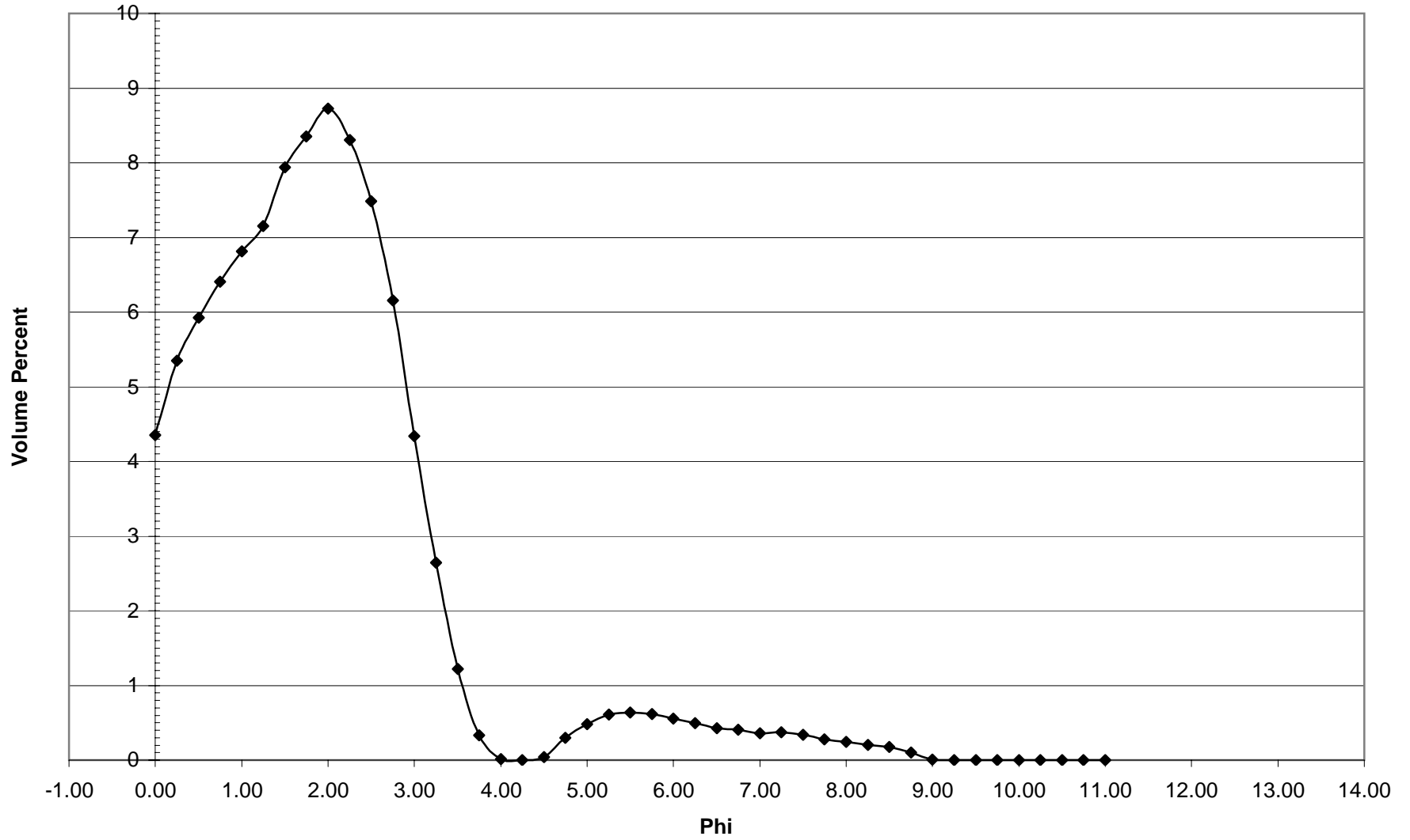
GP-68 Histogram
