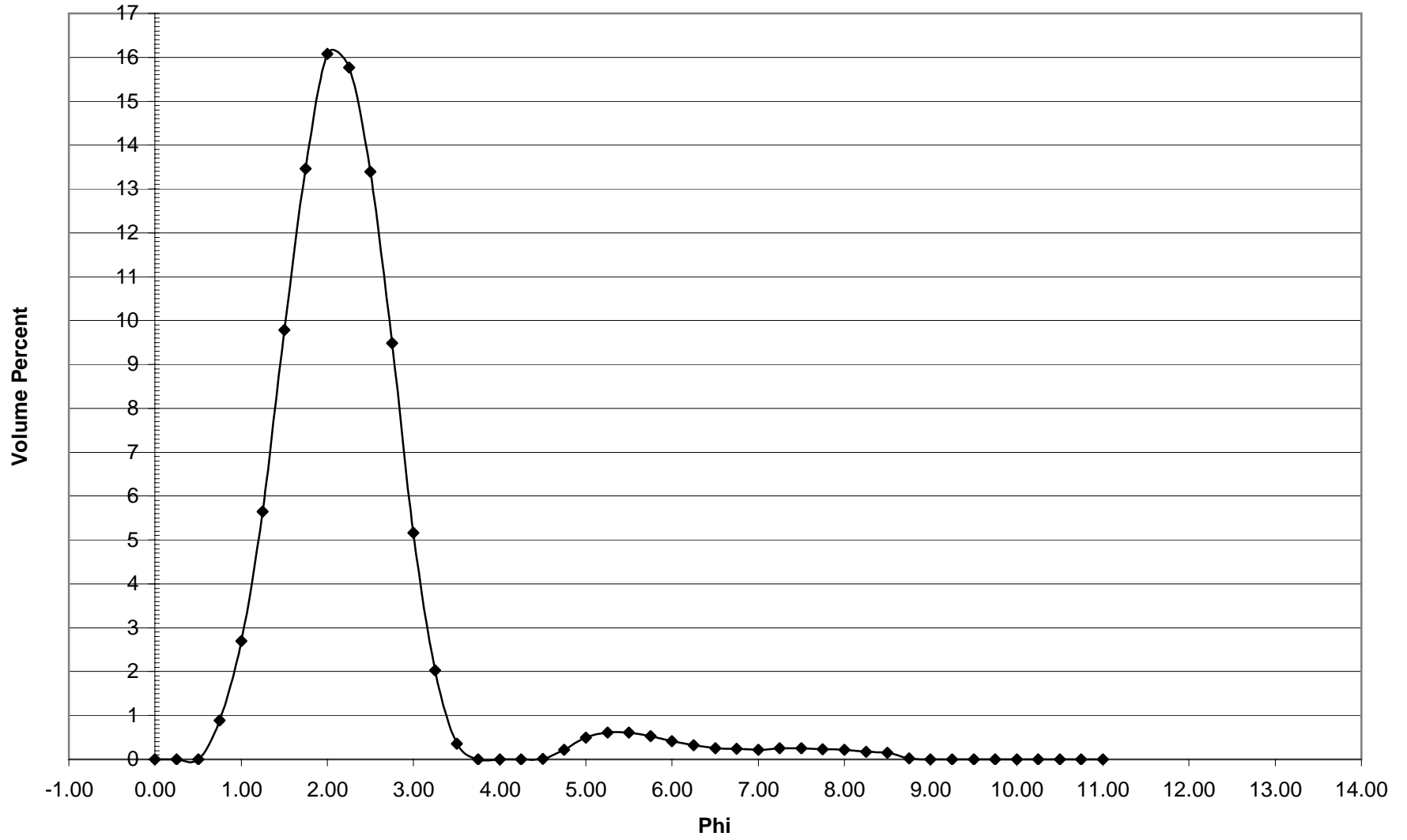
GP-69 Histogram
