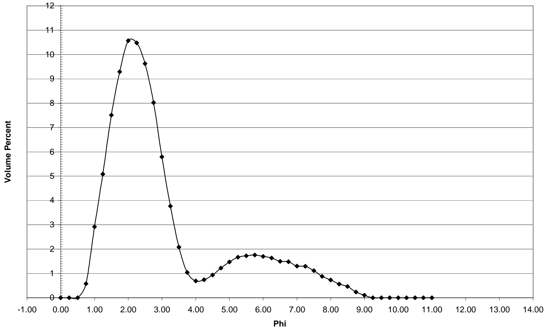
HC-38 Histogram
