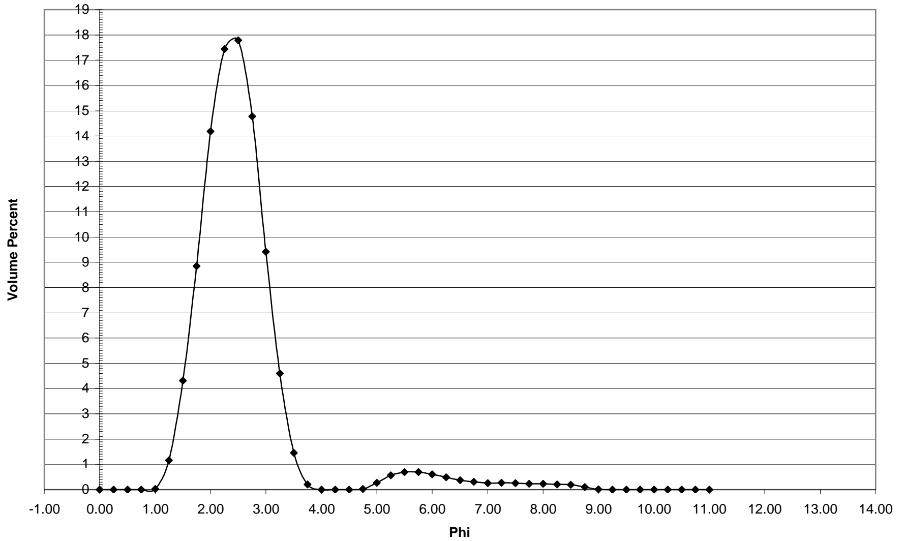
GP-70 Histogram
