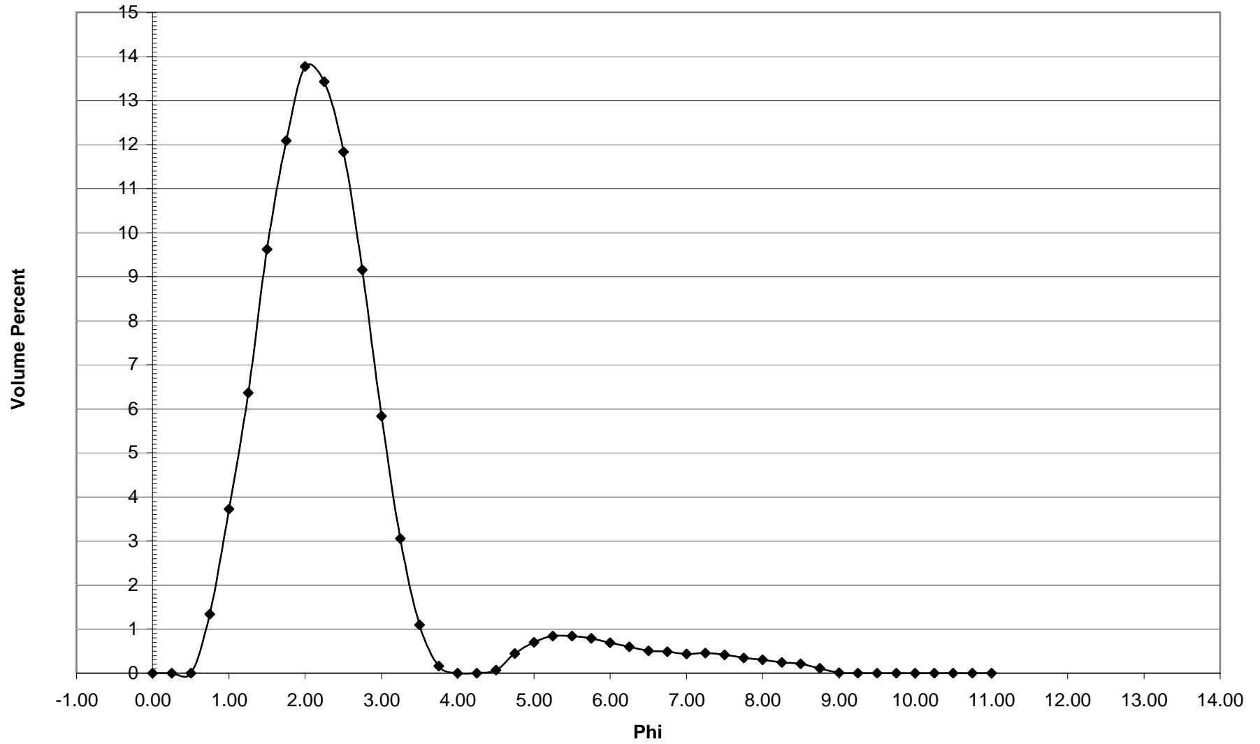
NB-10 Histogram
