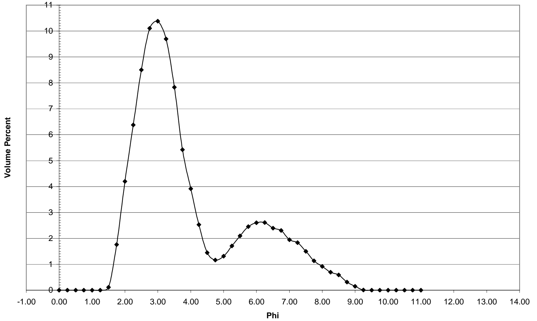
NB-45 Histogram
