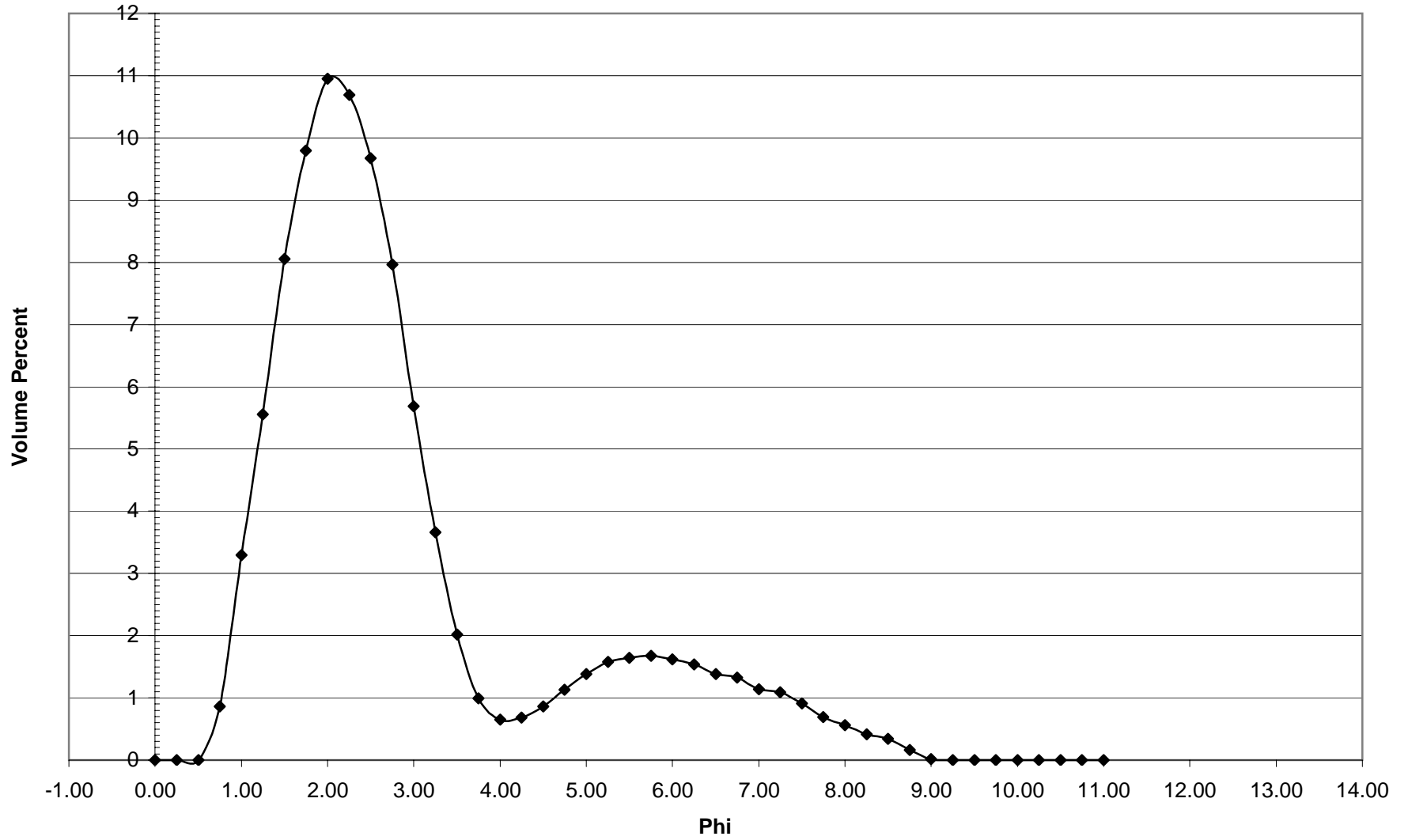
DB-54 Histogram
