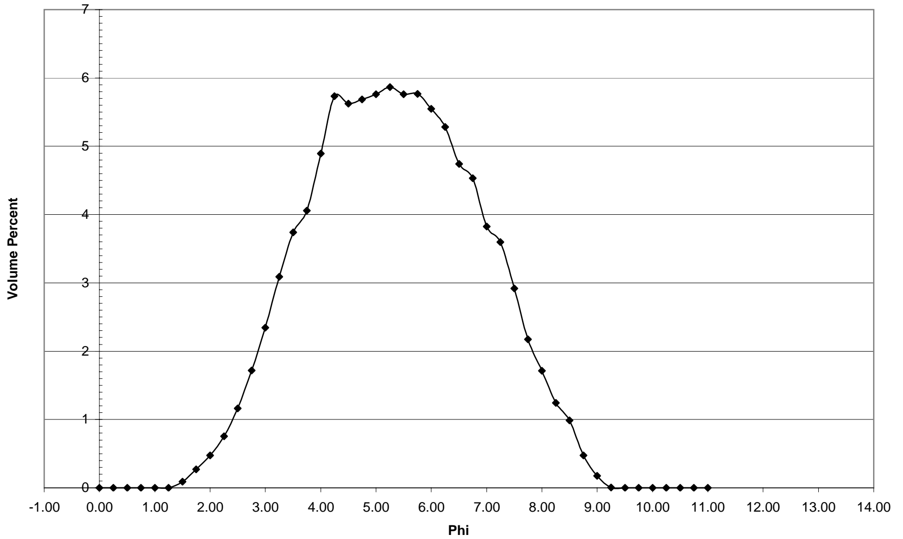
NB-27 Histogram
