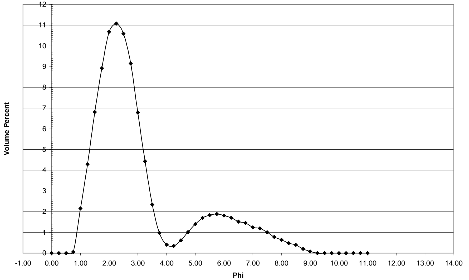
NB-16 Histogram
