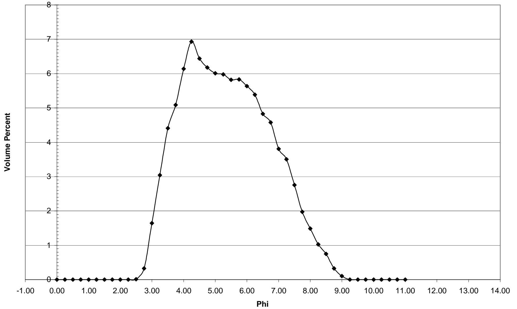
NB-30 Histogram
