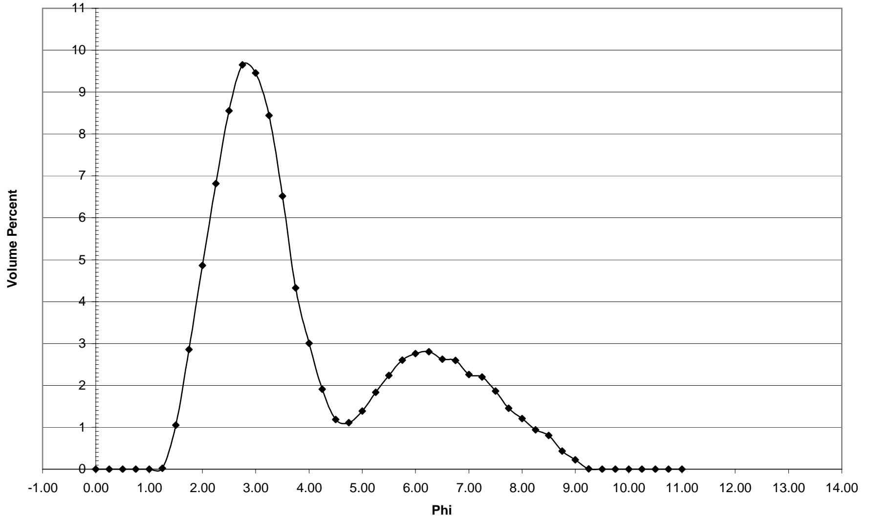
NB-43 Histogram
