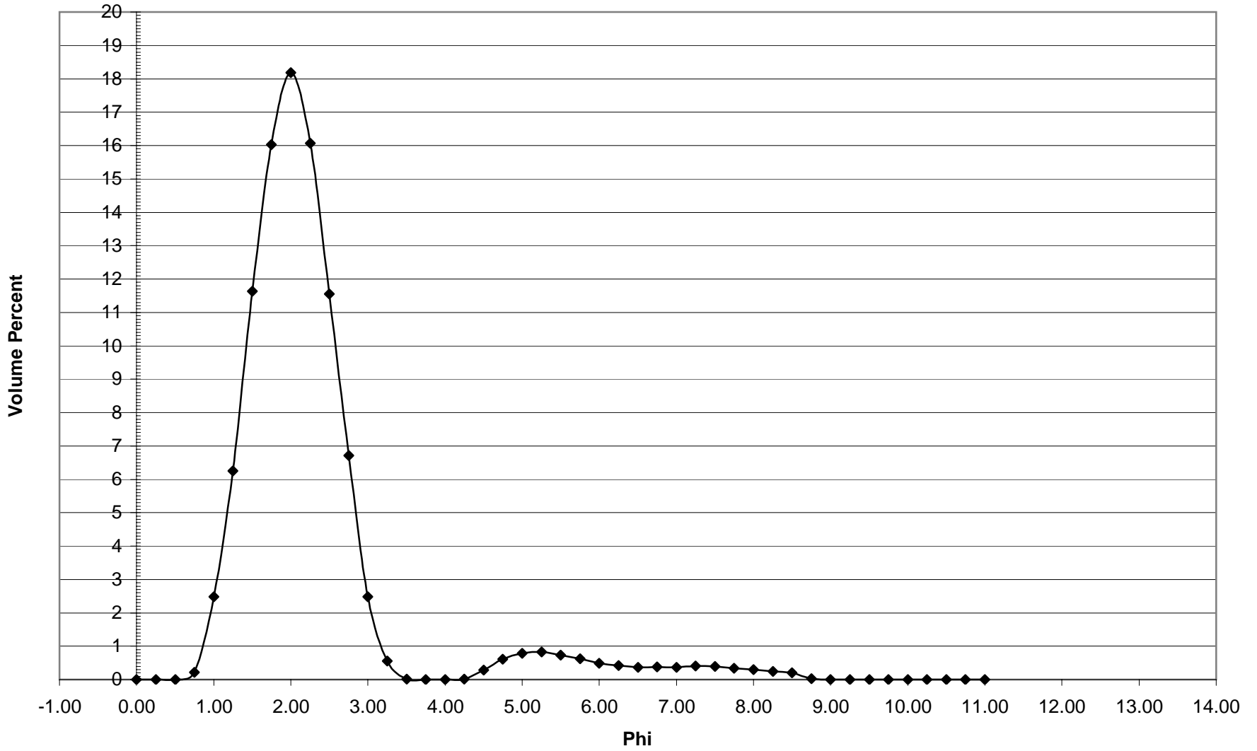
GR-68 Histogram
