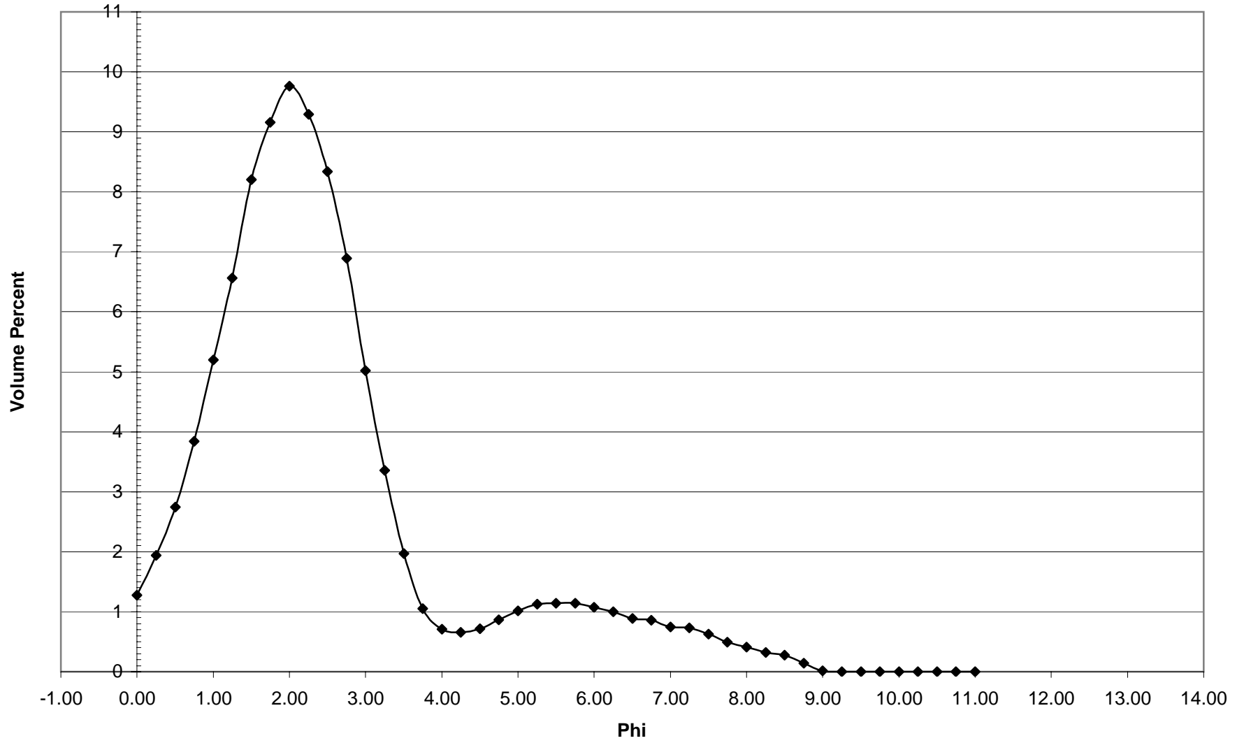
NB-39 Histogram
