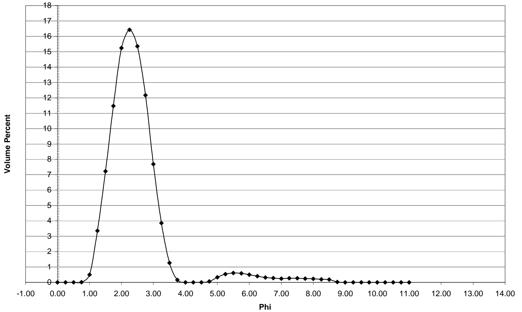
DB-61 Histogram
