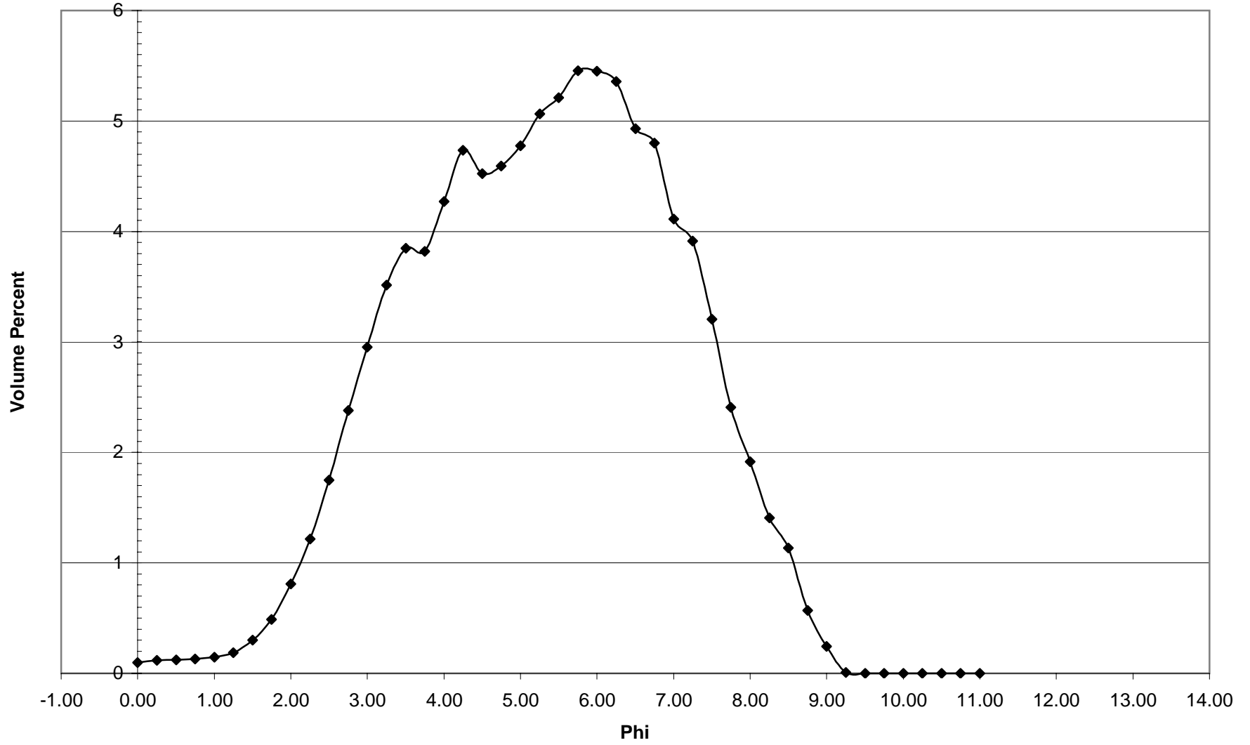
NB-31 Histogram
