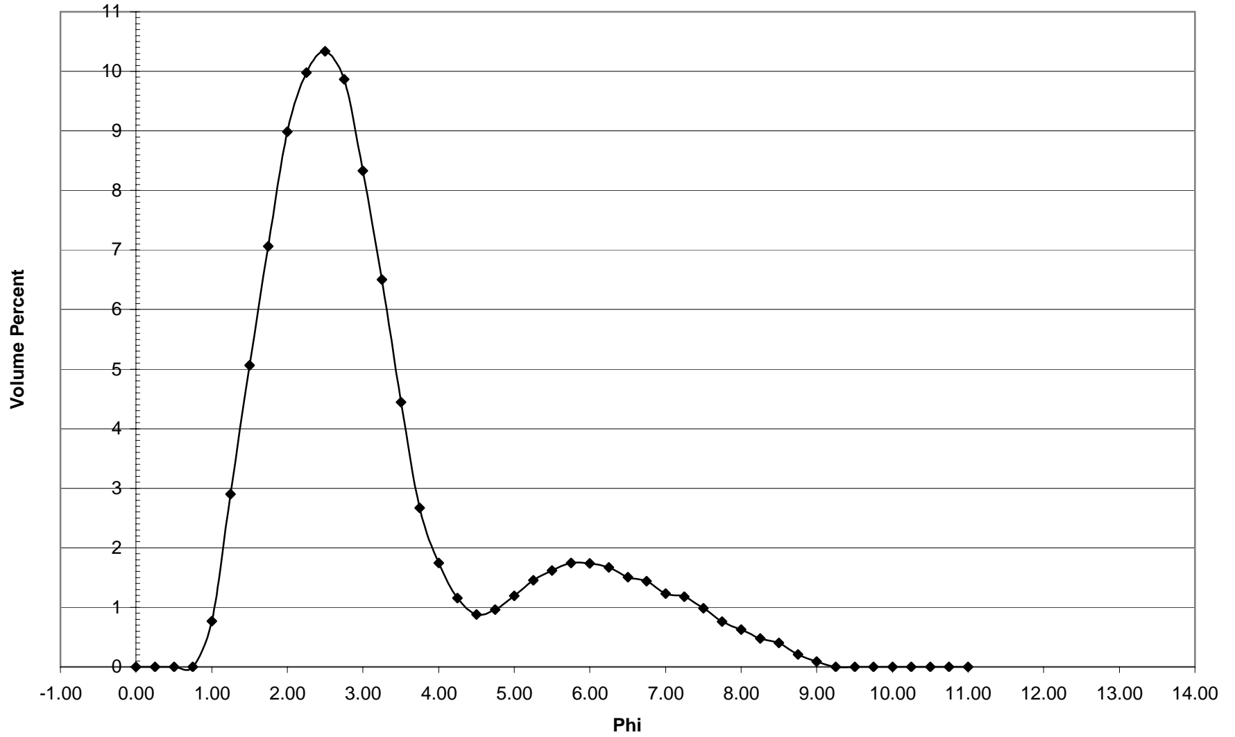
DB-56a Histogram
