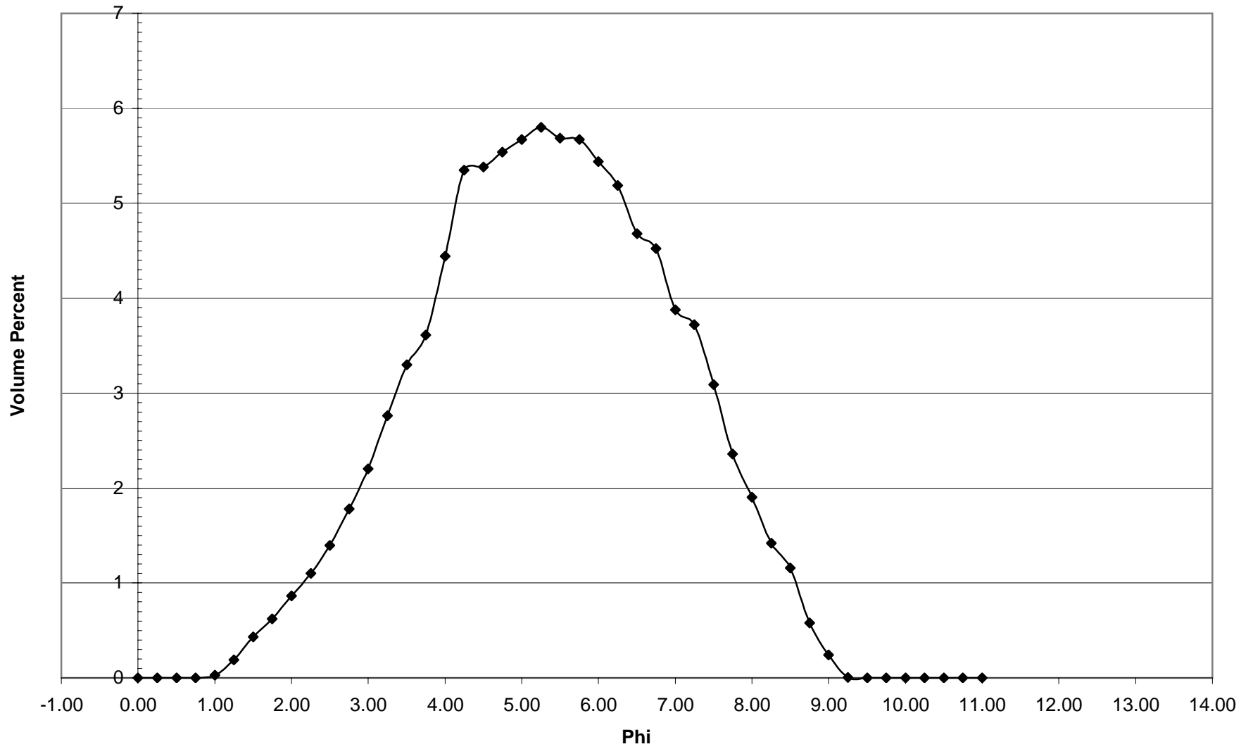
NB-23 Histogram
