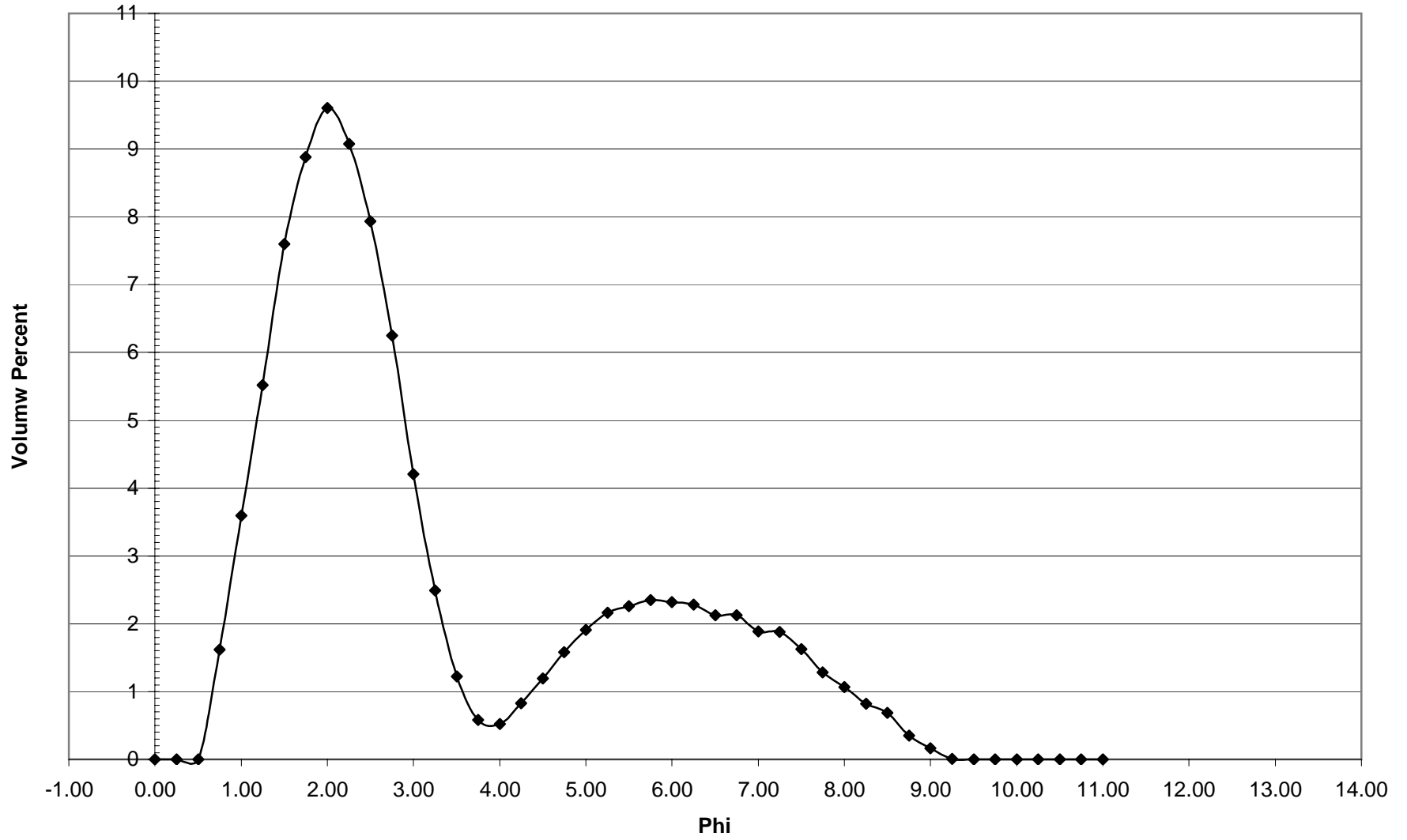
NB-19 Histogram
