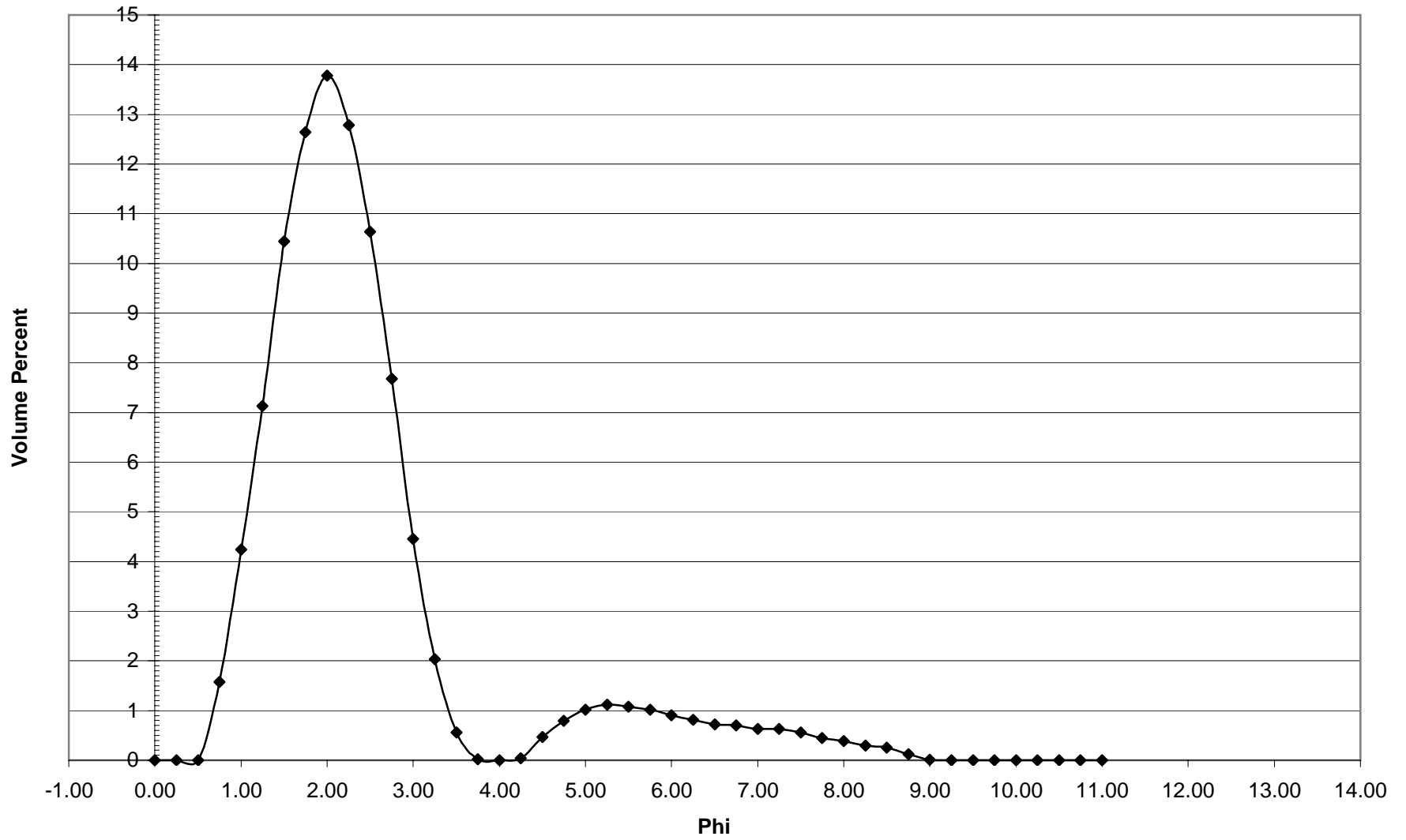
RC-66 Histogram
