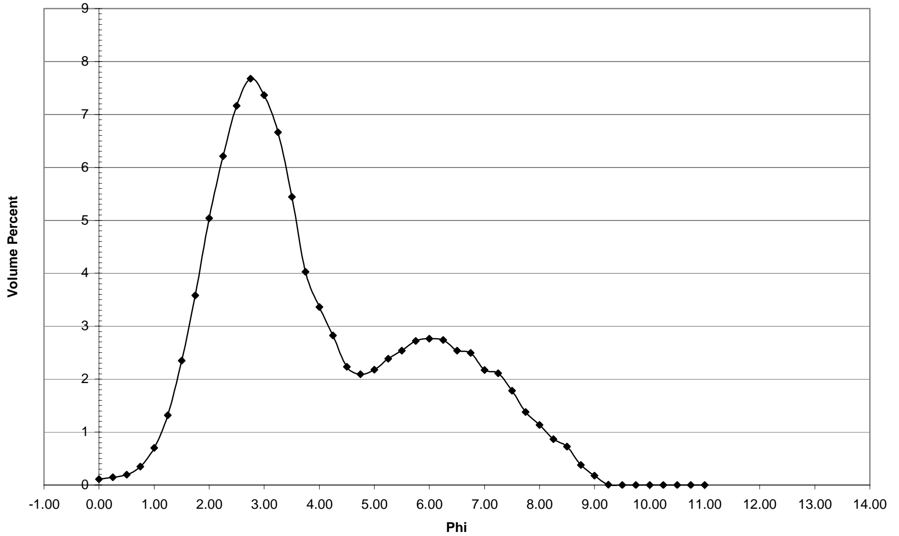
DB-64 Histogram
