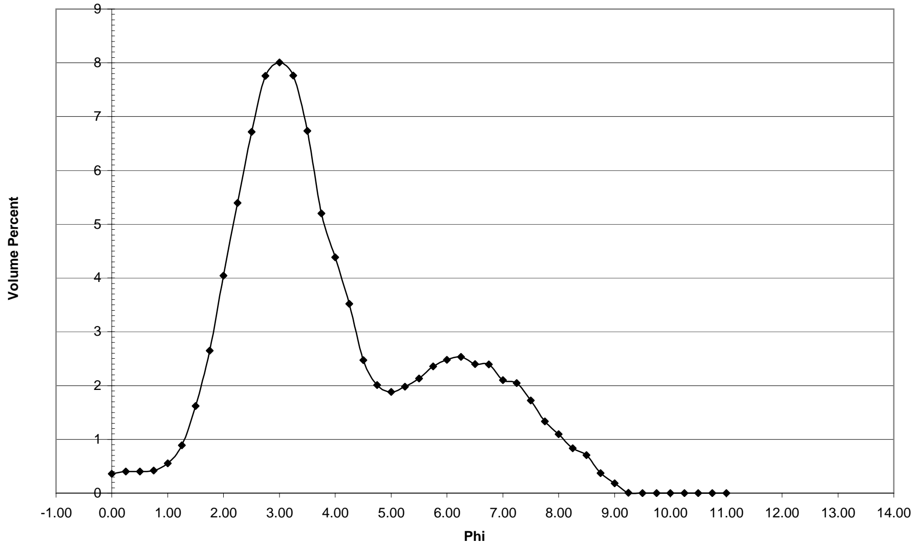
NB-44 Histogram
