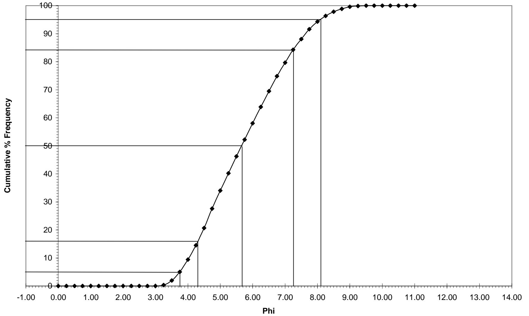
NB-30 % Frequency
