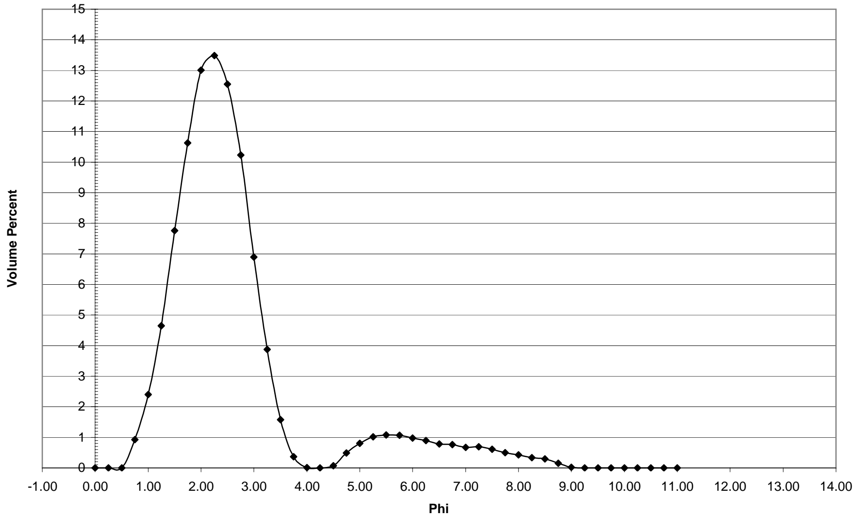
DB-56 Histogram
