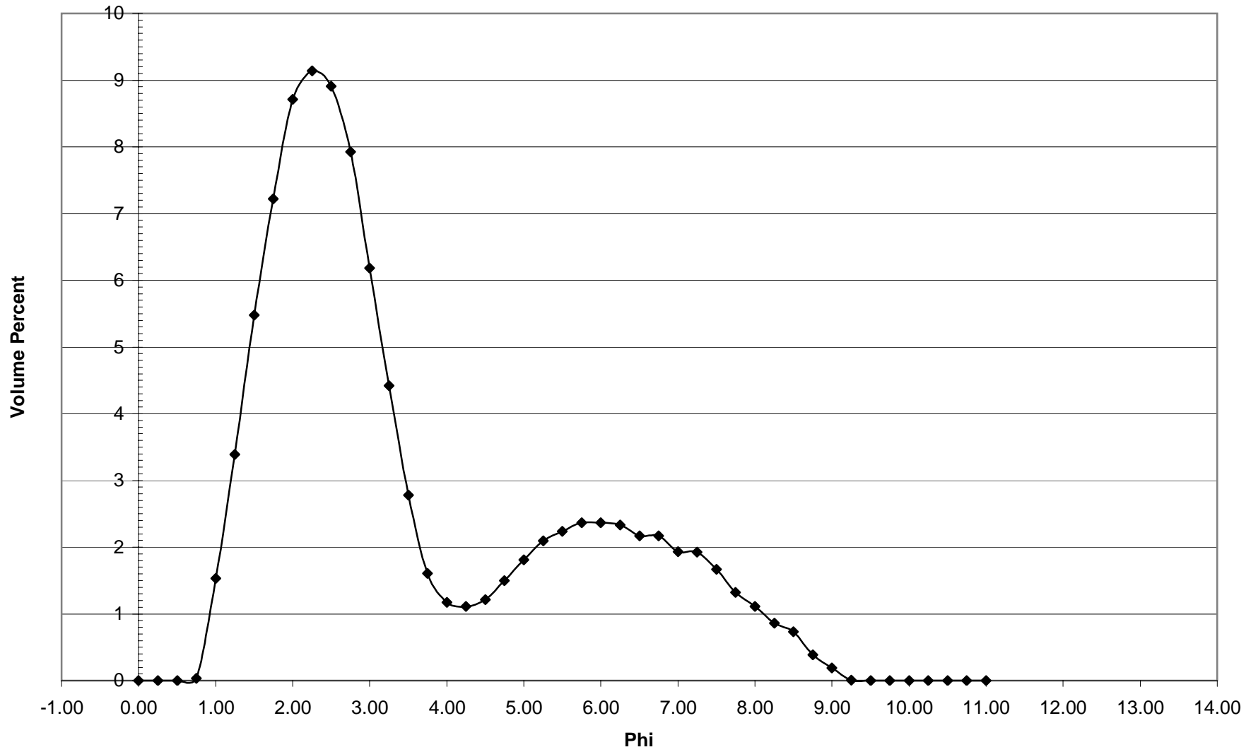
NB-18 Histogram
