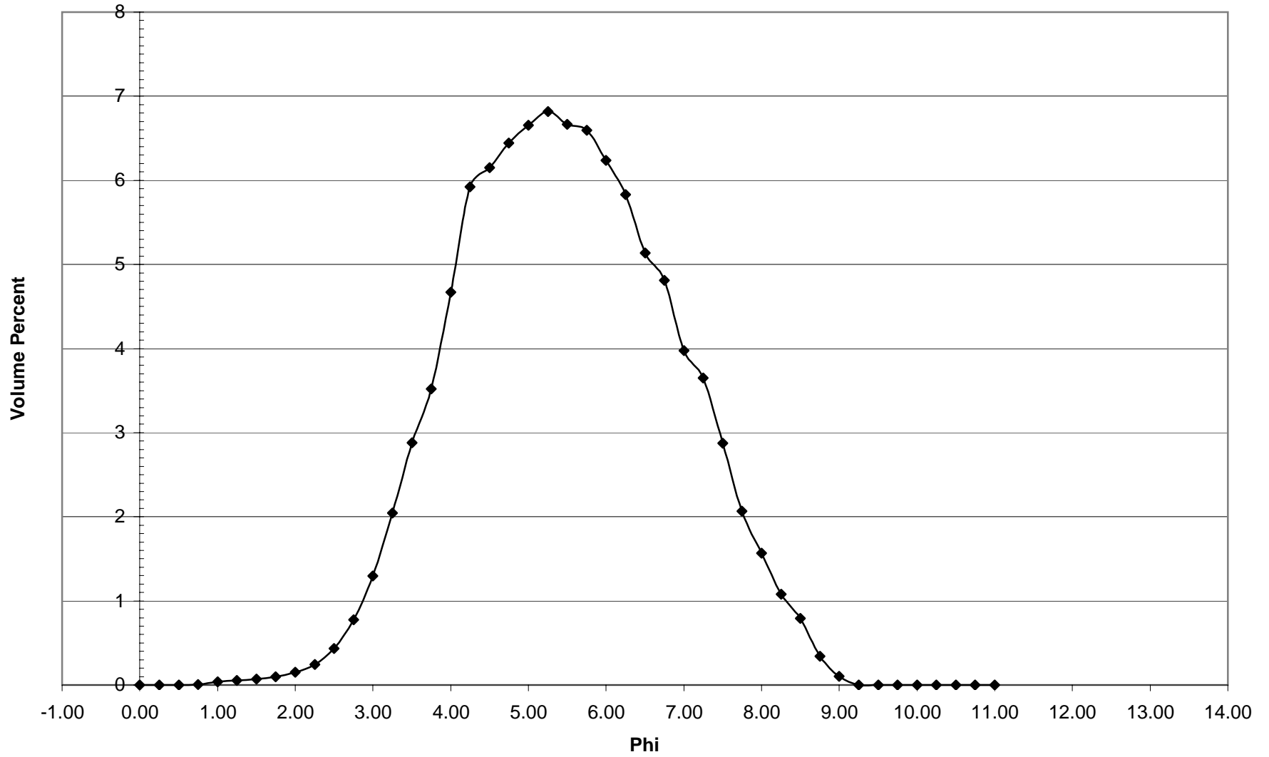
NB-24 Histogram
