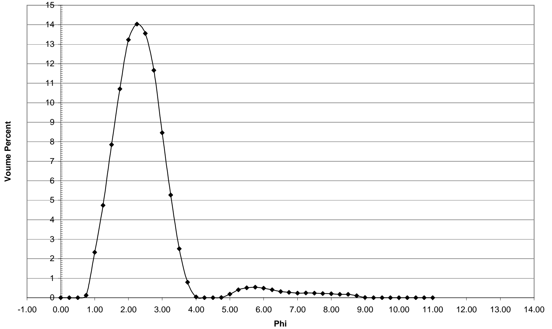
GP-71 Histogram
