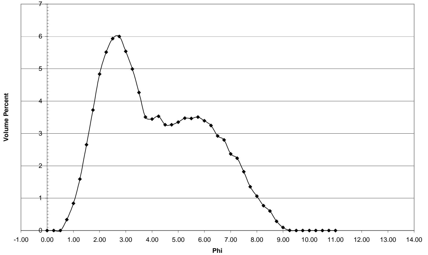
DB-62 Histogram
