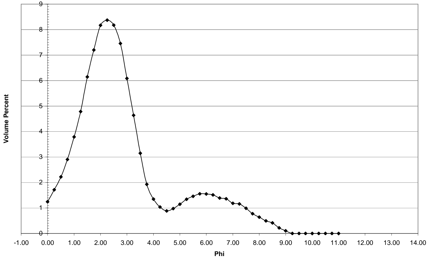
DB-59 Histogram
