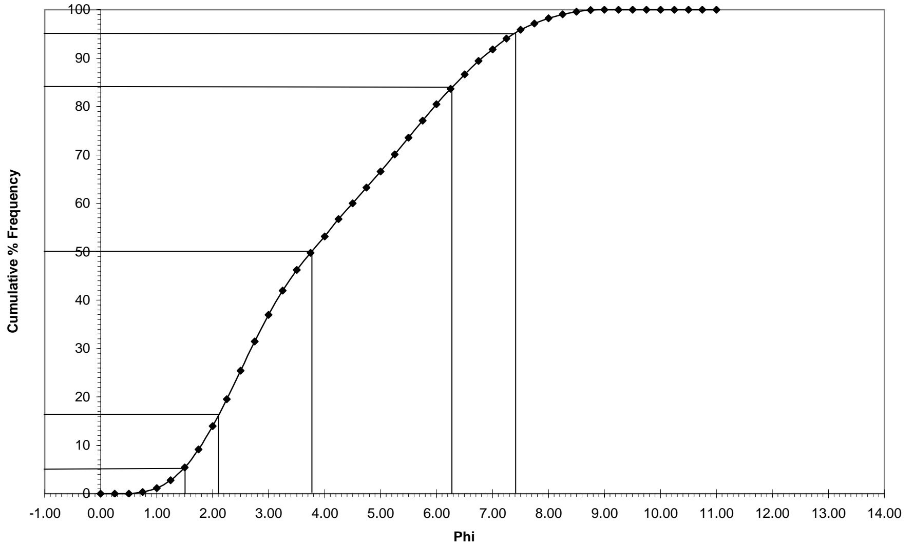
DB-62 % Frequency
