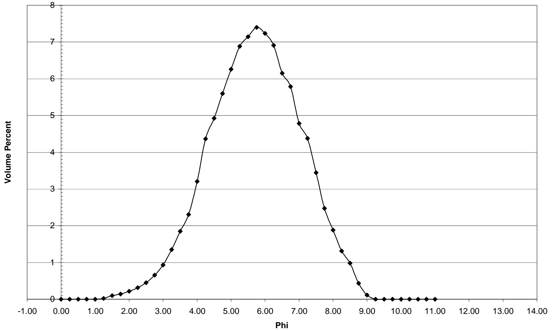
HC-36 Histogram
