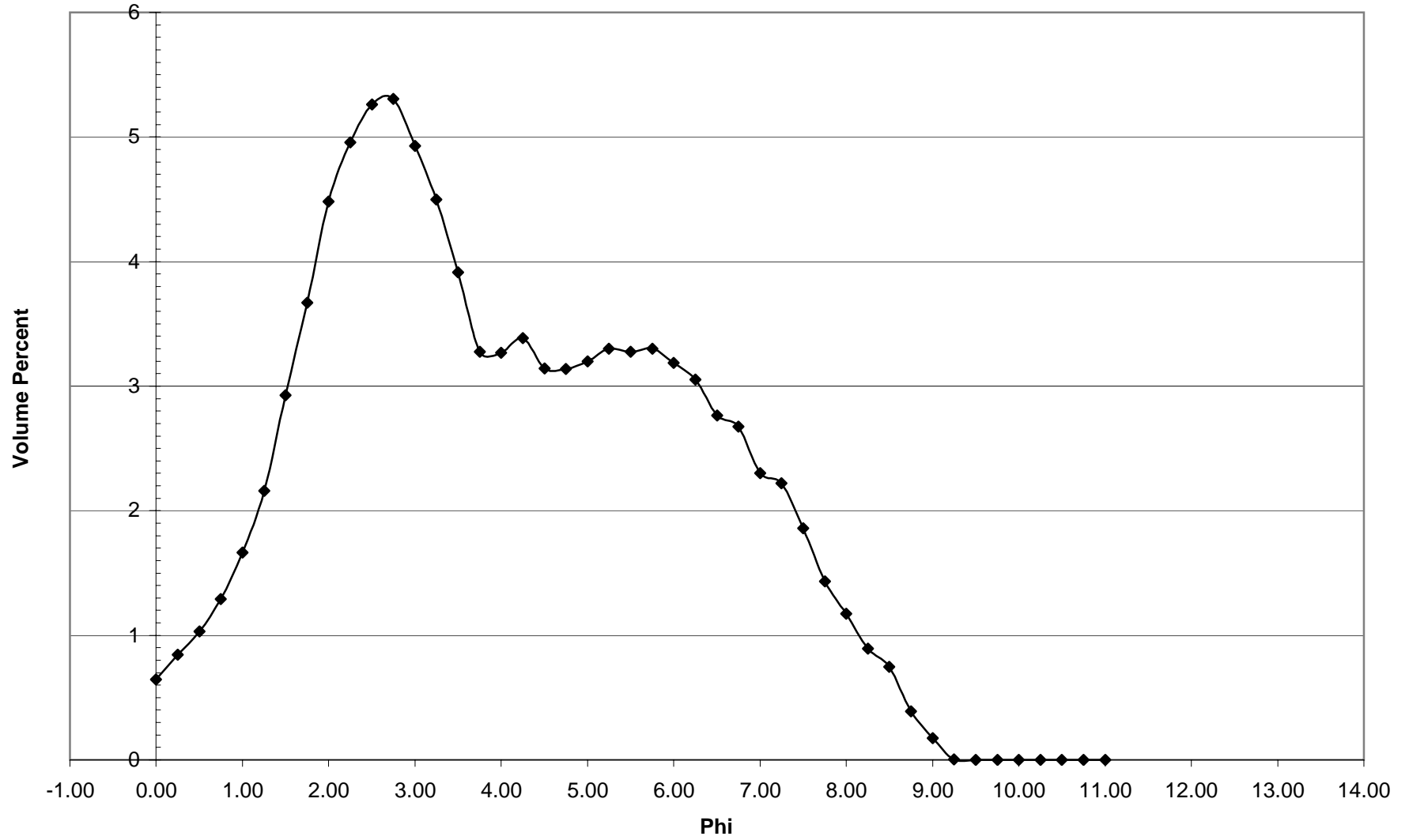
NB-02 Histogram
