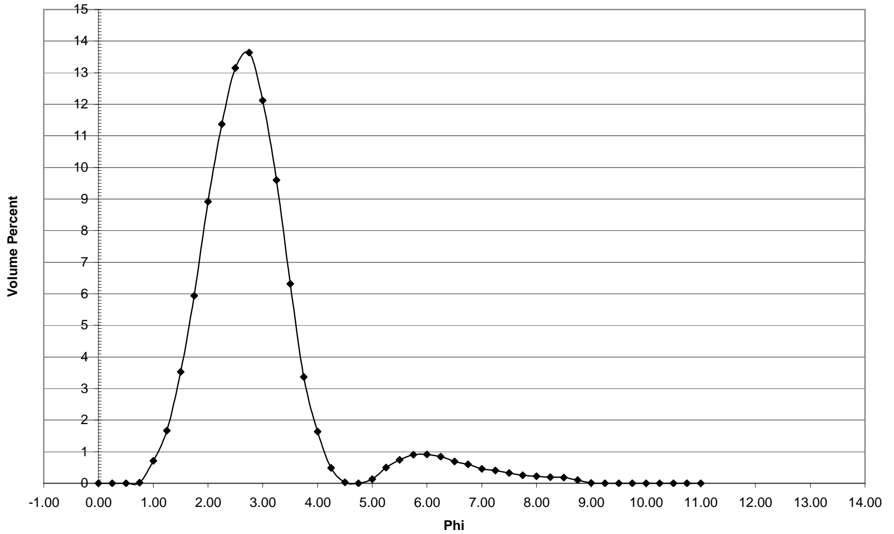
DB-53 Histogram
