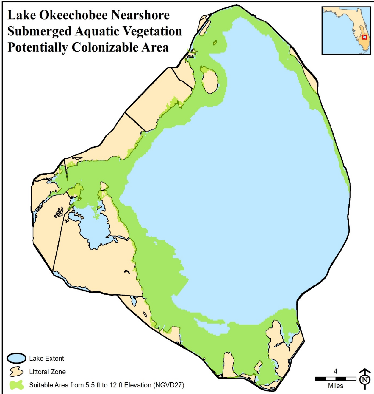
Figure 1. Nearshore green colored area is potentially colonizable by submerged aquatic vegetation (SAV). The potentially colonizable area is approximately 100,000 acres.
