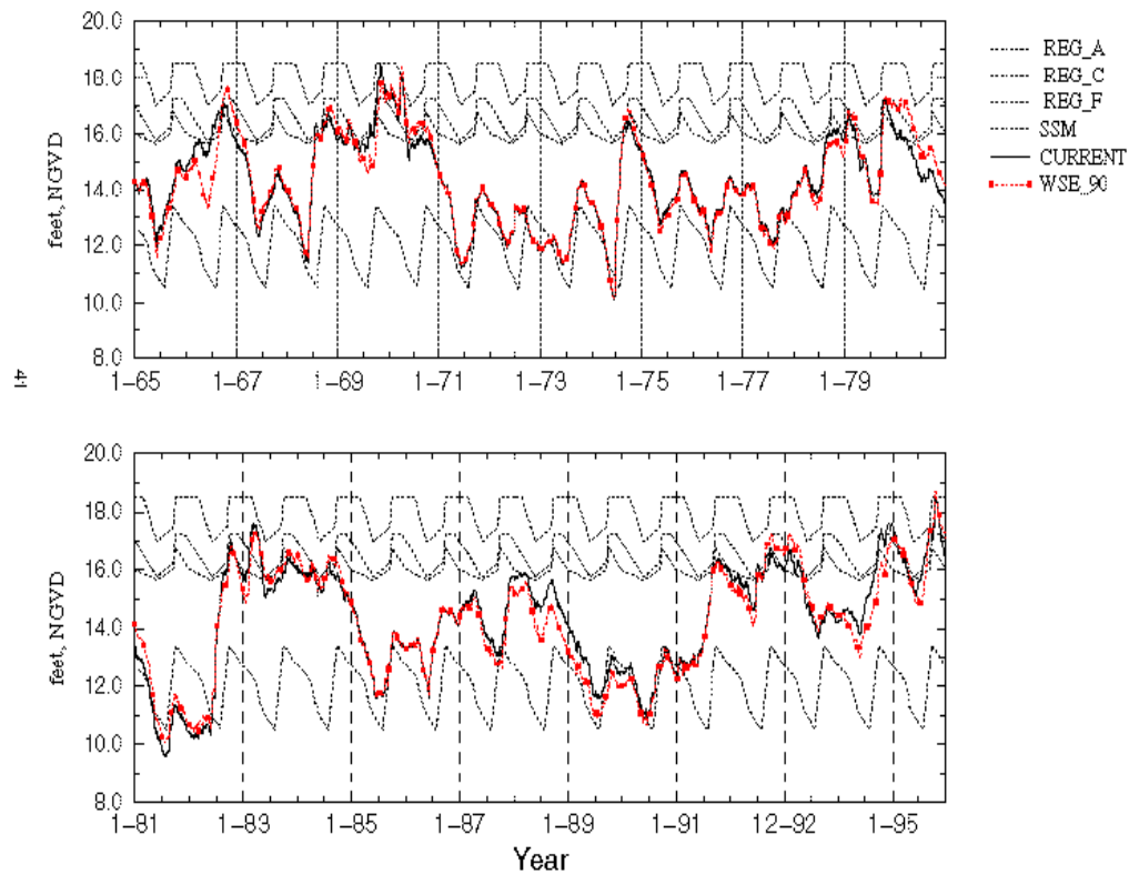
Figure 20. Comparison of Lake Okeechobee Water Level Hydrographs
