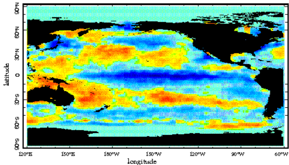
Figure 9b. Cold Sea Surface Temperature Anomaly Associated with 1989 La Nina (Florida in Drought Condition)
