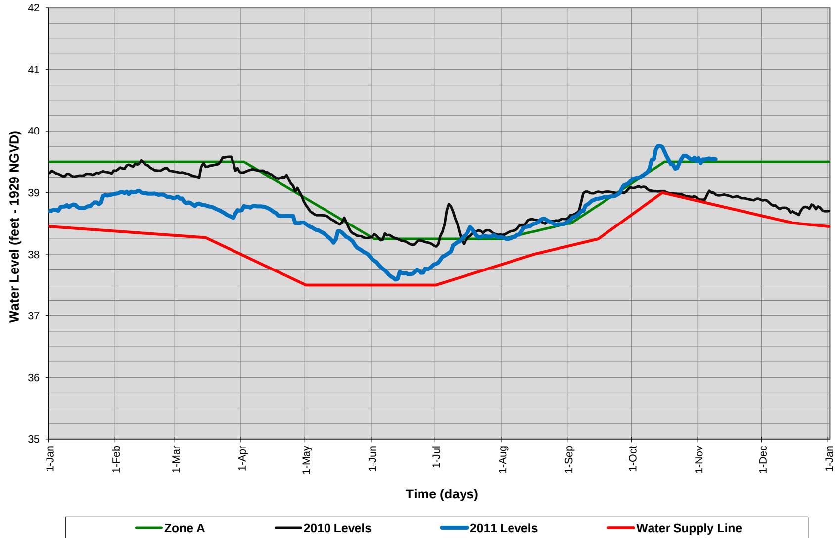
Lake Istokpoga Actual and Minimum Levels
