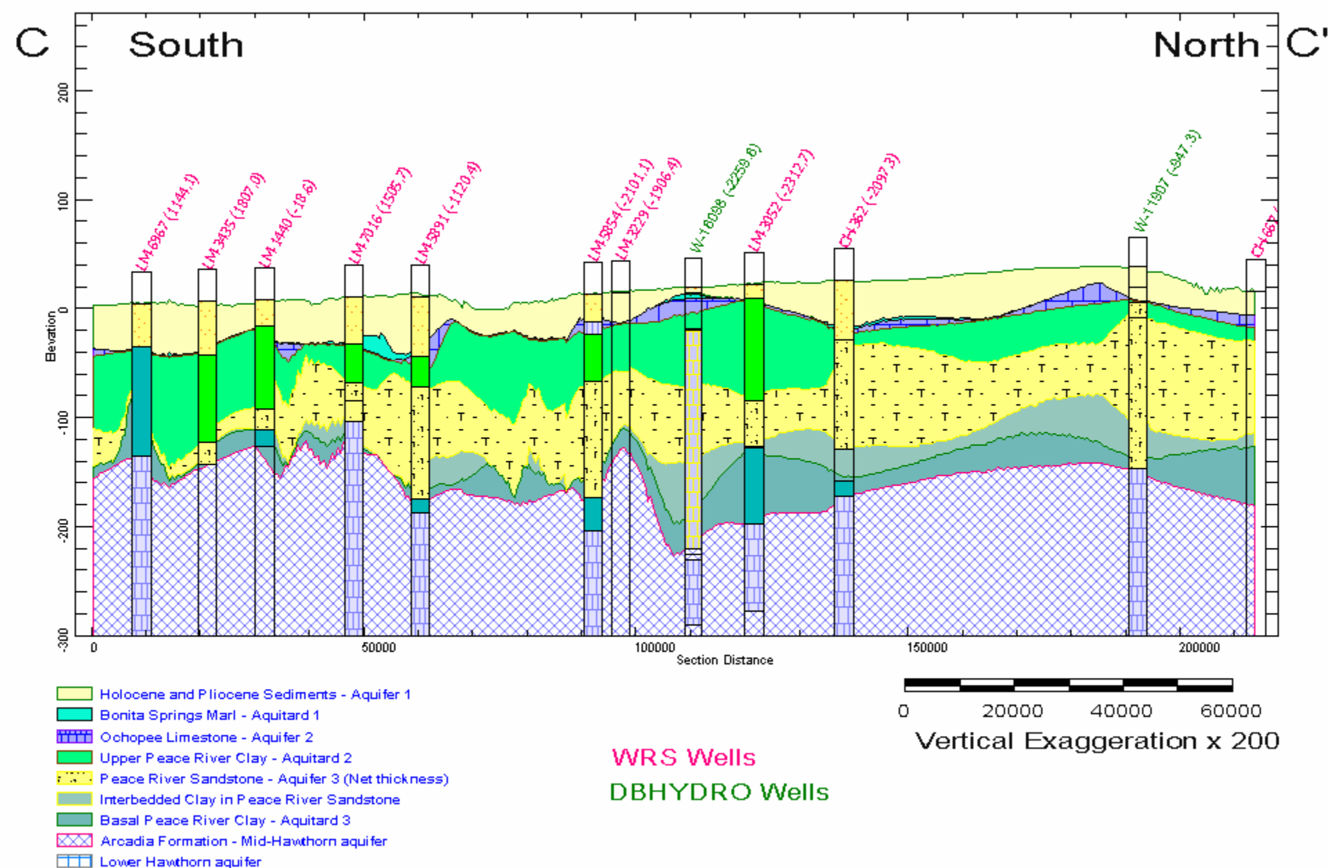
Figure 23: North-South Section C-C'
