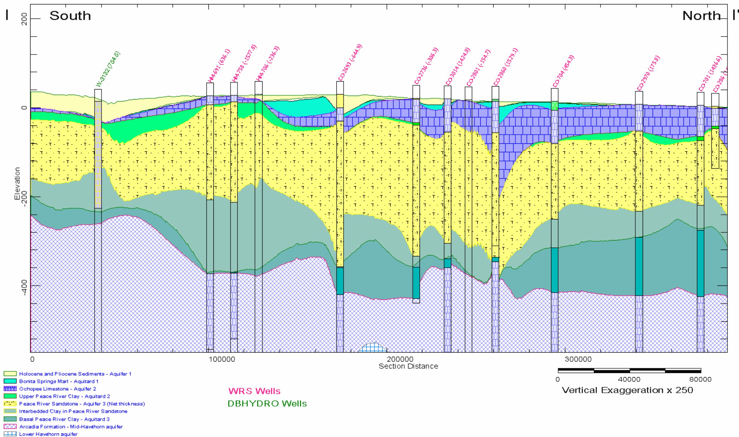
Figure 29: North-South Section I-I'
