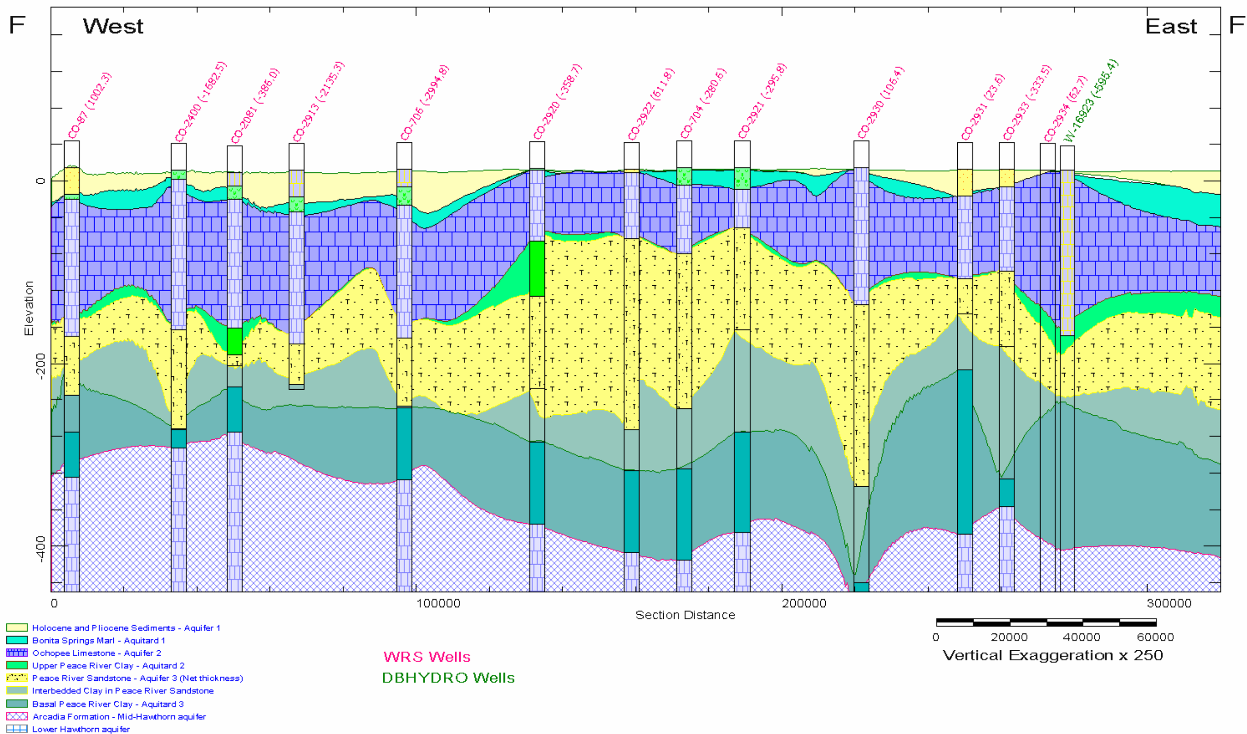
Figure 26: East-West Section F-F'
