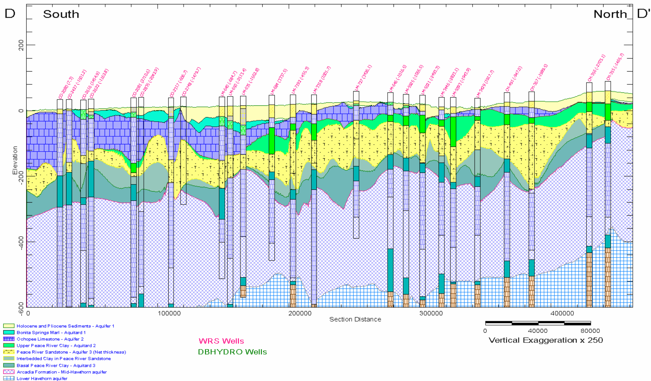
Figure 24: North-South Section D-D'
