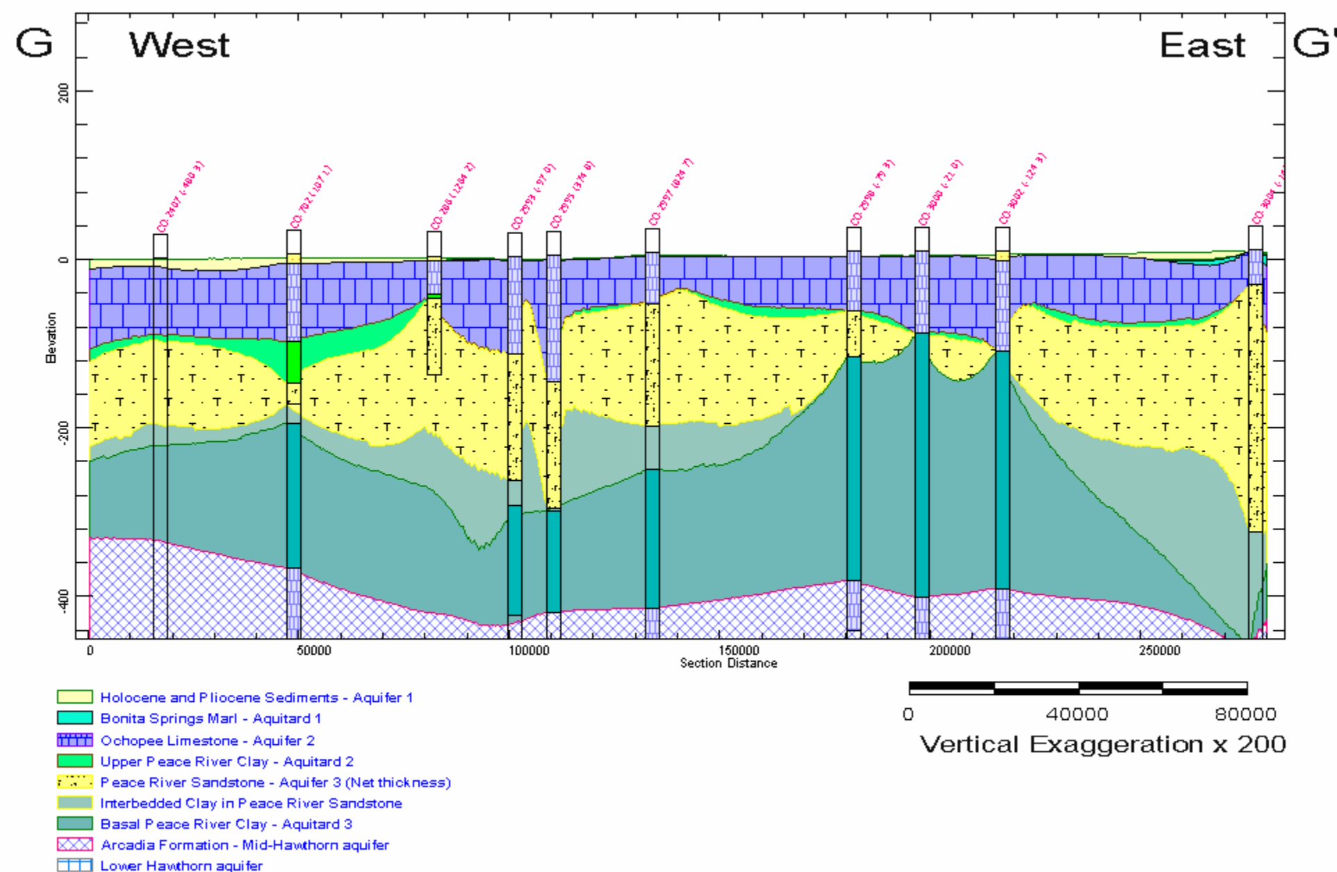
Figure 27: East-West Section G-G'
