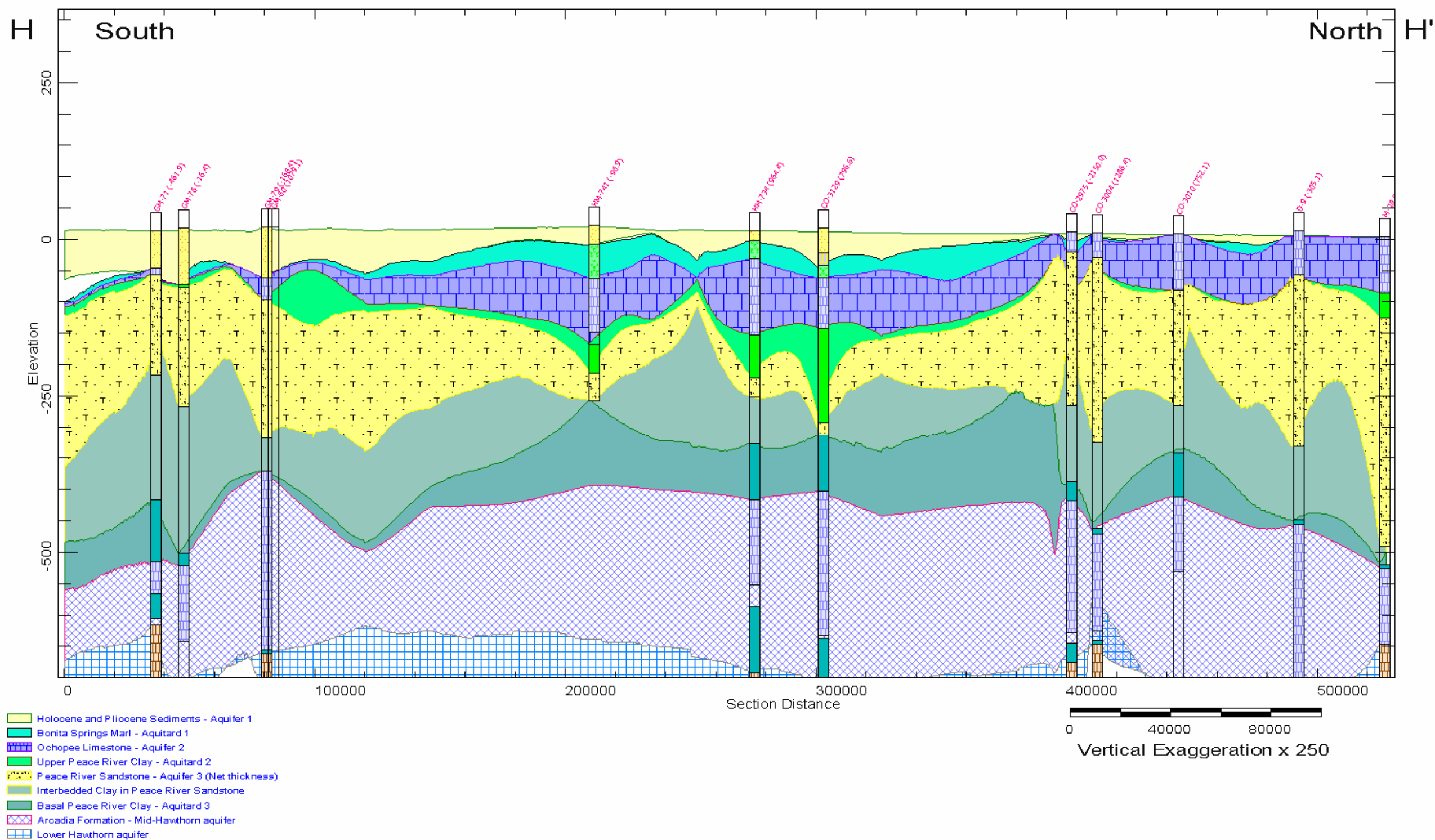
Figure 28: North-South Section H-H'
