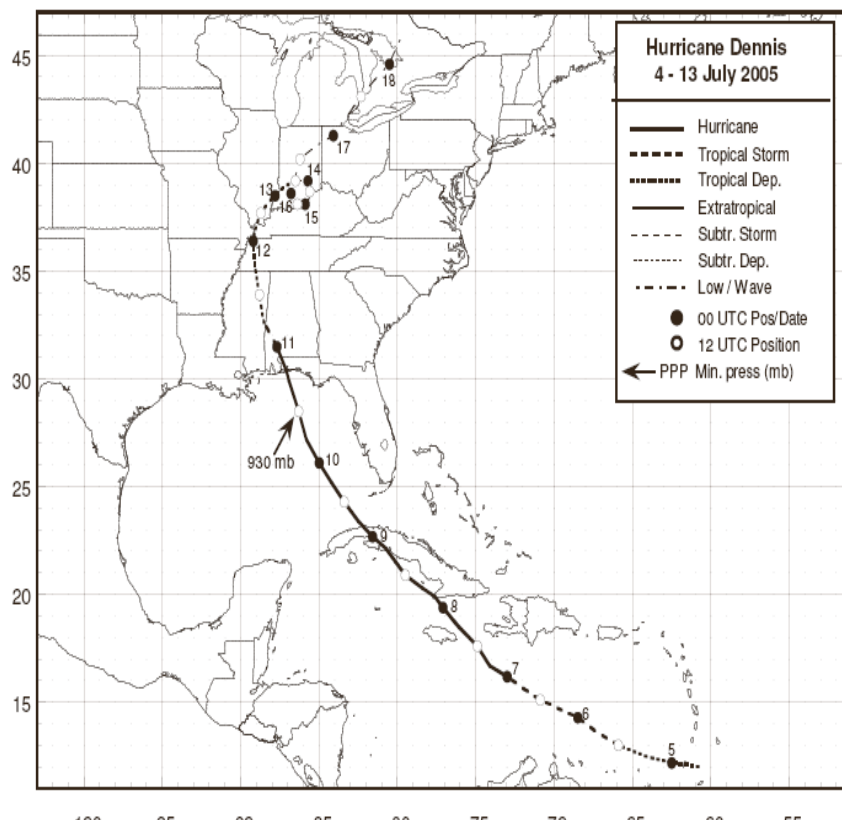
Figure 9a. Path and development of Hurricane Dennis from July 4 -13, 2005 (Beven, 2005).
