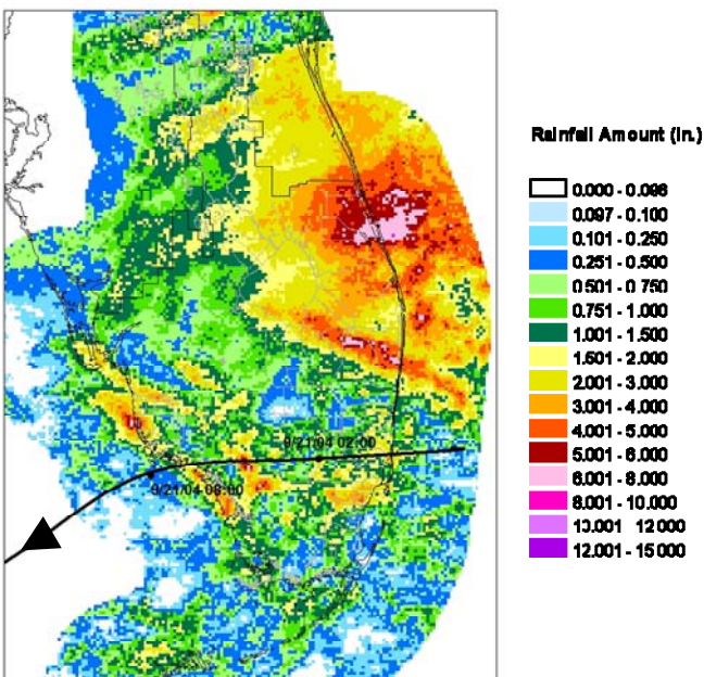
Figure 1c. Hurricane Ivan's path and radar rainfall (September 19–23, 2004).
