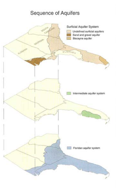
Figure 3. Area and extent of three major aquifer systems in Florida (Fernald and Purdum, 1998).
