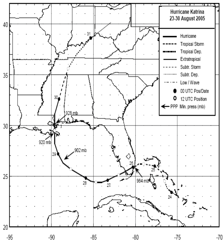
Figure 10a. Path and development of Hurricane Katrina during August 23-30, 2005 (Knabb et al., 2005).
