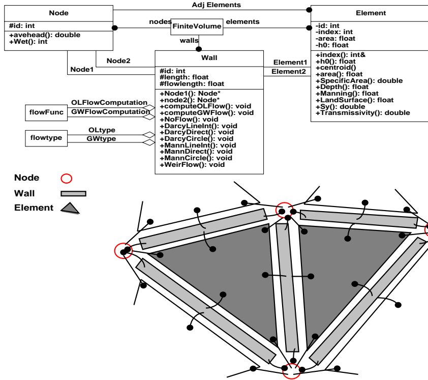
Figure 1: Object diagram and its relationship to the model domain.
