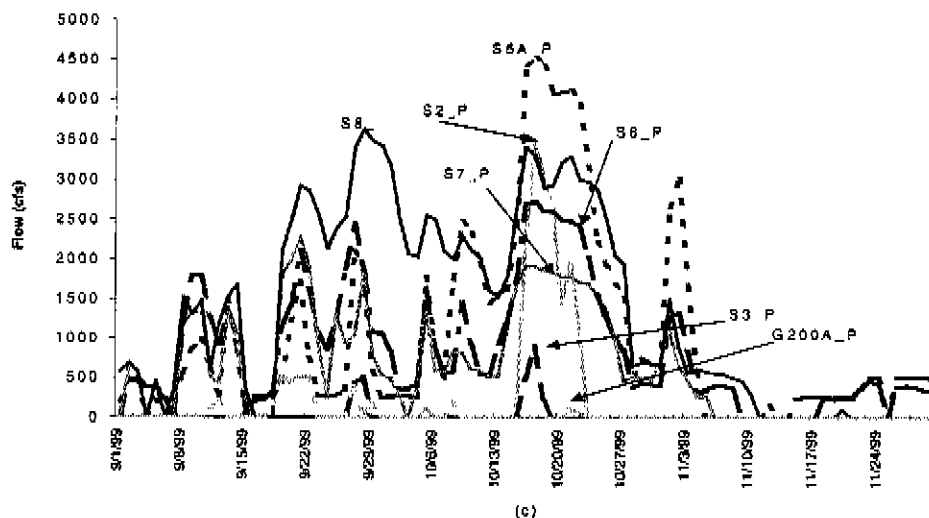
Figures 7a to c. Daily Average Flow for Pump Stations – September 1 through November 30, 1999.
