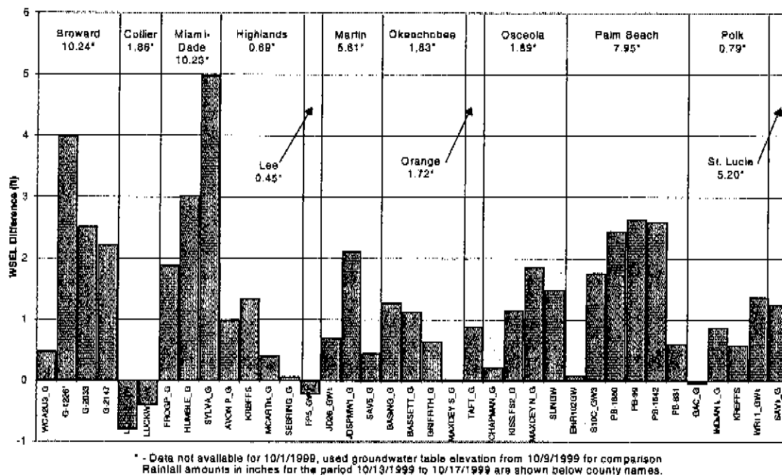
Figure 24. Groundwater Table Elevation Differences at 37 Selected Wells.
