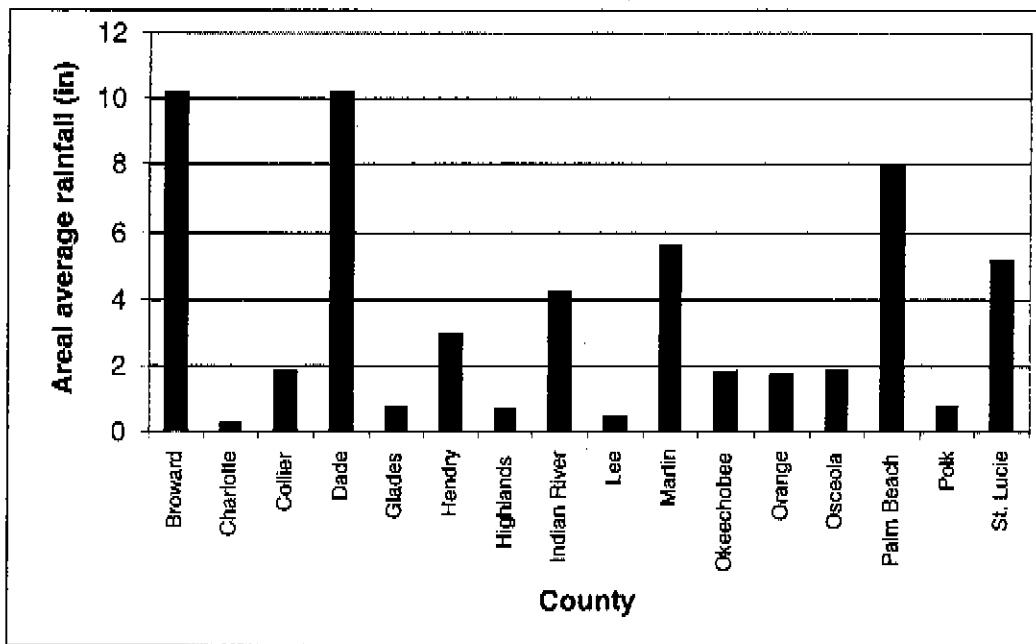
Figure 4. Hurricane Irene Areal Average Rainfall by County (October 13 through 17, 1999).
