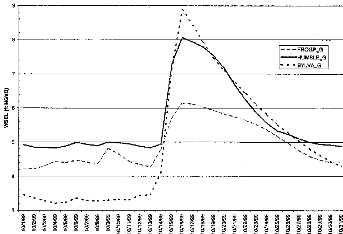
Figure 23. Groundwater Table Elevations at 3 Wells in Miami-Dade County - October 1999.
