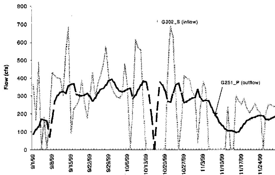
Figure 11. Inflow and Outflow to STA-6 - September 1 to November 30, 1999.
