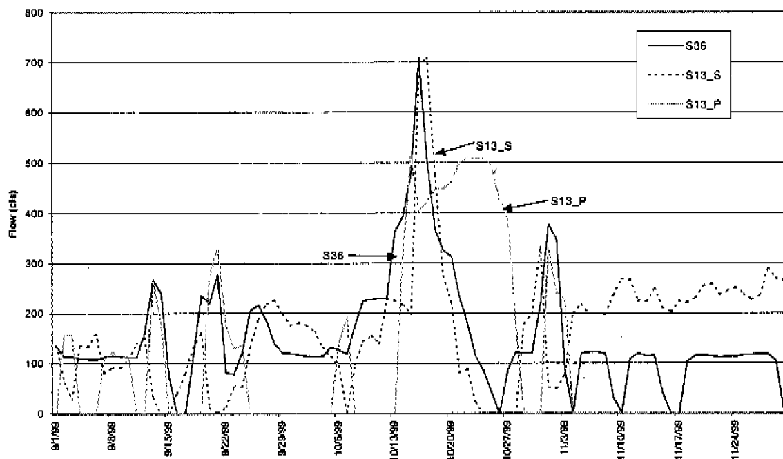
Figure 9d. Daily Average Outflow for Selected Coastal Structures – September 1 through November 30, 1999.
