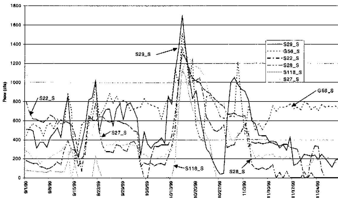
Figure 9b. Daily Average Outflow for Selected Coastal Structures – September 1 through November 30, 1999.
