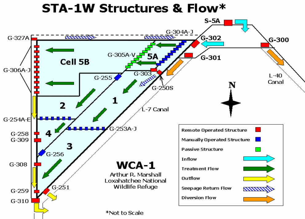
Figure 1. Configuration of sampling stations and flows in STA-1W as of October 2005.
