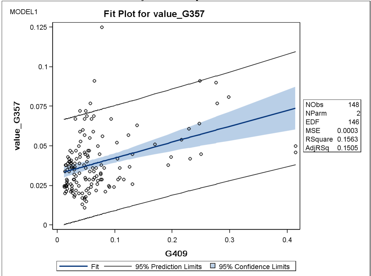
Figure 9. Linear regression of TPO4 concentrations collected by autosampler at stations G357 and G409.
