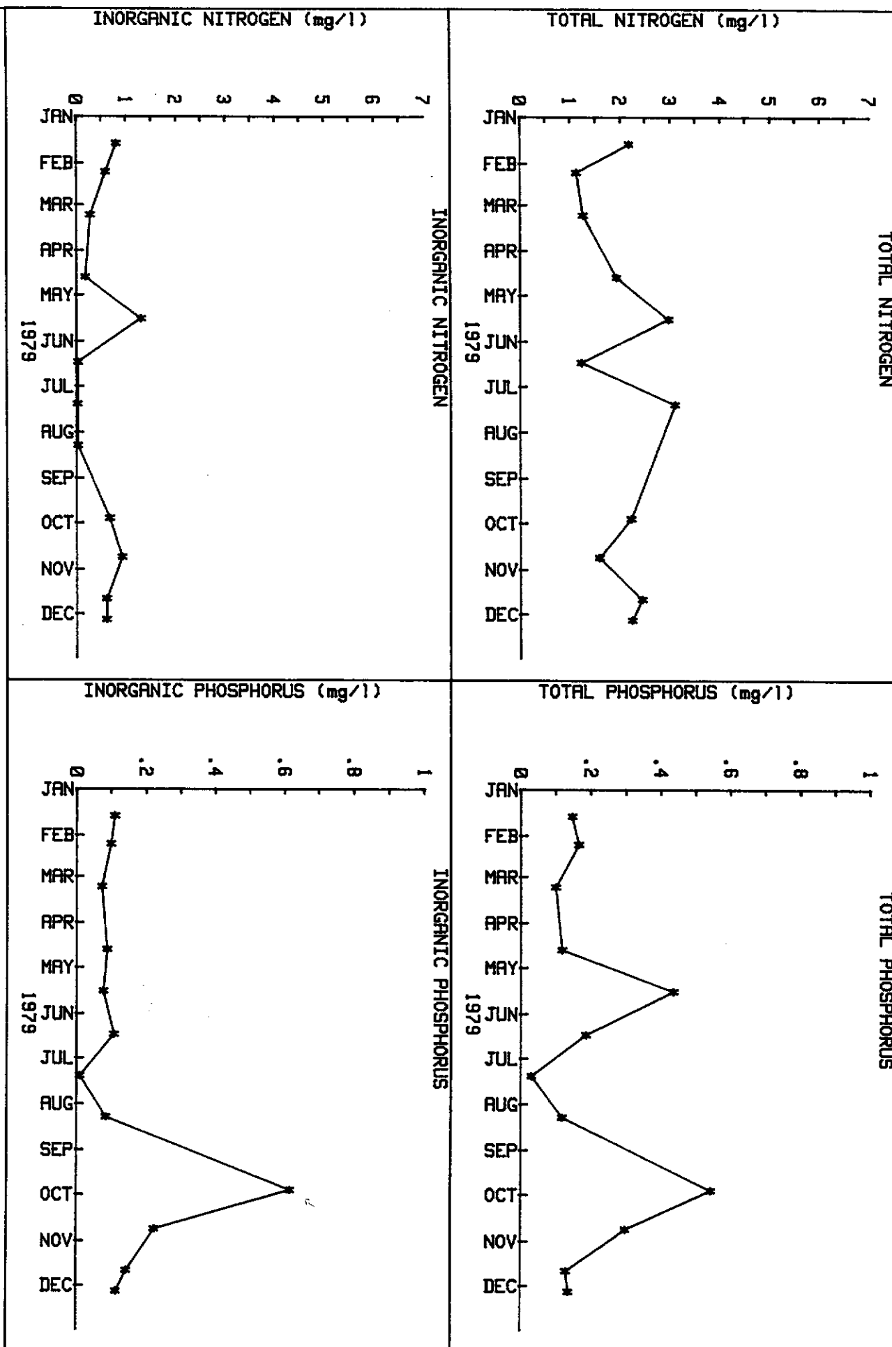
FIGURE . WATER QUALITY DATA VS TIME FOR C-15 AT SR 809
