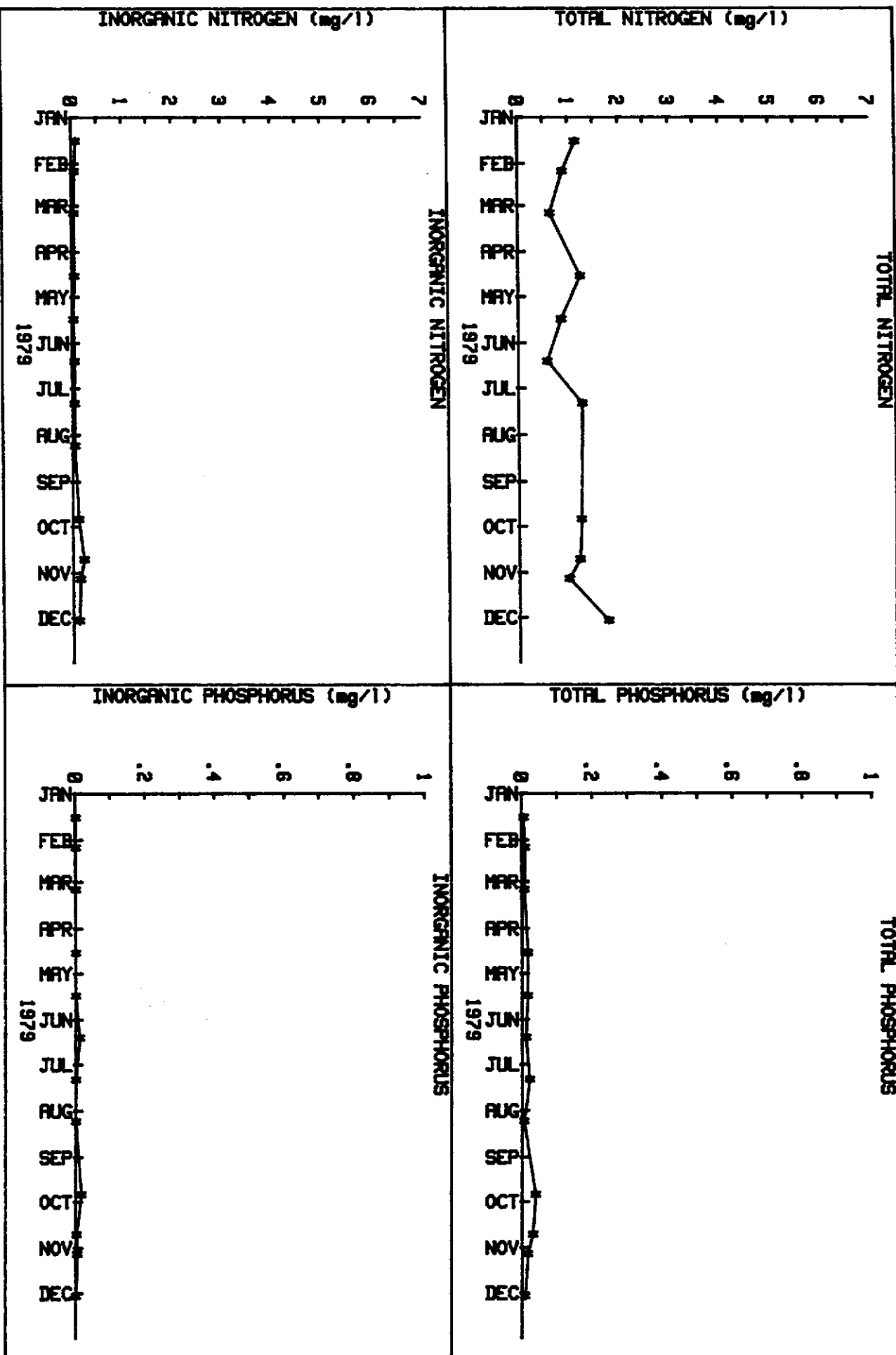
FIGURE . WATER QUALITY DATA VS TIME FOR THE GOLDEN GATE CANAL AT SR 951
