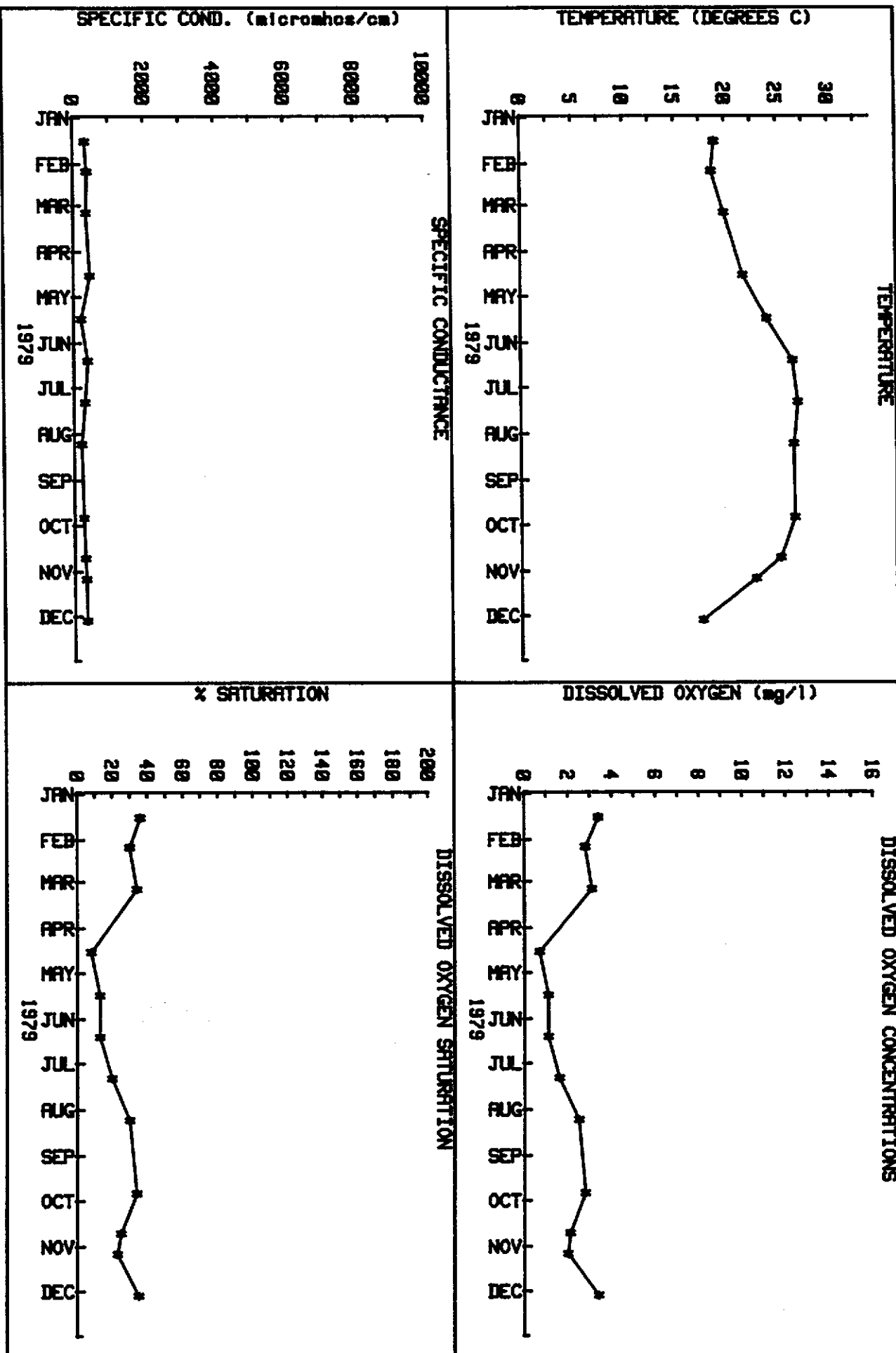
FIGURE . FIELD DATA VS TIME FOR THE TAMiami CNAL AT BRIDGE #105
