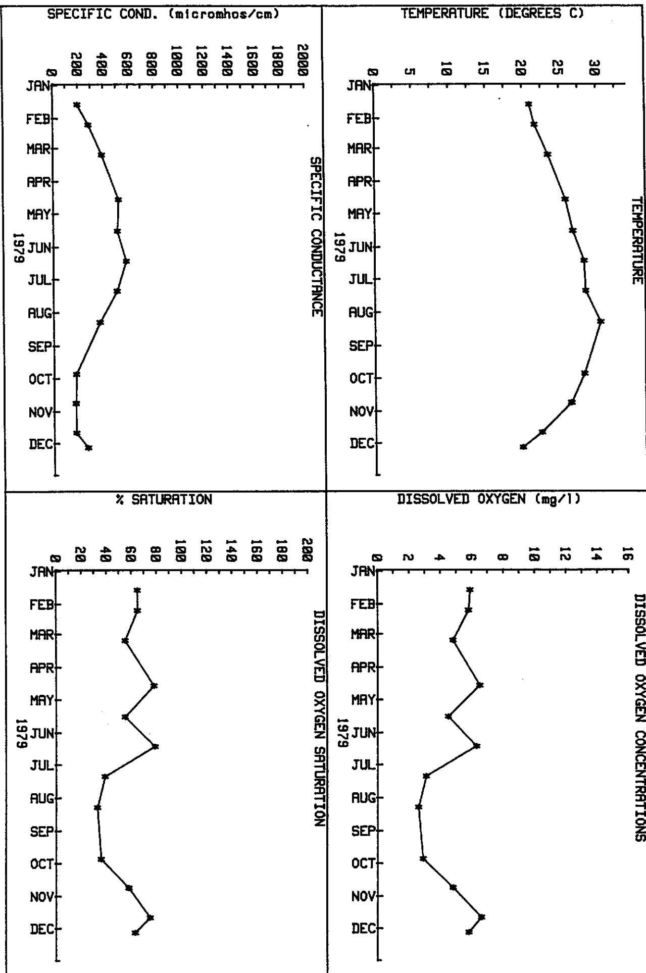
FIGURE . FIELD DATA VS TIME FOR C-18 AT S.R. 710
