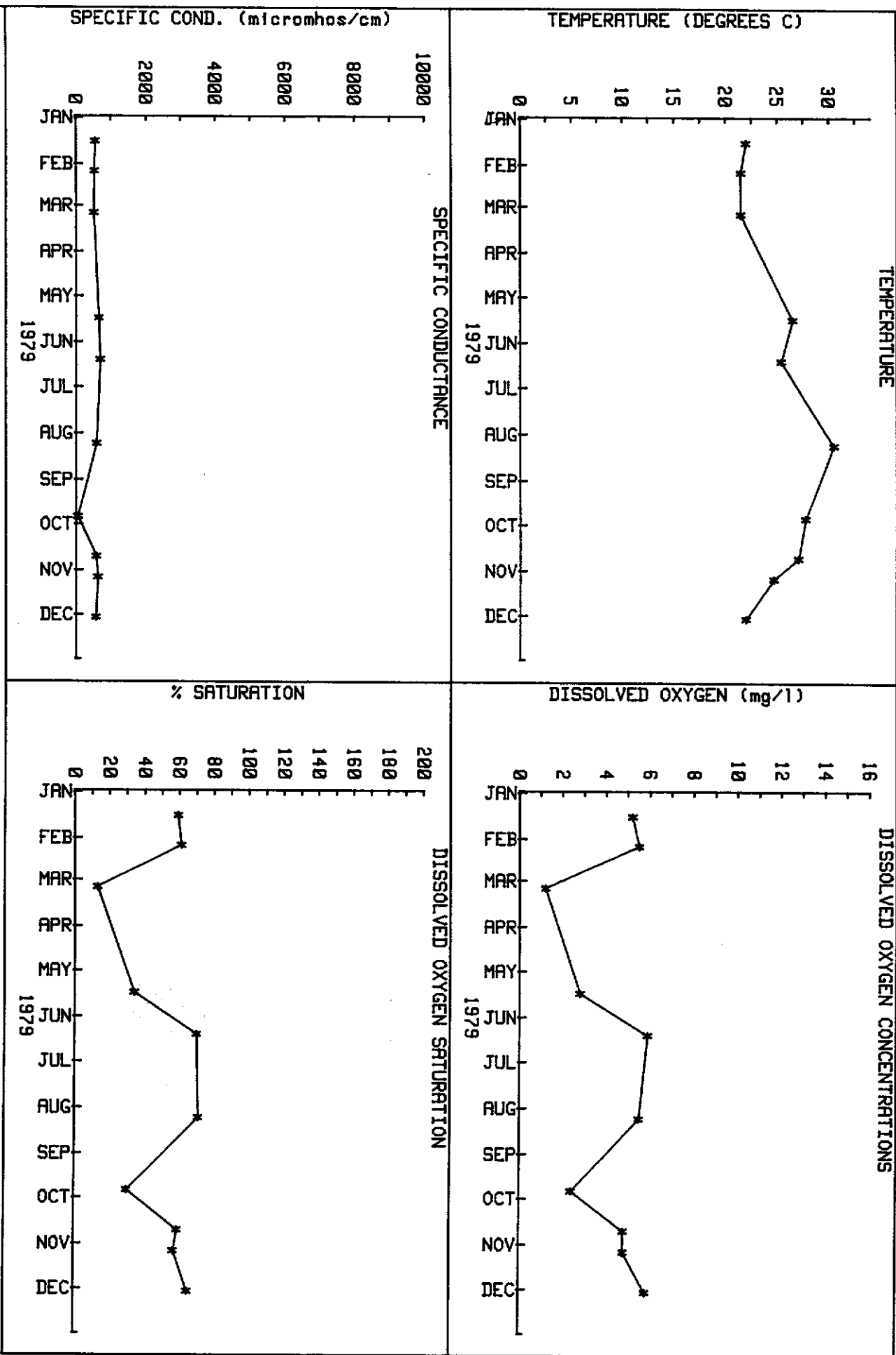
FIGURE . FIELD DATA VS TIME FOR THE COCOHATCHEE CANAL AT S.R. 951
