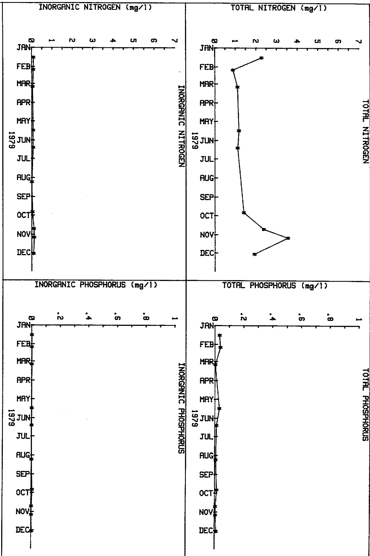
FIGURE . WATER QUALITY DATA VS TIME FOR THE COCOHATCHEE CANAL AT SR 951
