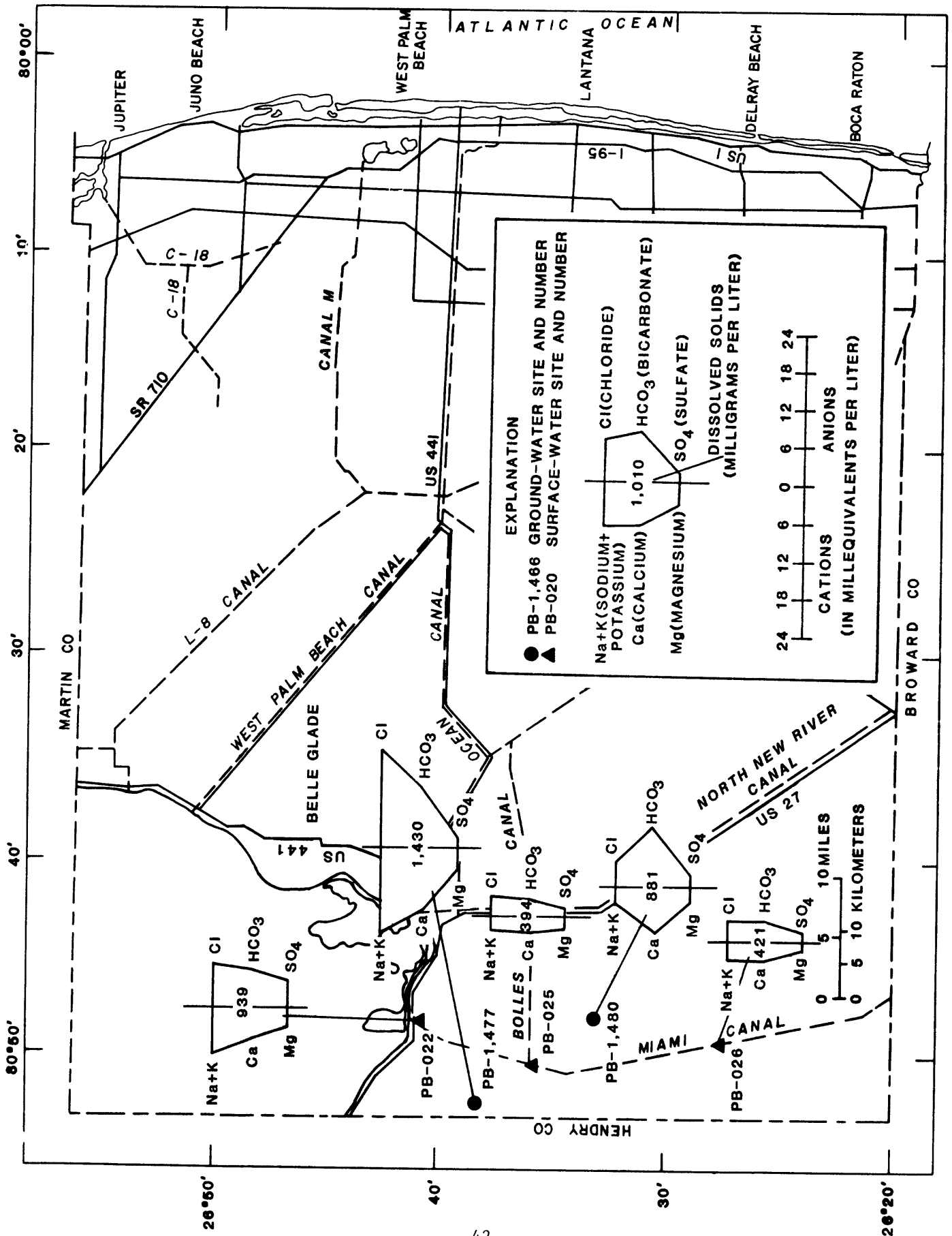
Figure 17.--Chemical composition of water in Miami Canal and nearby wells, April 1984.
