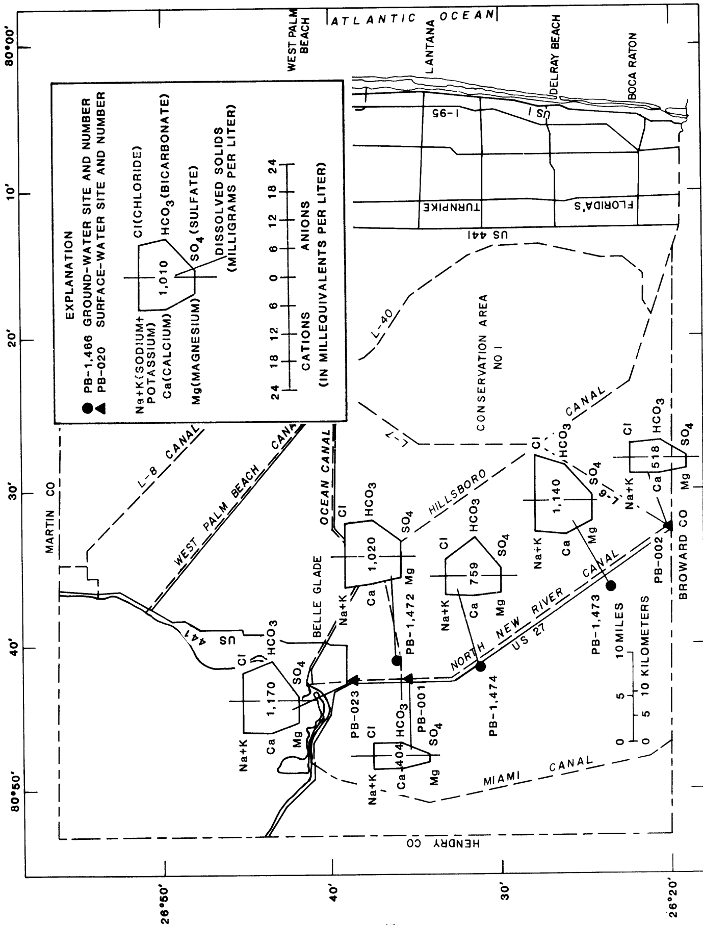
Figure 16.--Chemical composition of water in North New River Canal and nearby wells, April 1984.
