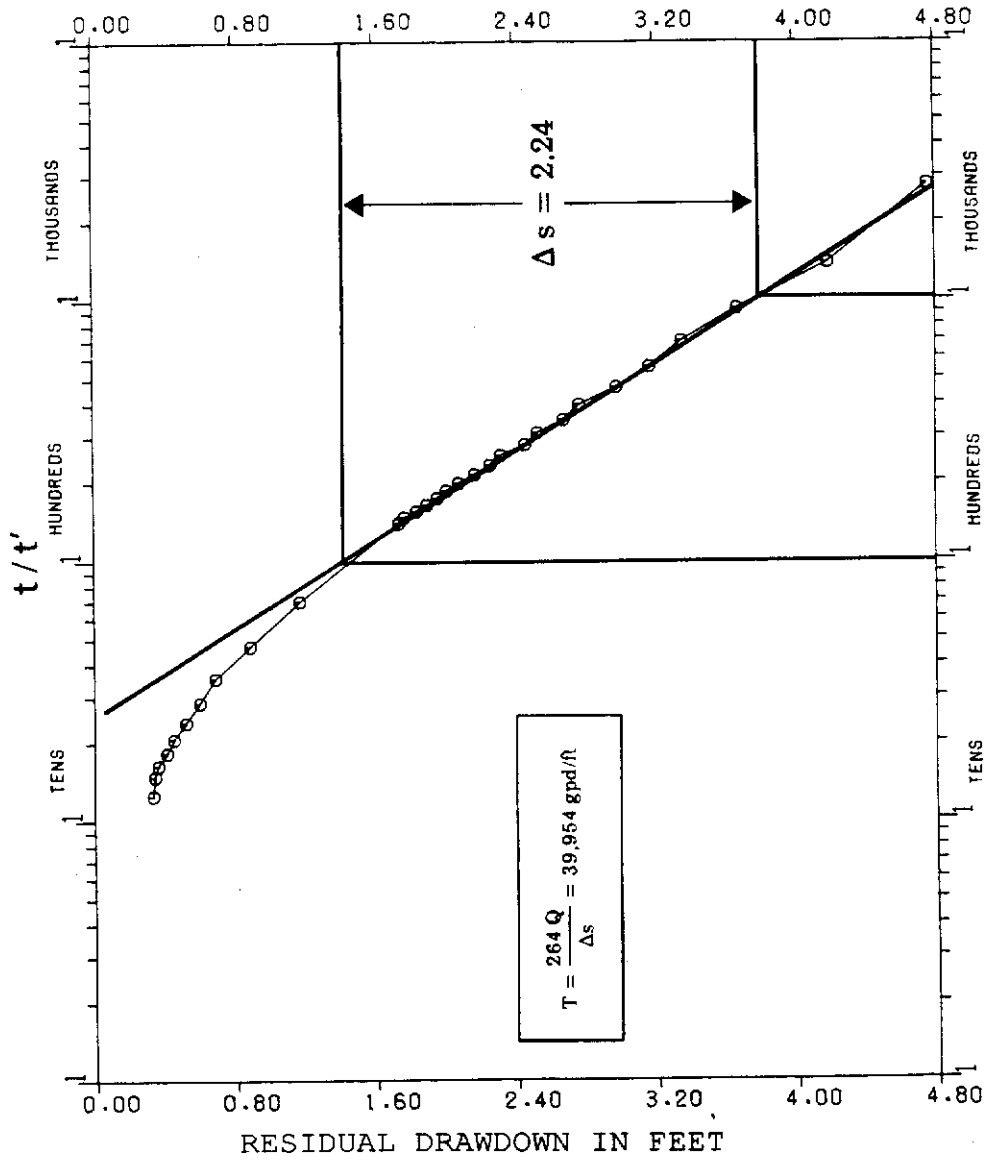
GRAPH 3. L-65 APT Recovery: Observation Well D
