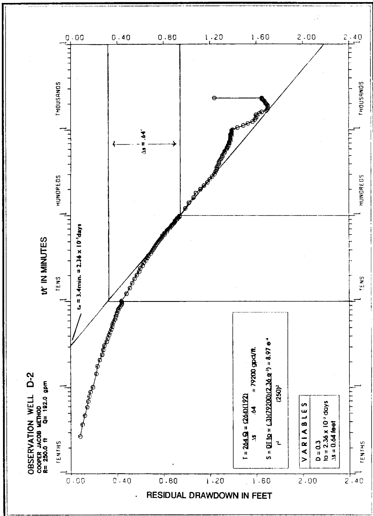
GRAPH 37. STLAPT 2 APT Recovery: Observation Well D-2
