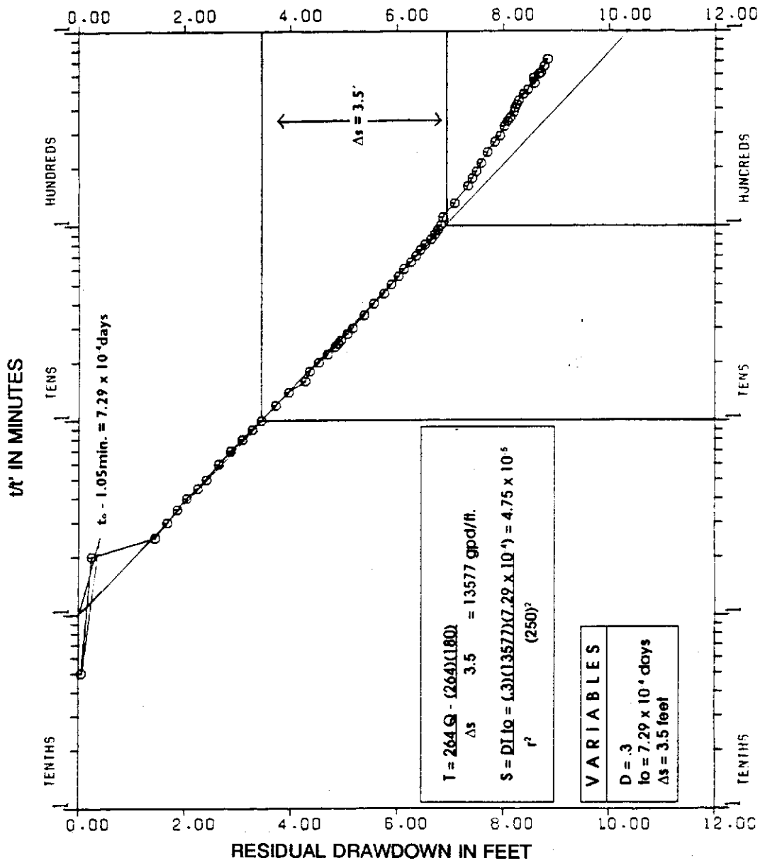
GRAPH 72. Monte Carlo Country Club APT Drawdown: Observation Well OBS3 (Jacob Method)
