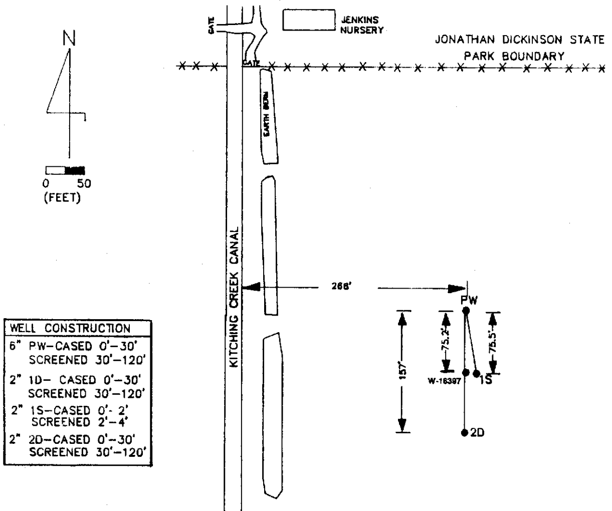
FIGURE 46. Site Layout and Well Construction Details- Jonathan Dickinson State Park APT Site
