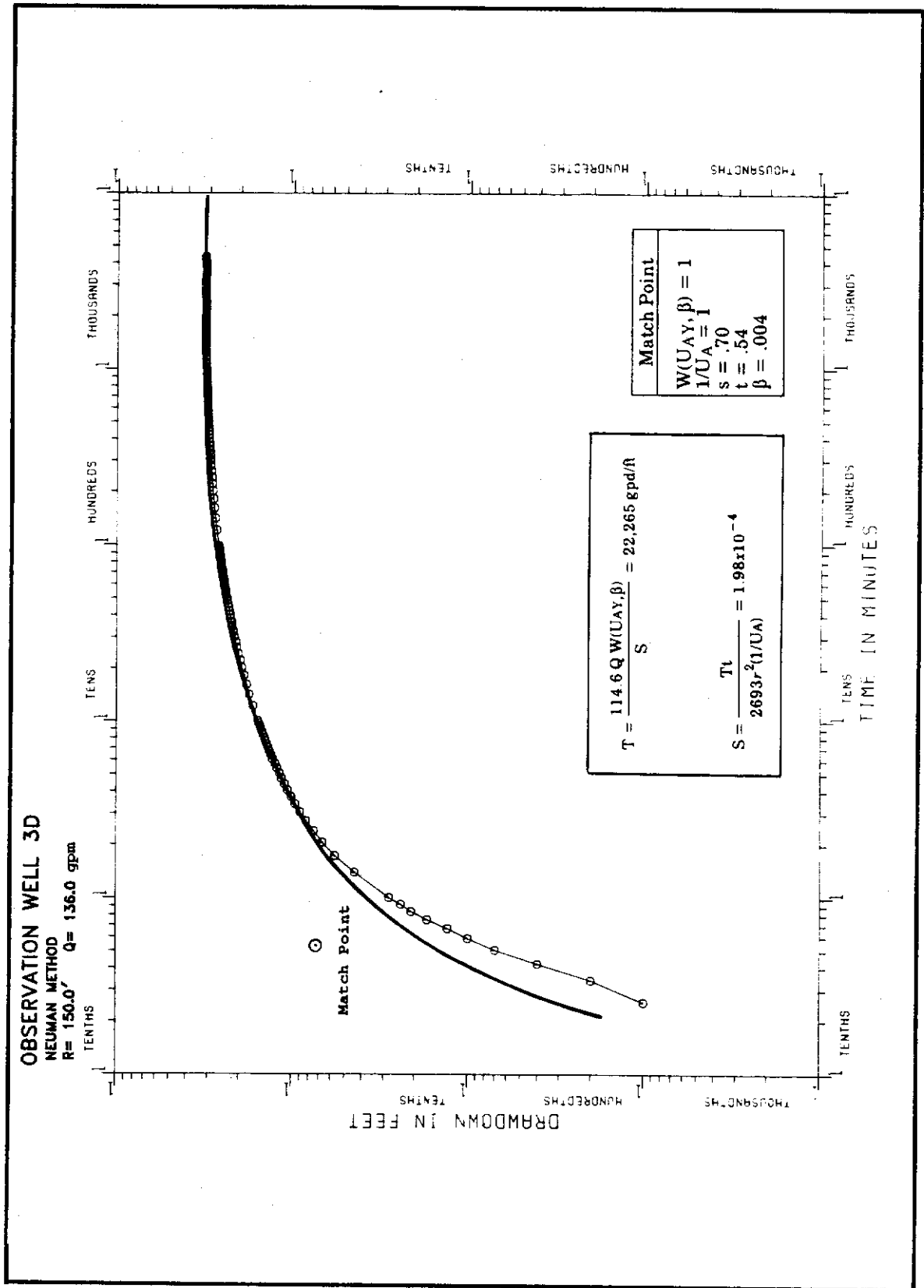
GRAPH 21. Monreve Ranch APT Drawdown: Observation Well 3D
