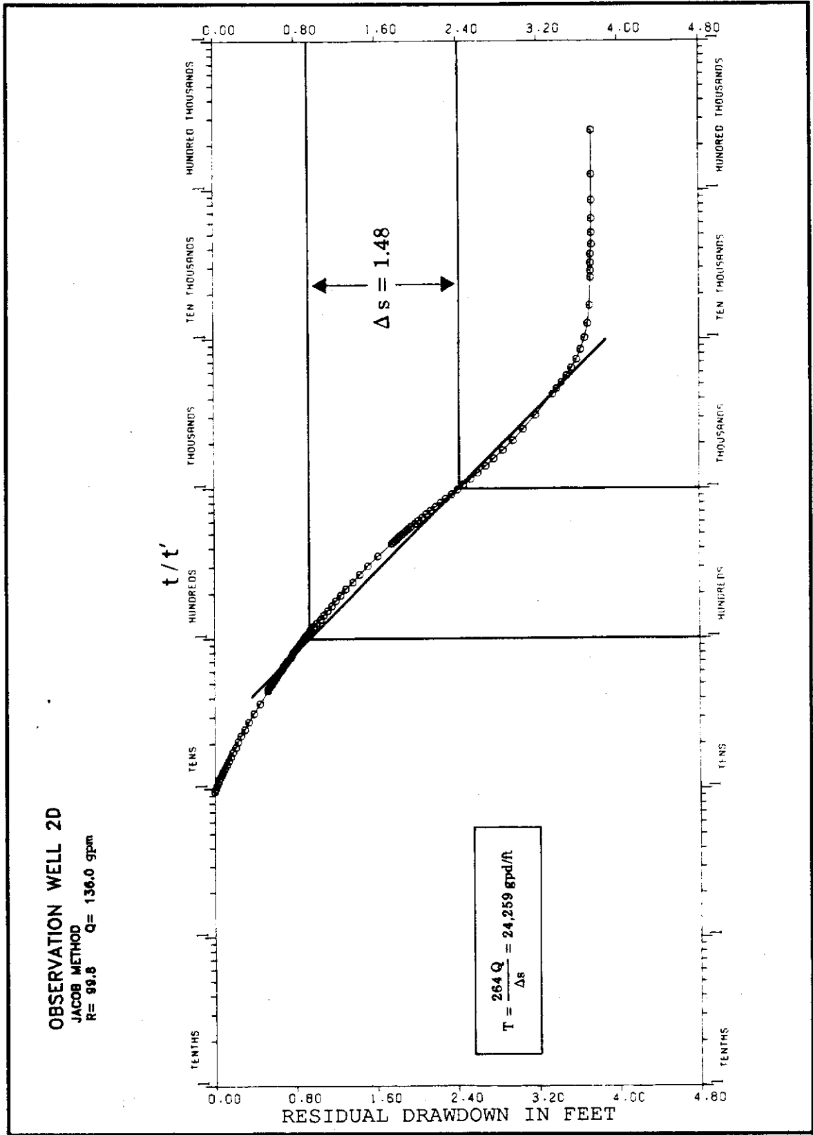
GRAPH 22. Monreve Ranch APT Recovery: Observation Well 2D
