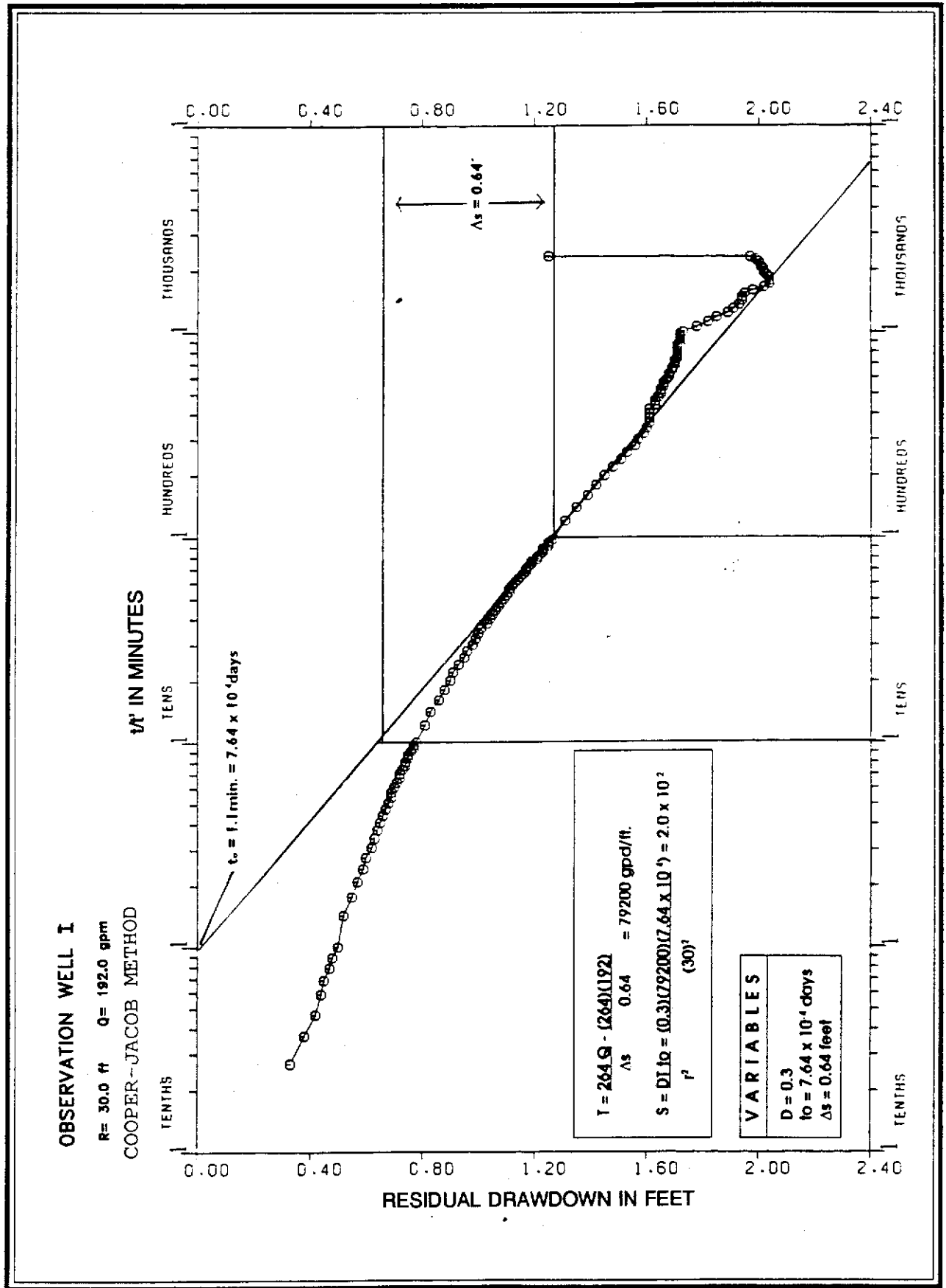
GRAPH 38. STLAPT 2 APT Drawdown: Observation Well D-3
