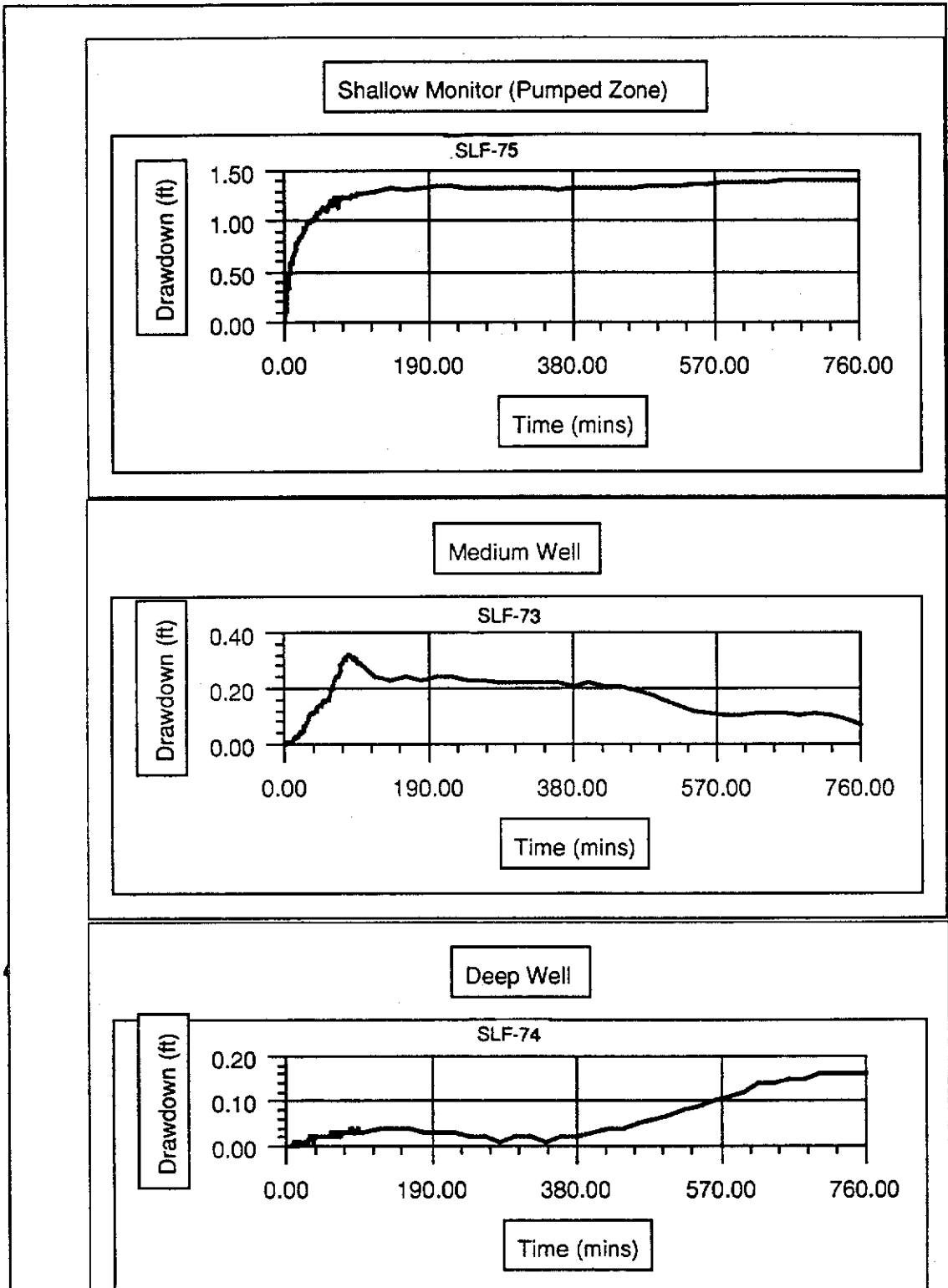
FIGURE 72. Water-Level Drawdowns in three Floridan Aquifer System Zones (Wells SLF-73, SLF-74 and SLF-75) while Pumping the Shallow Zone (SLF-75)
