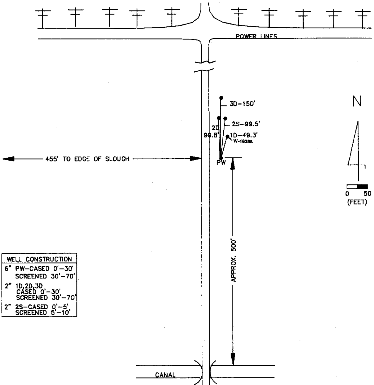
FIGURE 52. Site Layout and Well Construction Details - Monreve Ranch APT Site
