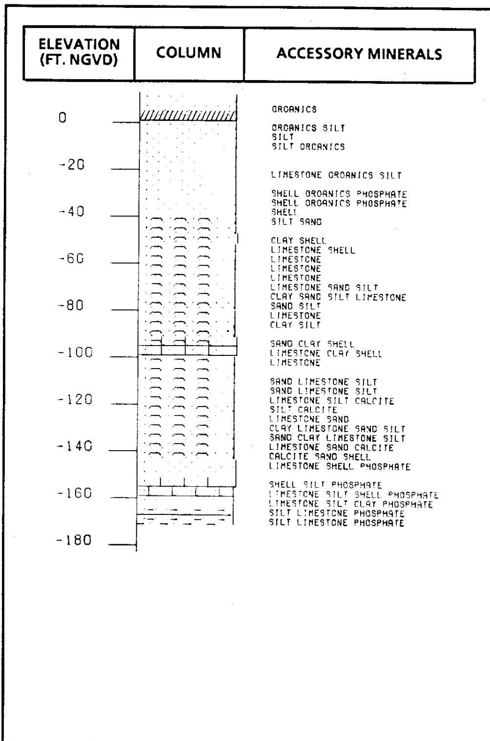
FIGURE 50. Lithologic Column for Well W-16460, Mobil (TP&J) APT Site
