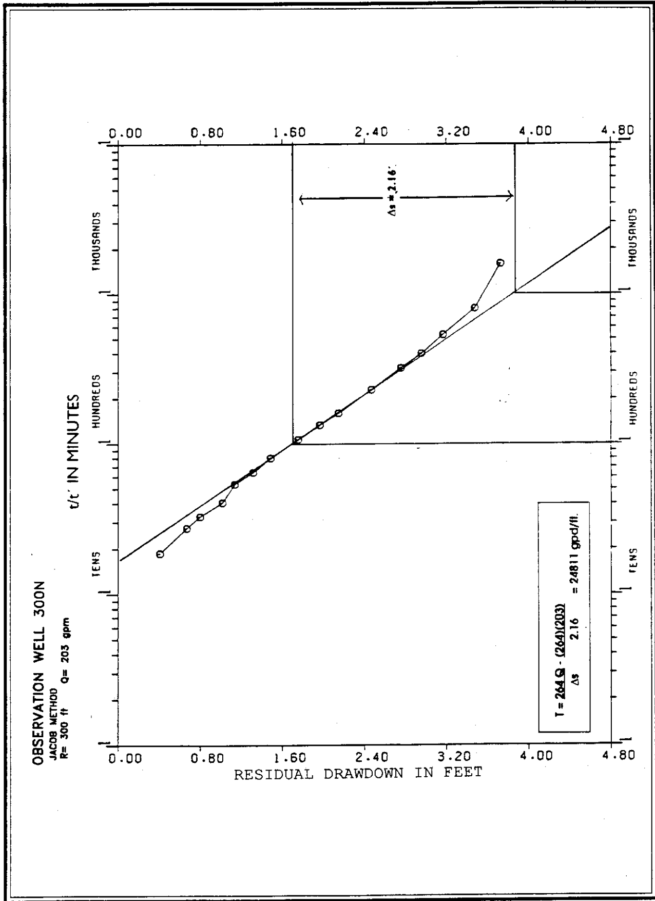
GRAPH 54. Indrio Road APT Recovery: Observation Well 300N
