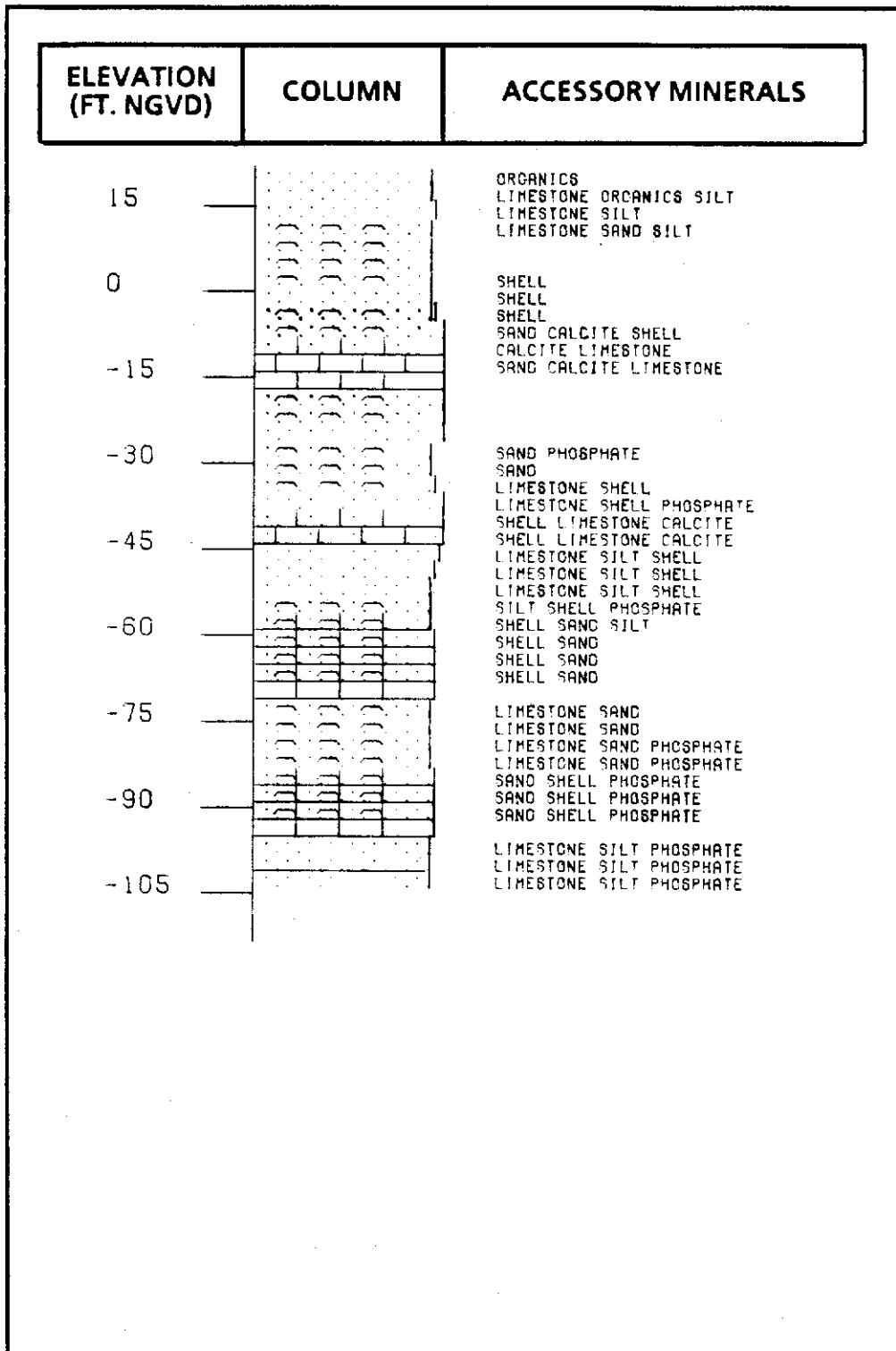
FIGURE 53. Lithologic Column for Well W-16398, Monreve Ranch APT Site
