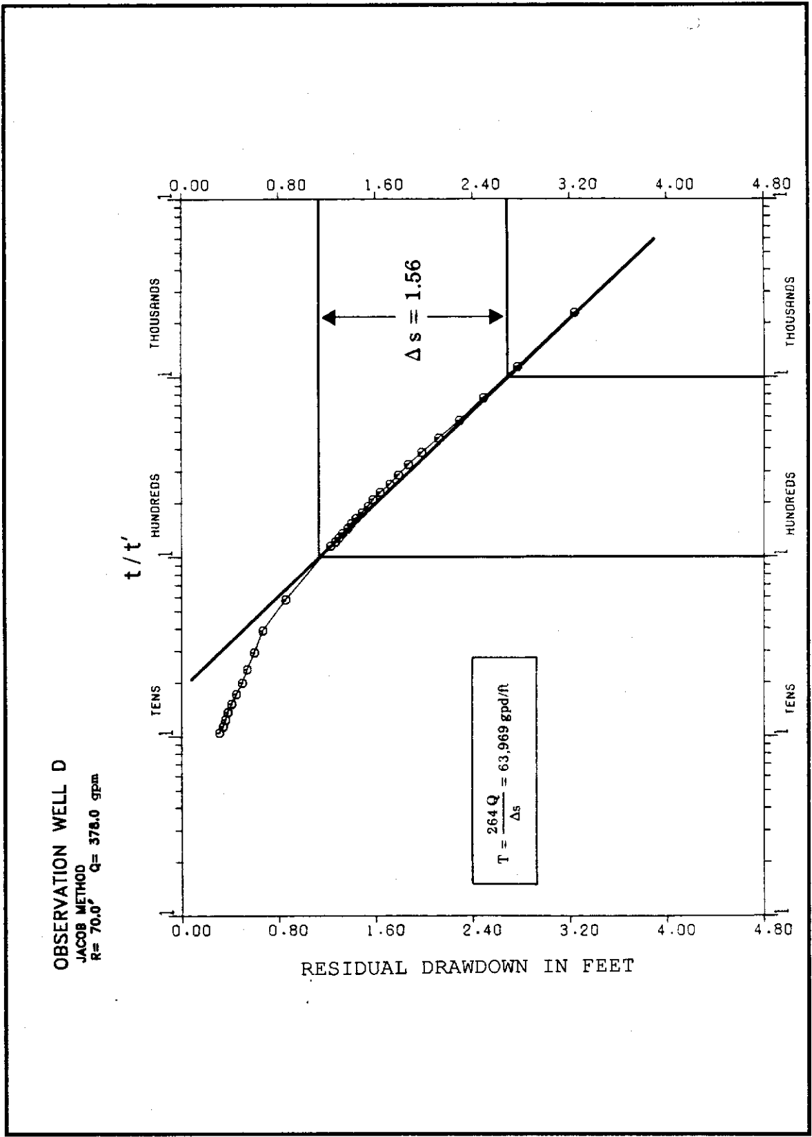
GRAPH 7. Caulkin's Grove APT Recovery: Observation Well D
