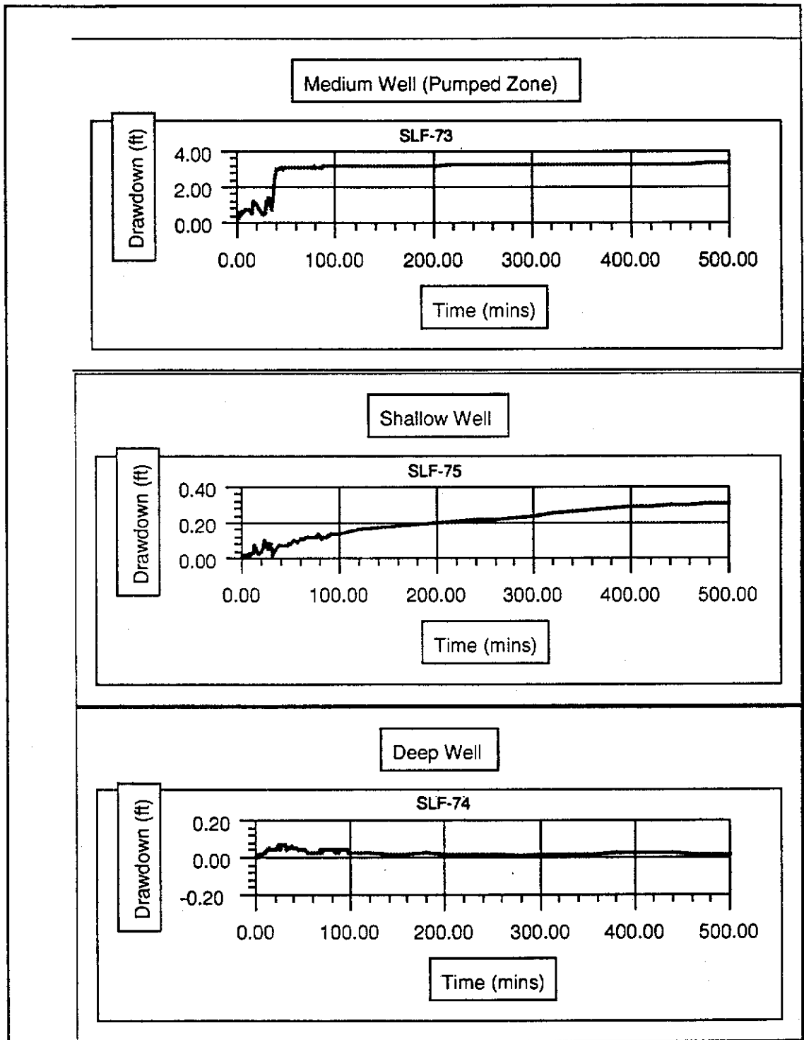
FIGURE 73. Water-Level Drawdowns in three Floridan Aquifer System Zones (Wells SLF-73, SLF-74 and SLF-75) while Pumping the Middle Zone (SLF-76)
