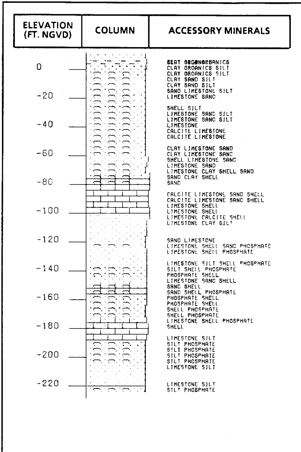
FIGURE 47. Lithologic Column - Jonathan Dickinson State Park APT Site
