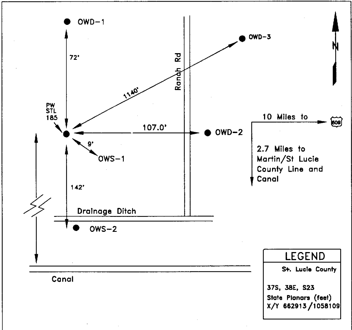
FIGURE 65. Location Map and Site Layout - McCarty Ranch APT Site
