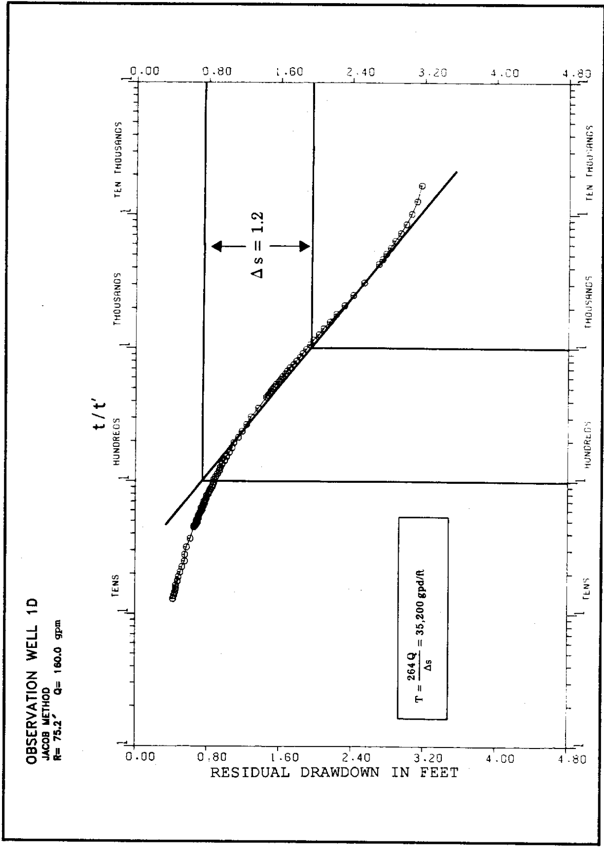
GRAPH 11. Jonathan Dickinson State Park APT Recovery: Observation Well 1D
