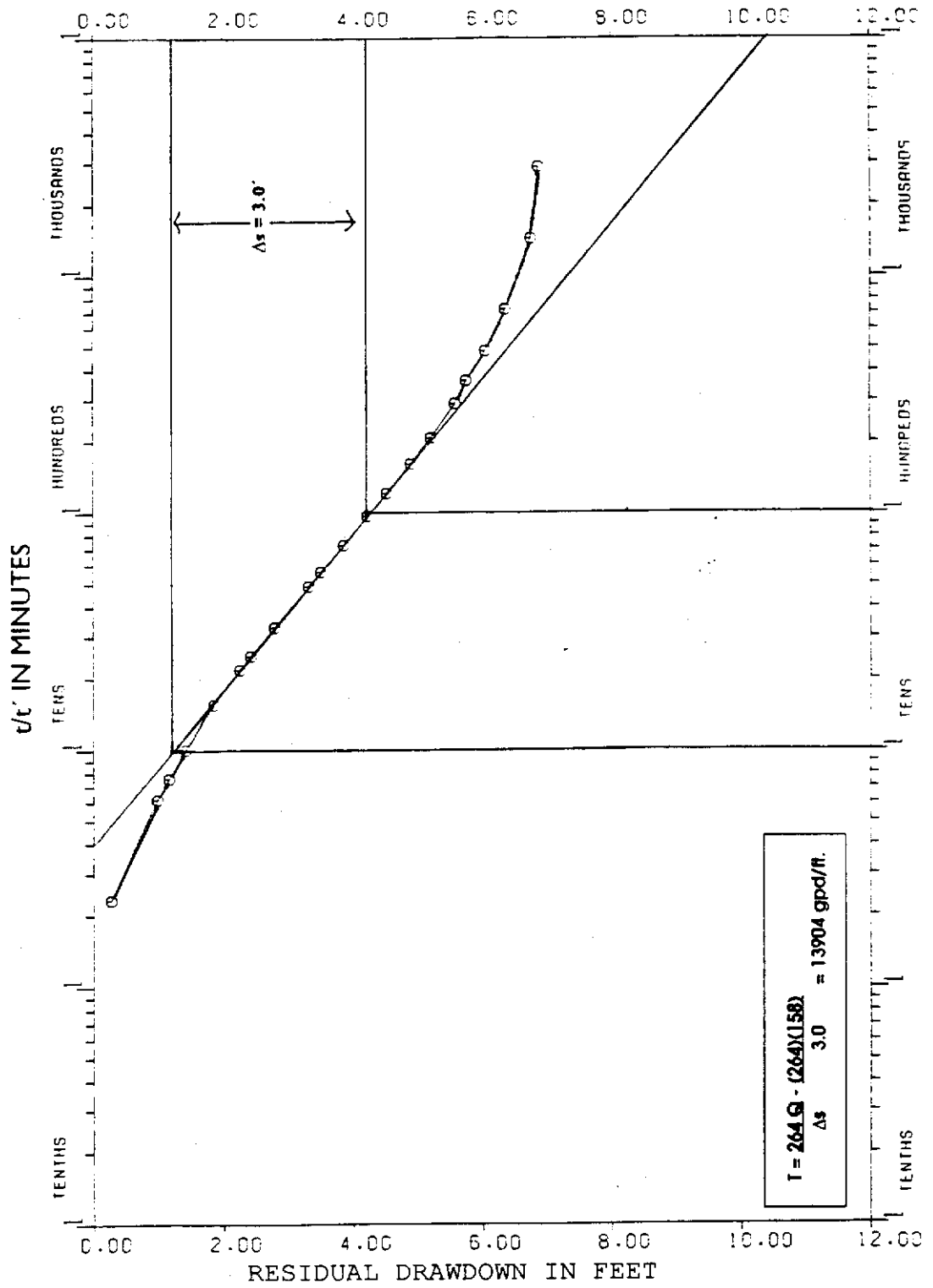
GRAPH 50. Ft. Pierce Interchange APT Recovery: Observation Well 200W
