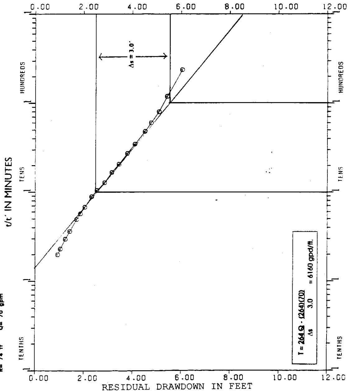
GRAPH 56. Savage Road APT Recovery: Observation Well 74S
