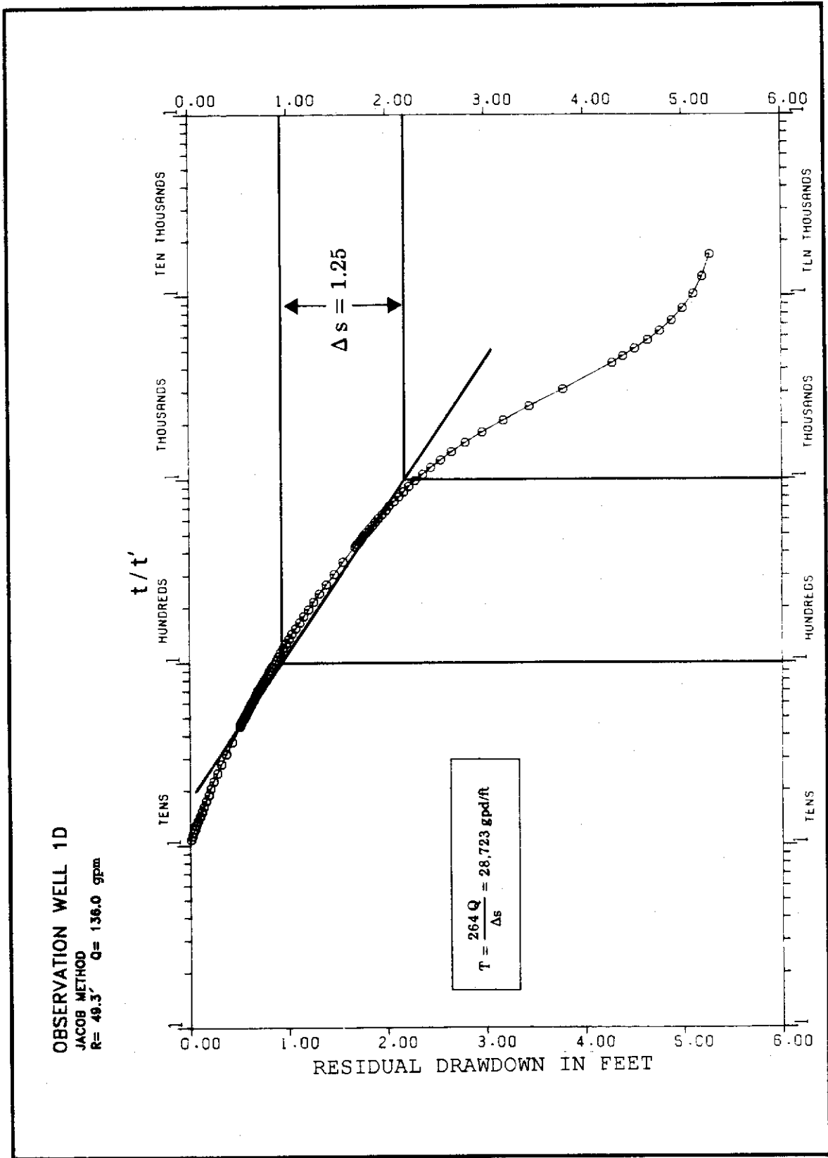
GRAPH 19. Monreve Ranch APT Recovery: Observation Well 1D
