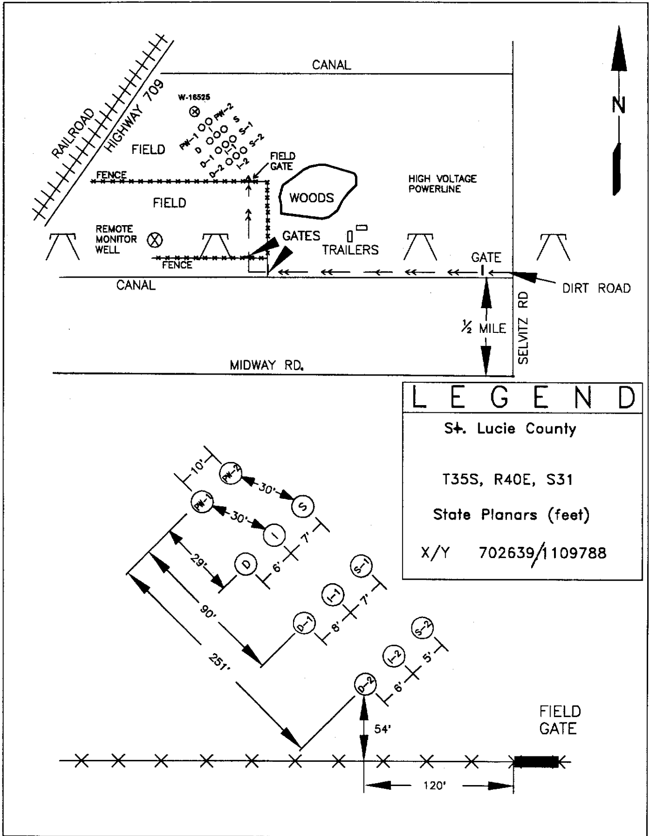
FIGURE 61. Location Map and Site Layout - STL-APT 1 Site
