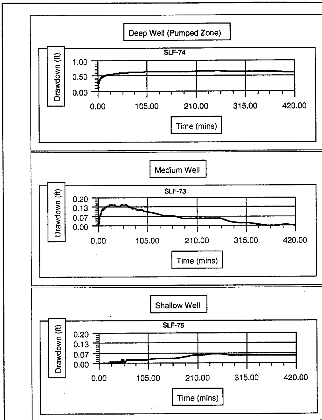
FIGURE 74. Water-Level Drawdowns in three Floridan Aquifer System Zones (Wells SLF-73, SLF-74 and SLF-75) while Pumping the Deep Zone (SLF-74)
