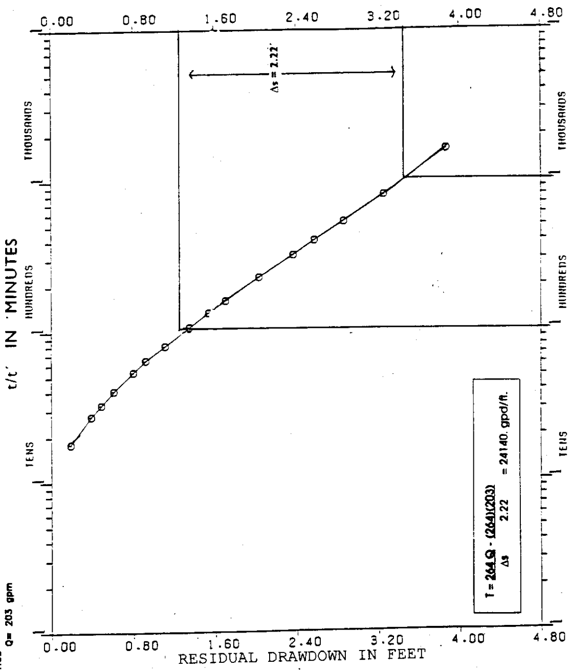
GRAPH 52. Indrio Road APT Recovery: Observation Well 150S
