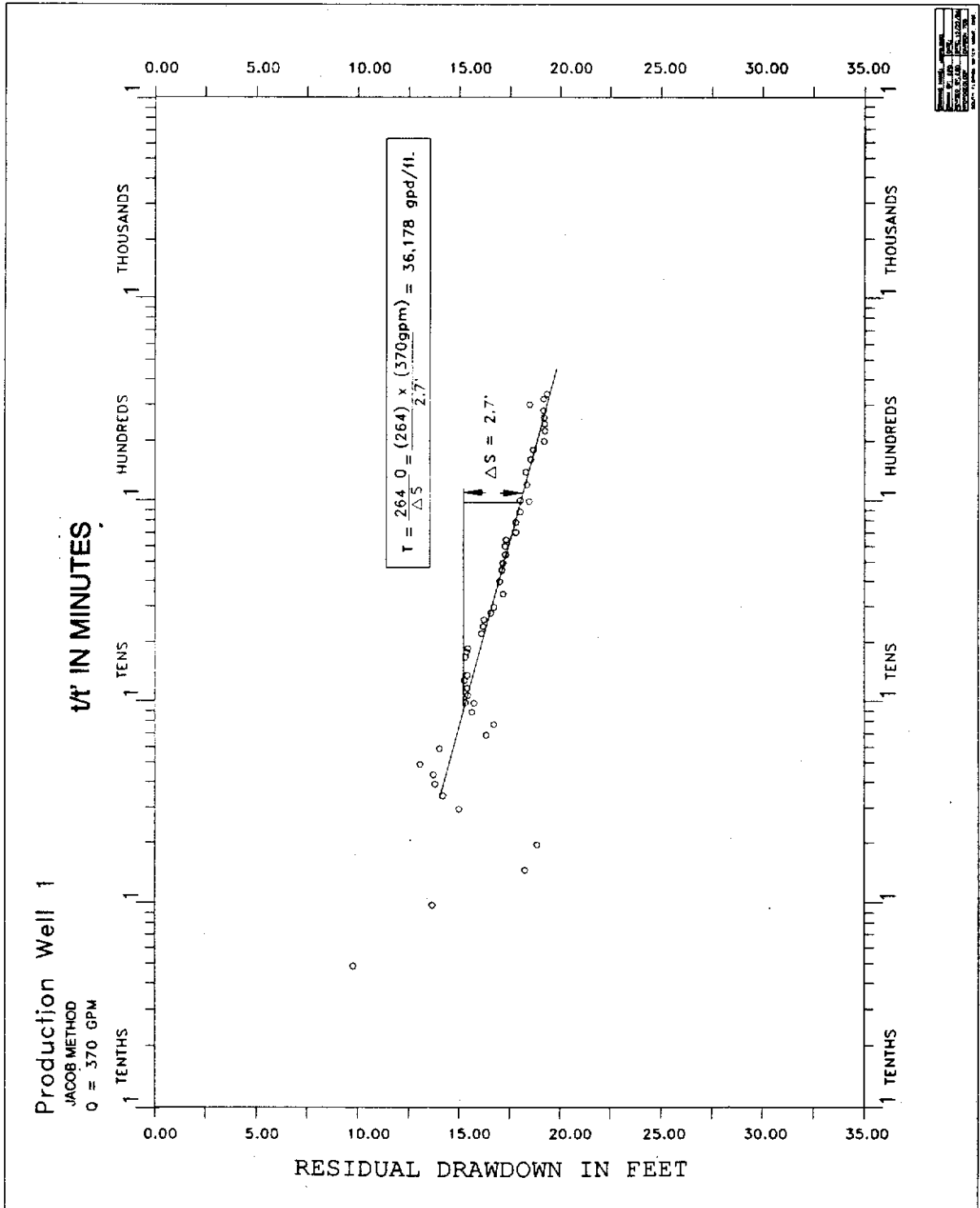
GRAPH 63. Harbor Ridge APT Drawdown: Production Well 1
