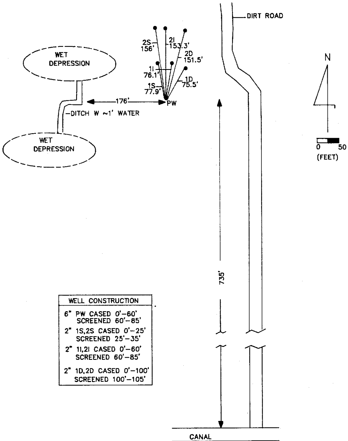
FIGURE 49. Site Layout and Well Construction Details-Mobil (TP&J) APT Site
