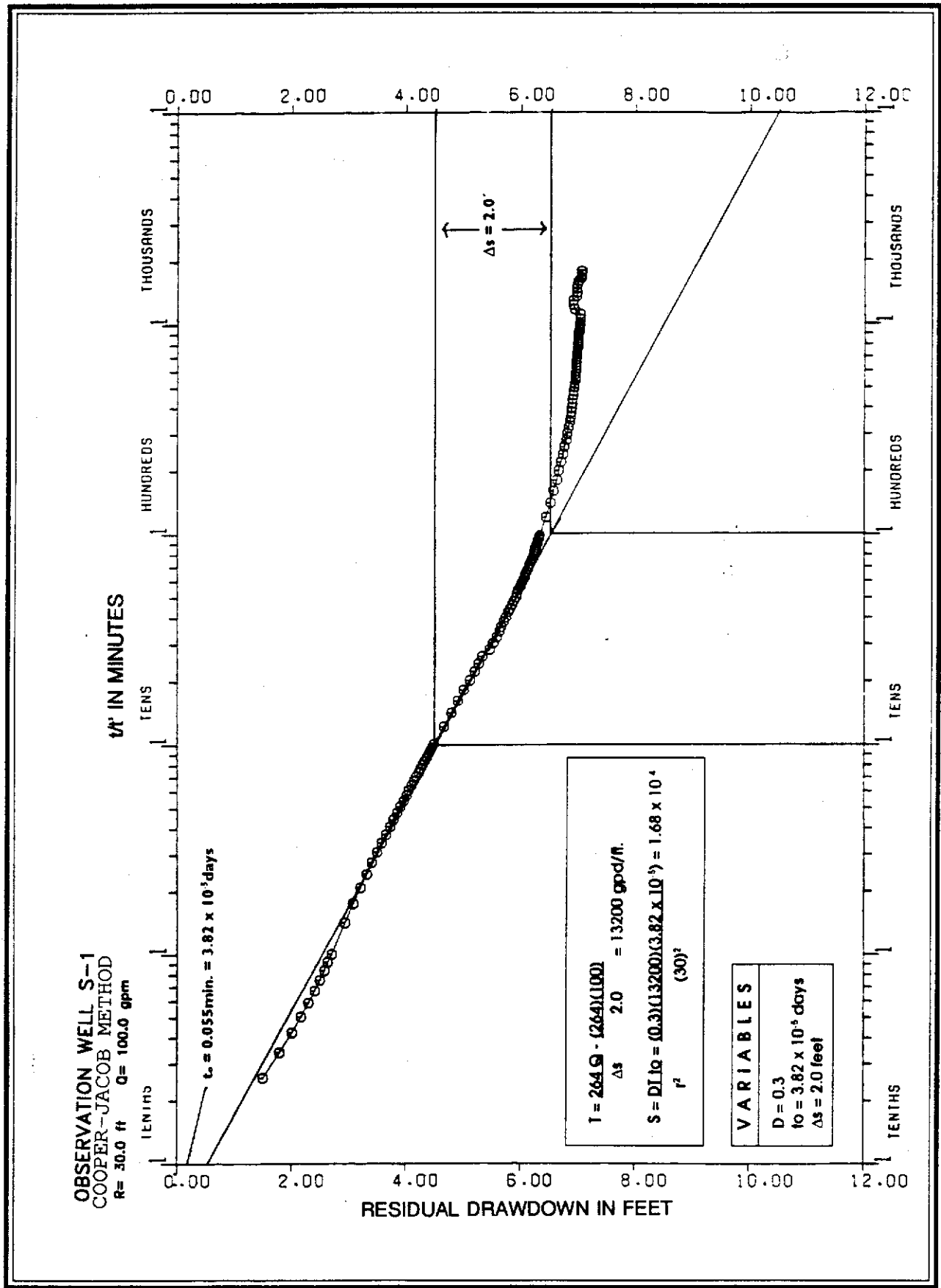
GRAPH 39. STLAPT 4 APT Drawdown: Observation Well S-1
