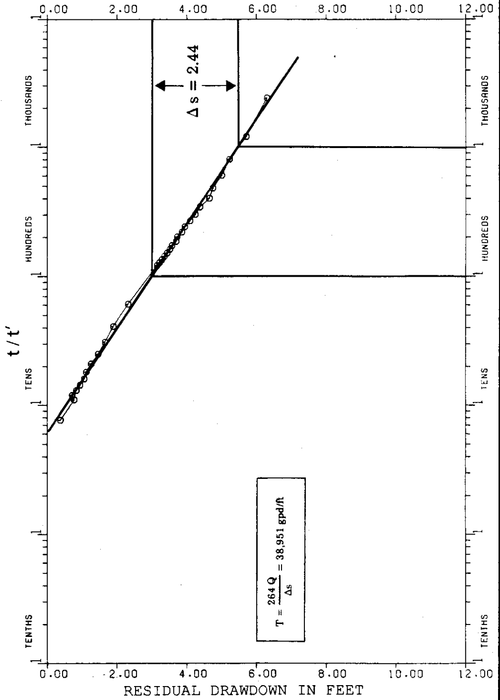
GRAPH 9. State Road 76 APT Recovery: Observation Well 1D
