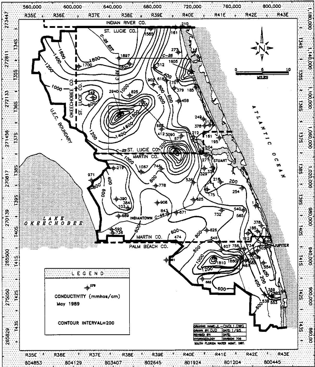
FIGURE 11. Distribution of Specific Conductivity Values in the Surficial Aquifer System Sand/Soil Zone.
