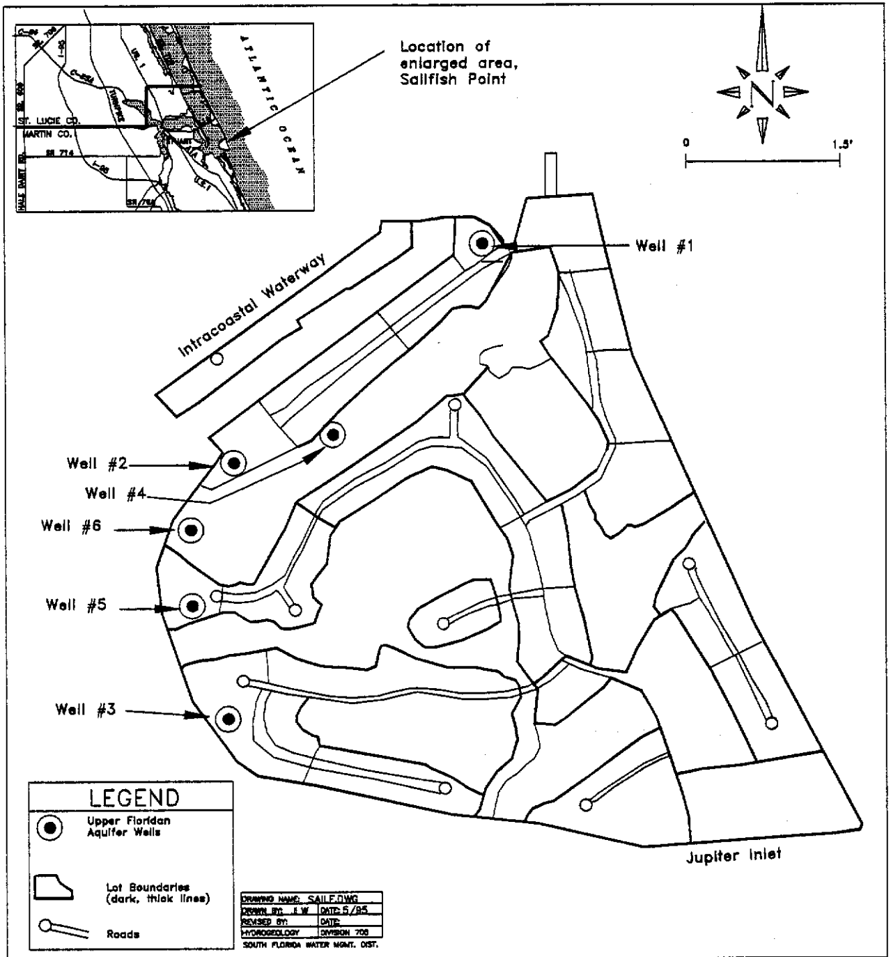
FIGURE 42. Upper Floridan Aquifer Well Locations on Sailfish Point.
