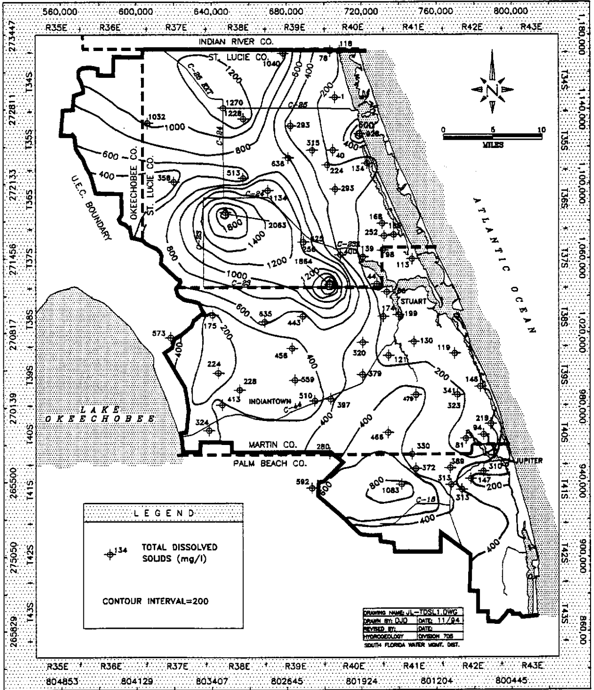
FIGURE 9. Distribution of Total Dissolved Solids Concentrations in the Surficial Aquifer System Sand/Soil Zone.
