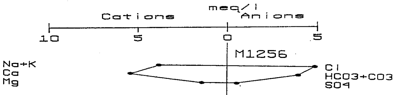
FIGURE 6. Stiff Diagram.
