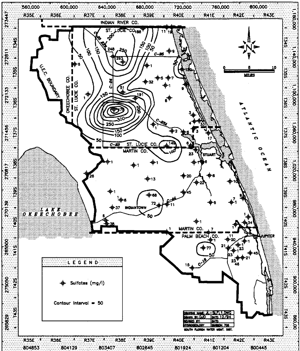
FIGURE 12. Distribution of Dissolved Sulfate Concentrations in the Surficial Aquifer System Sand/Soil Zone.
