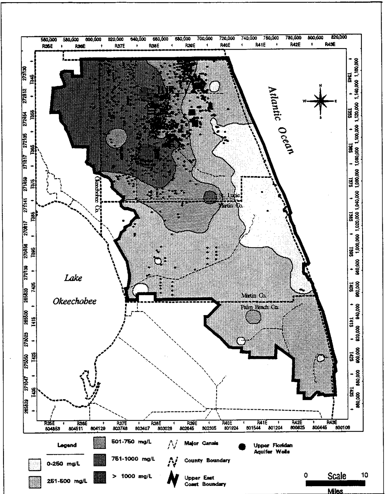
FIGURE 10. Total Dissolved Solids Concentrations in the Surficial Aquifer System Sand/Soil Zone and Permitted Upper Floridan Aquifer Well Locations.
