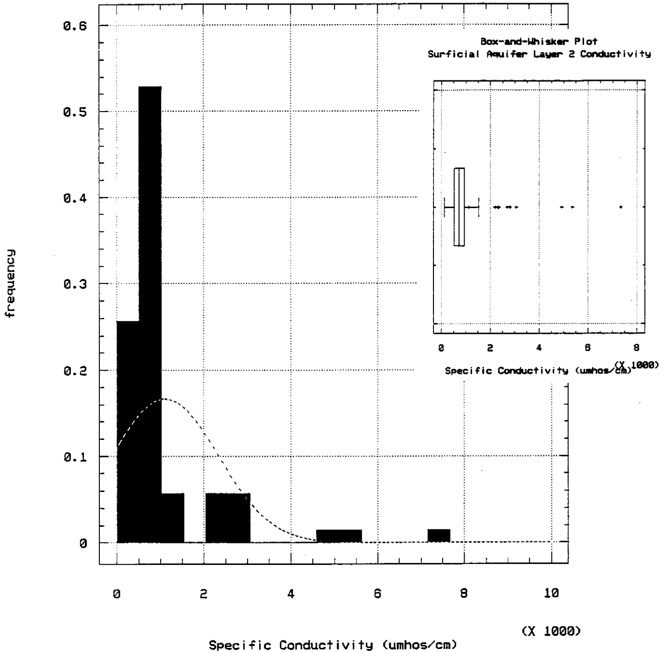
FIGURE B-7. Frequency Histogram and Box and Whisker Plot Showing Specific Conductivity Sample Variance from the SFWMD's Network of Wells Completed to the Production Zone (Surficial Aquifer System)
