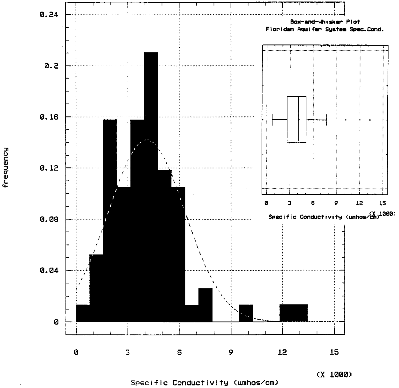
FIGURE B-11. Frequency Histogram and Box and Whisker Plot Showing Specific Conductivity Sample Variance from the SFWMD's Network of Wells Completed to the Upper Floridan Aquifer
