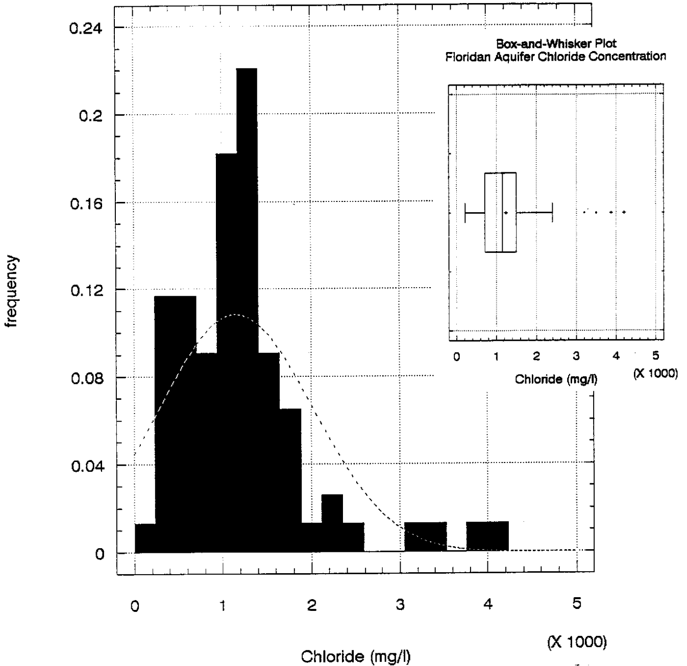
FIGURE B-9. Frequency Histogram and Box and Whisker Plot Showing Chloride Concentration Sample Variance from the SFWMD's Network of Wells Completed to the Upper Floridan Aquifer
