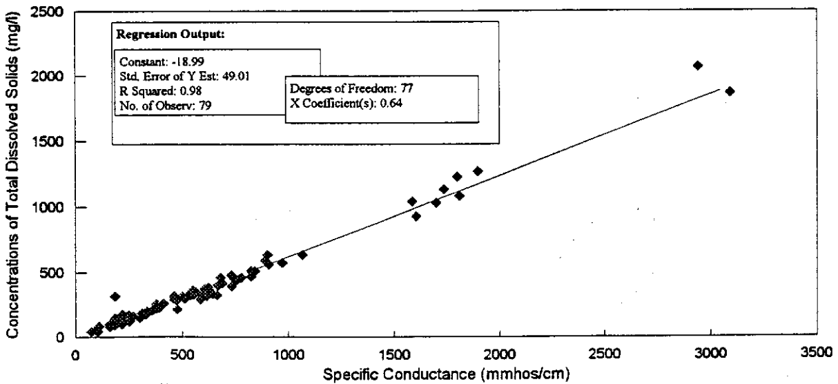
FIGURE 15. Linear Regression of Specific Conductivity and Total Dissolved Solids Concentrations in the Surficial Aquifer System Sand/Soil Zone.
