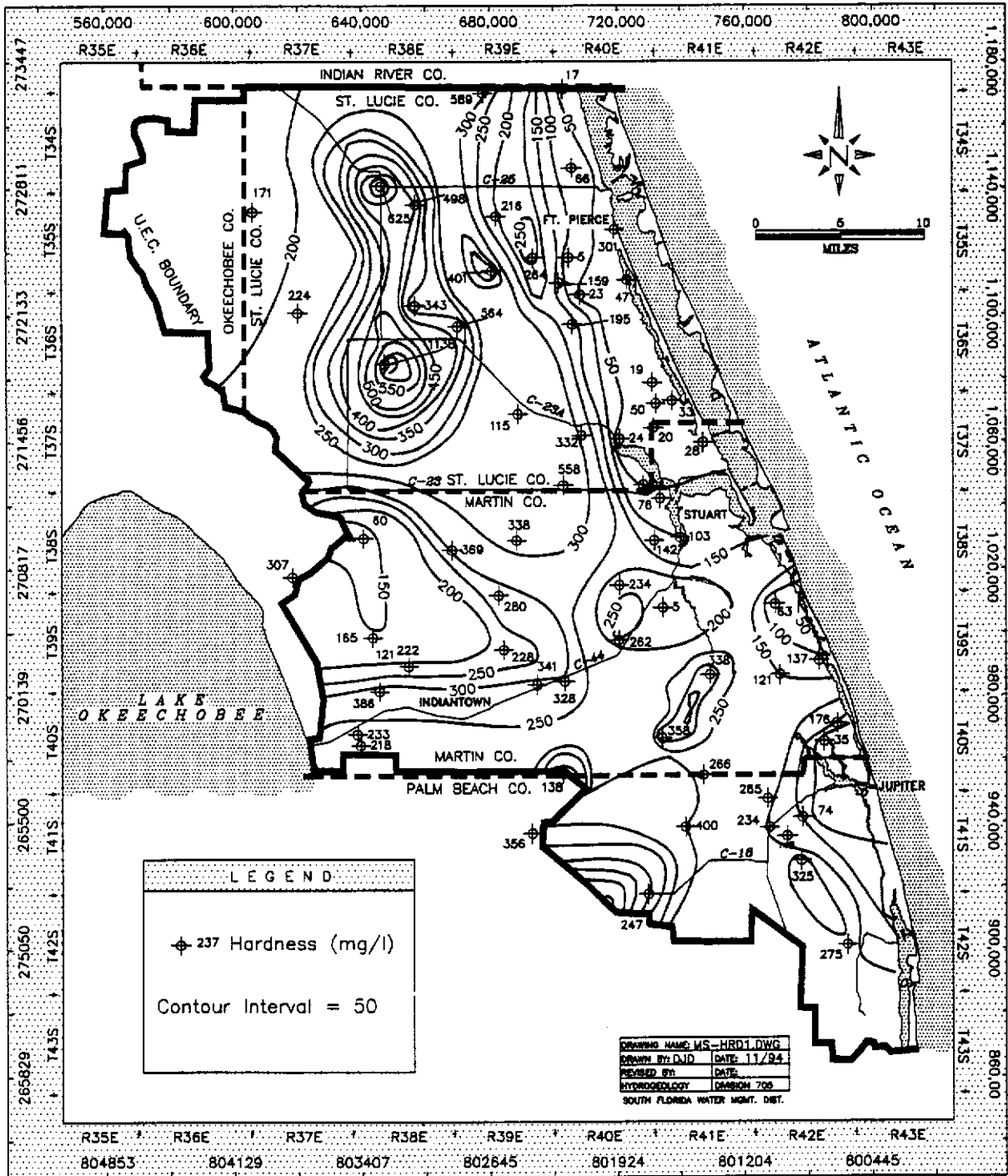
FIGURE 13. Distribution of Hardness (CaCO 3 ) in the Surficial Aquifer System Sand/Soil Zone.
