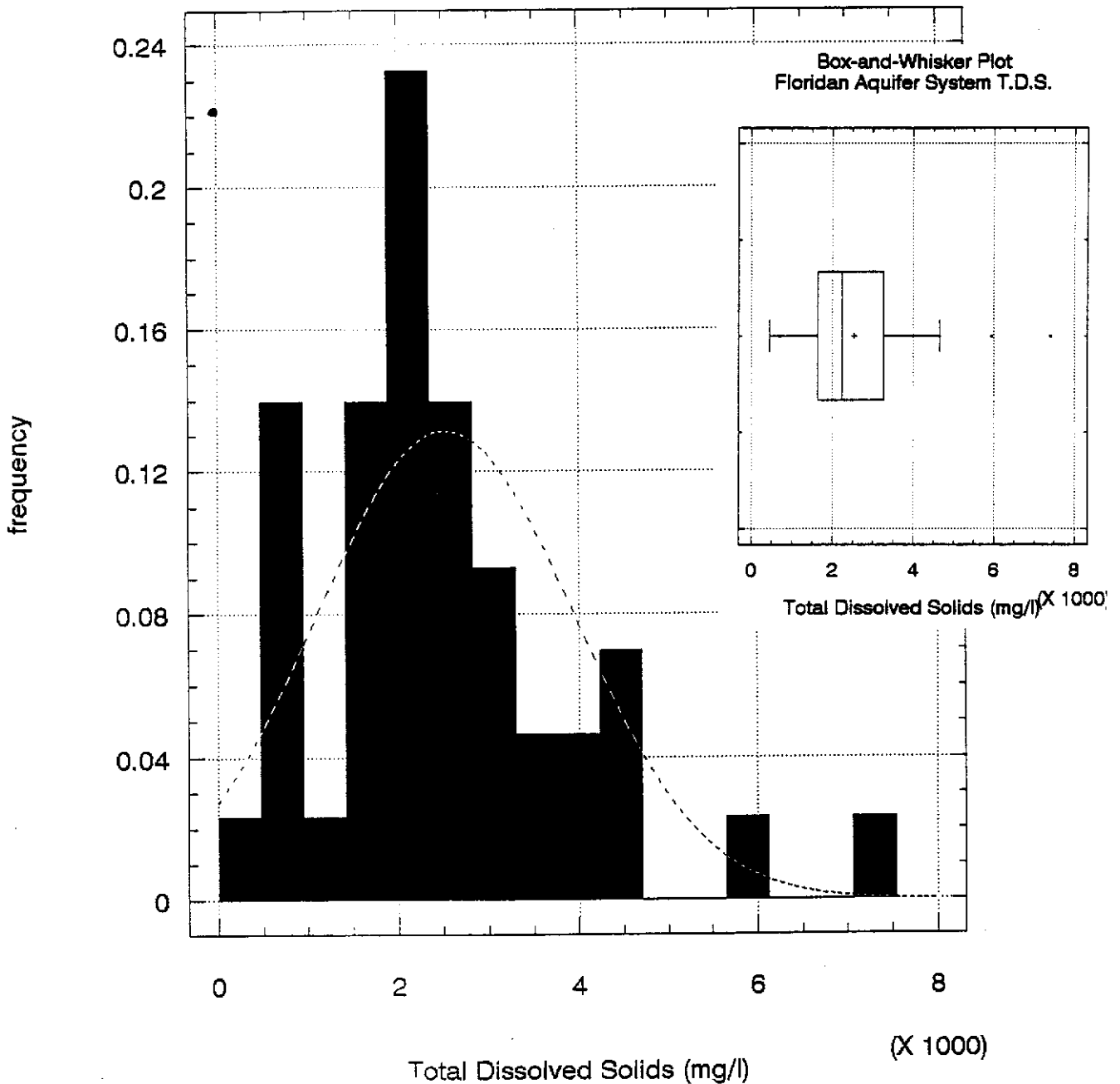
FIGURE B-10. Frequency Histogram and Box and Whisker Plot Showing Total Dissolved Solids Concentration Sample Variance from the SFWMD's Network of Wells Completed to the Upper Floridan Aquifer
