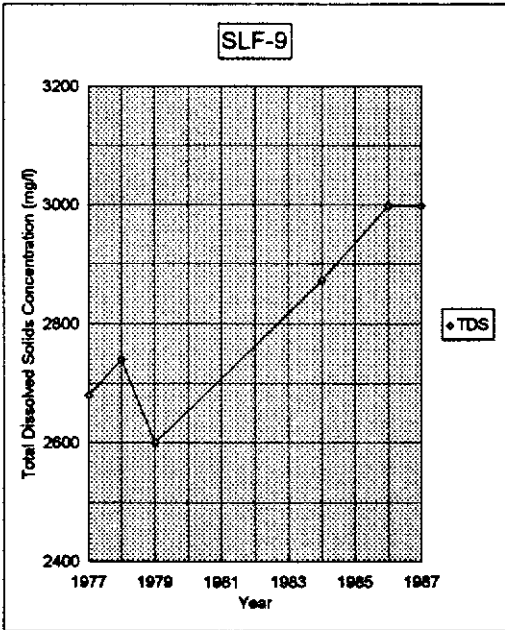
FIGURE 39. Total Dissolved Solids Concentration Variations over Time From Four Agricultural Monitor Wells Completed in the Upper Floridan Aquifer.
