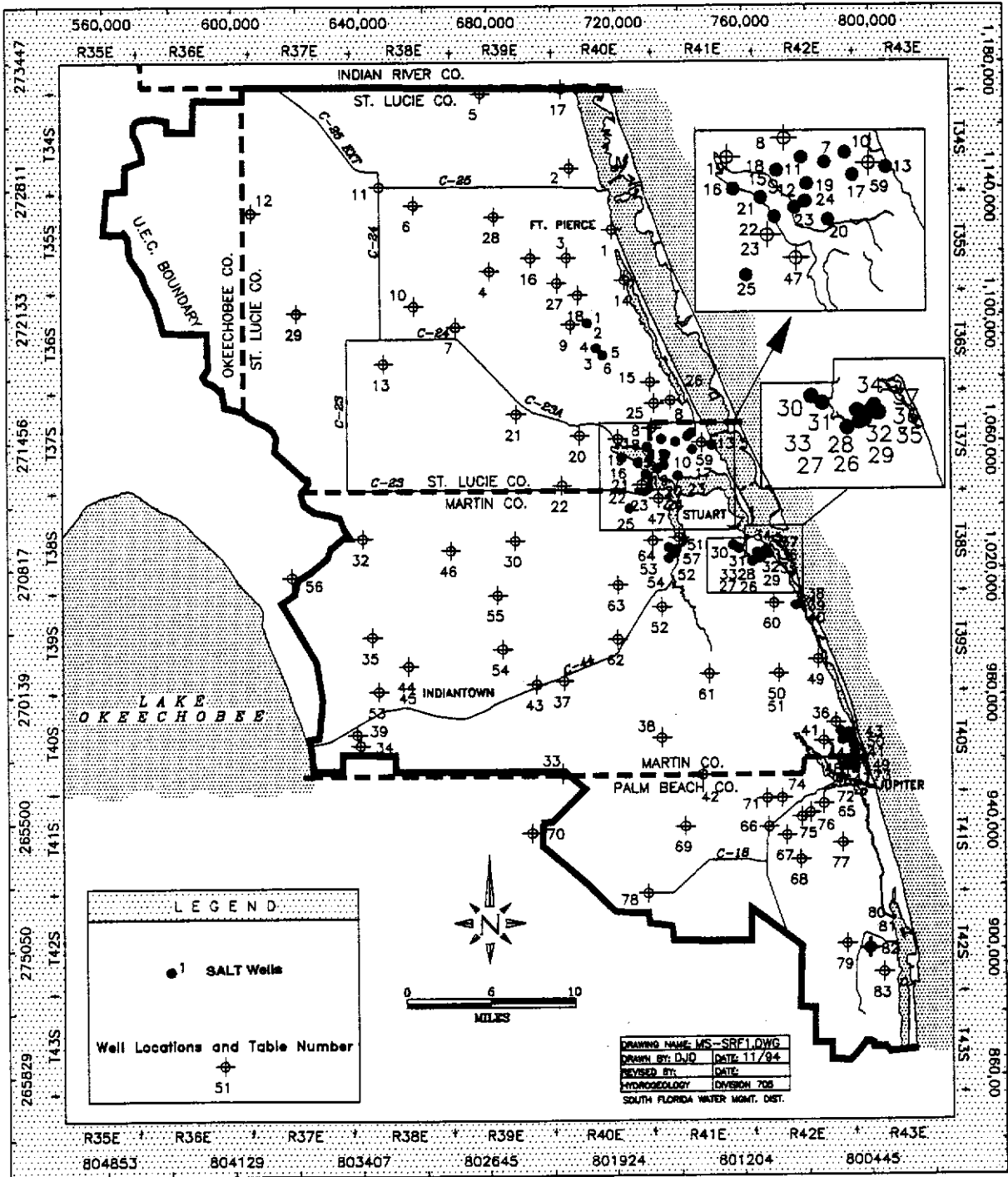
FIGURE 7. Location of Wells Completed in the Sand/Soil Zone (Layer 1).
