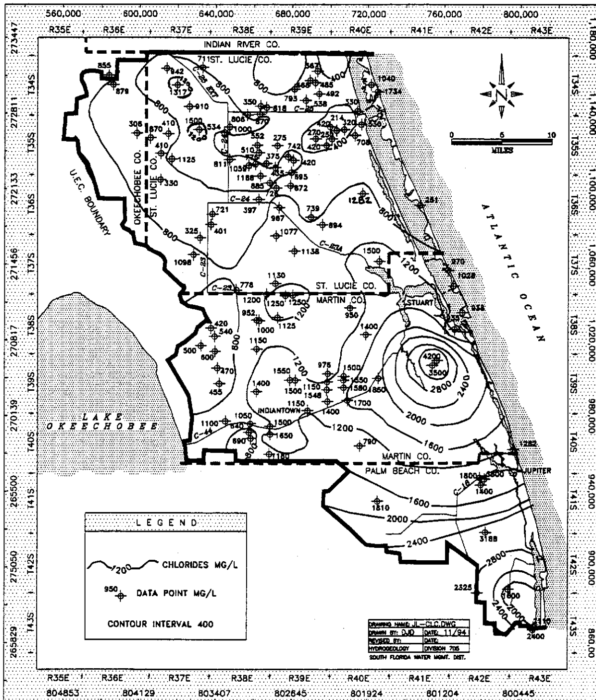
FIGURE 28. Distribution of Chloride Concentrations in the Upper Floridan Aquifer.
