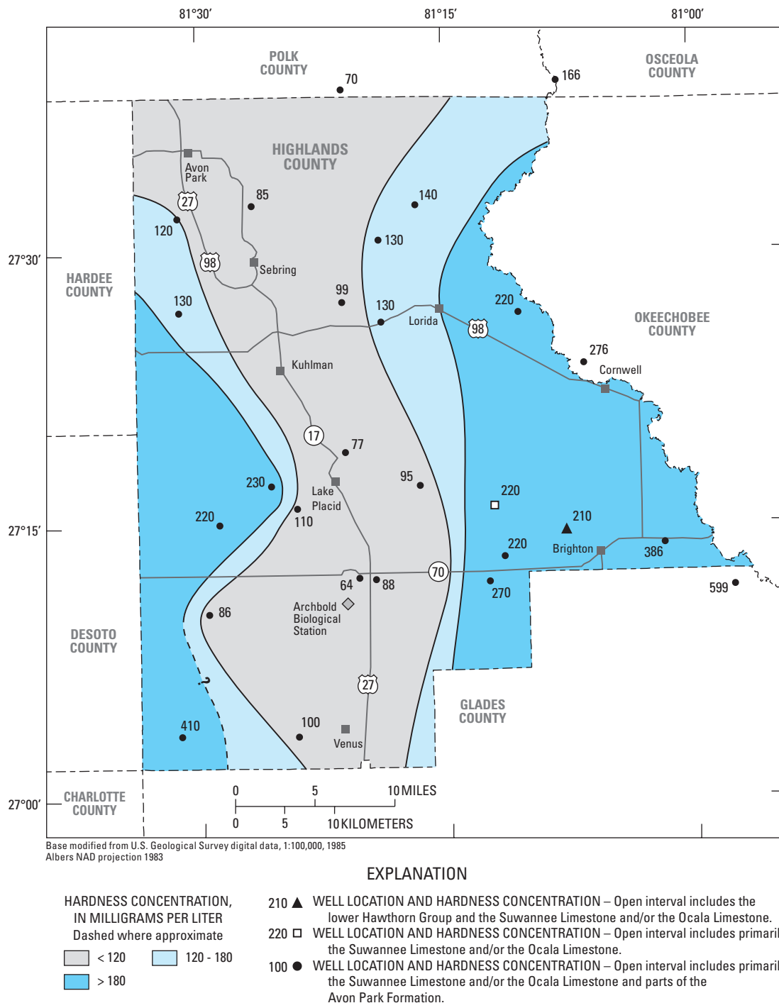
Figure 48. Generalized distribution of hardness concentrations in water from the Upper Floridan aquifer.
