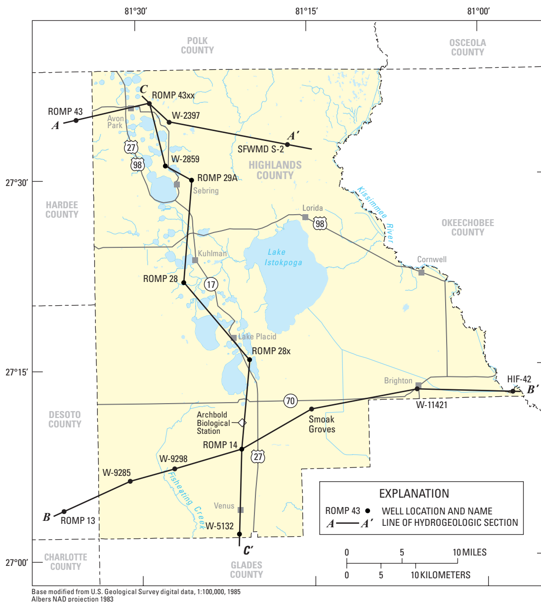
Figure 15. Location of hydrogeologic sections.
