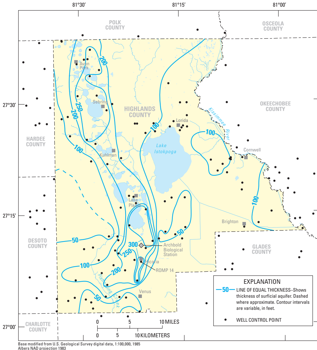
Figure 18. Generalized thickness of the surficial aquifer.
