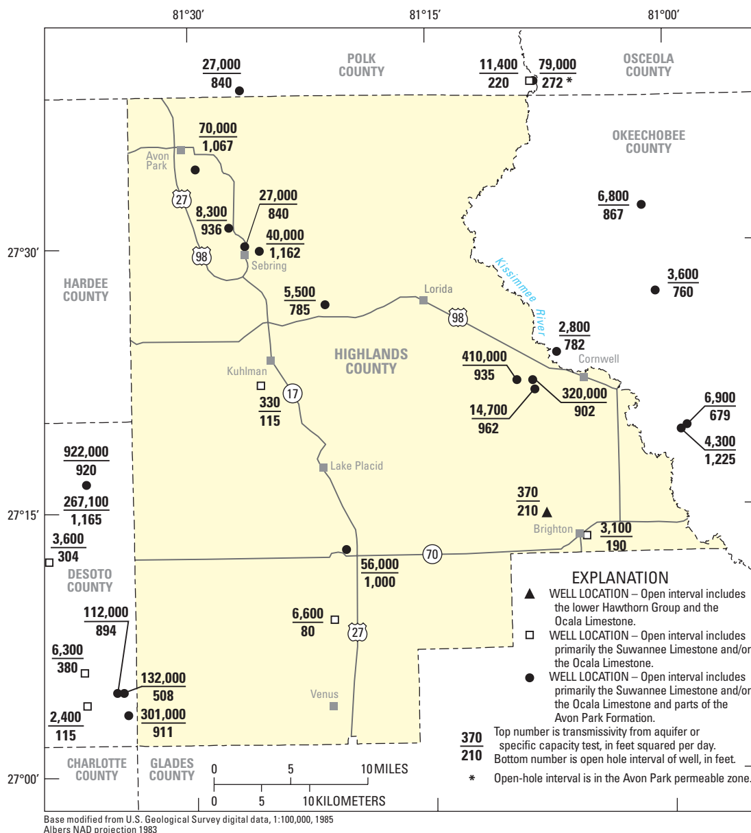
Figure 25. Transmissivity of the Upper Floridan aquifer. From Shaw and Trost (1984), Bradner (1994), Clayton (1998), DeWitt (1998), Baldini and Rappuhn (1999), Southwest Florida Water Management District (2000), and Mallams and Lee (2005).
