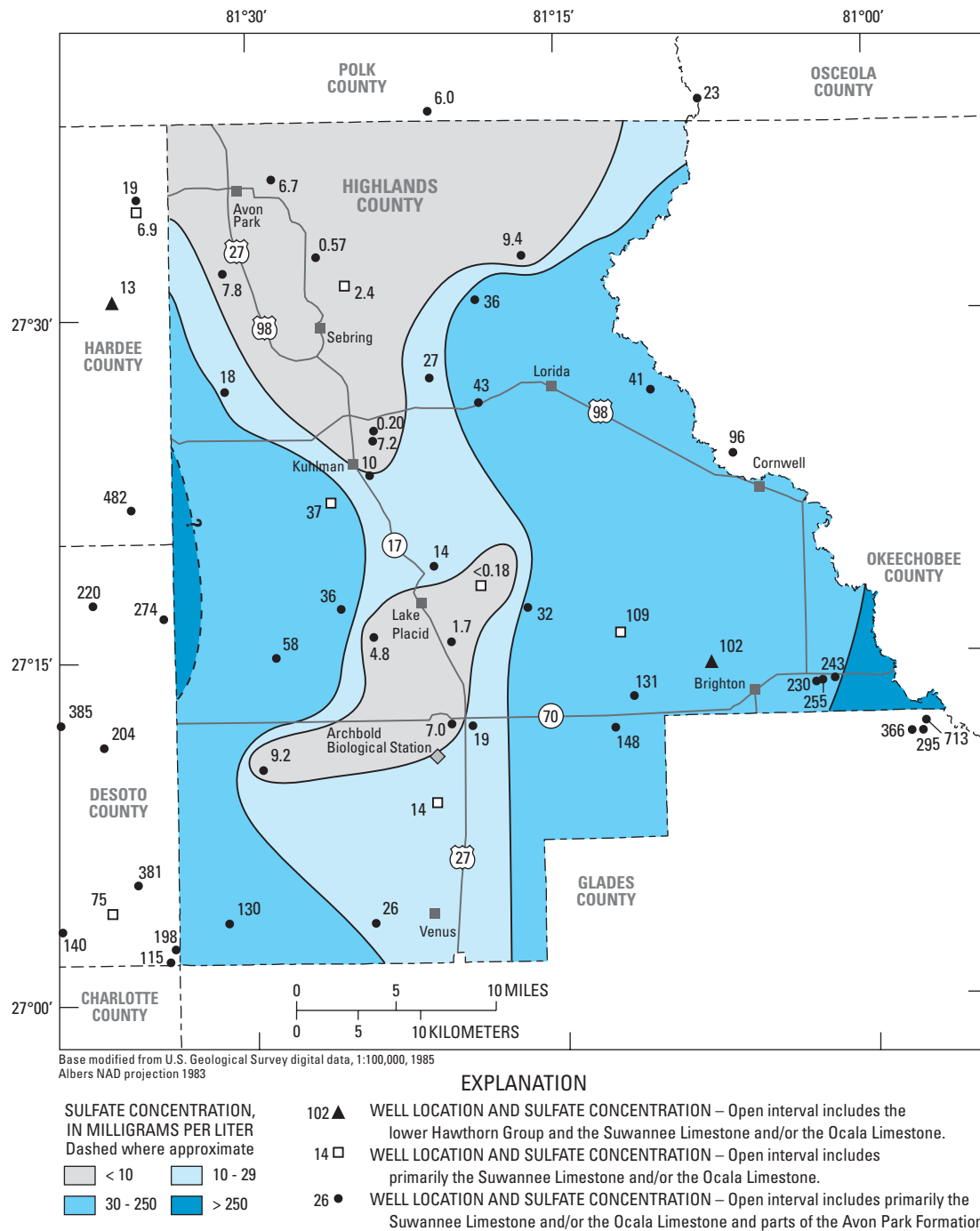
Figure 46. Generalized distribution of sulfate concentrations in water from the Upper Floridan aquifer.
