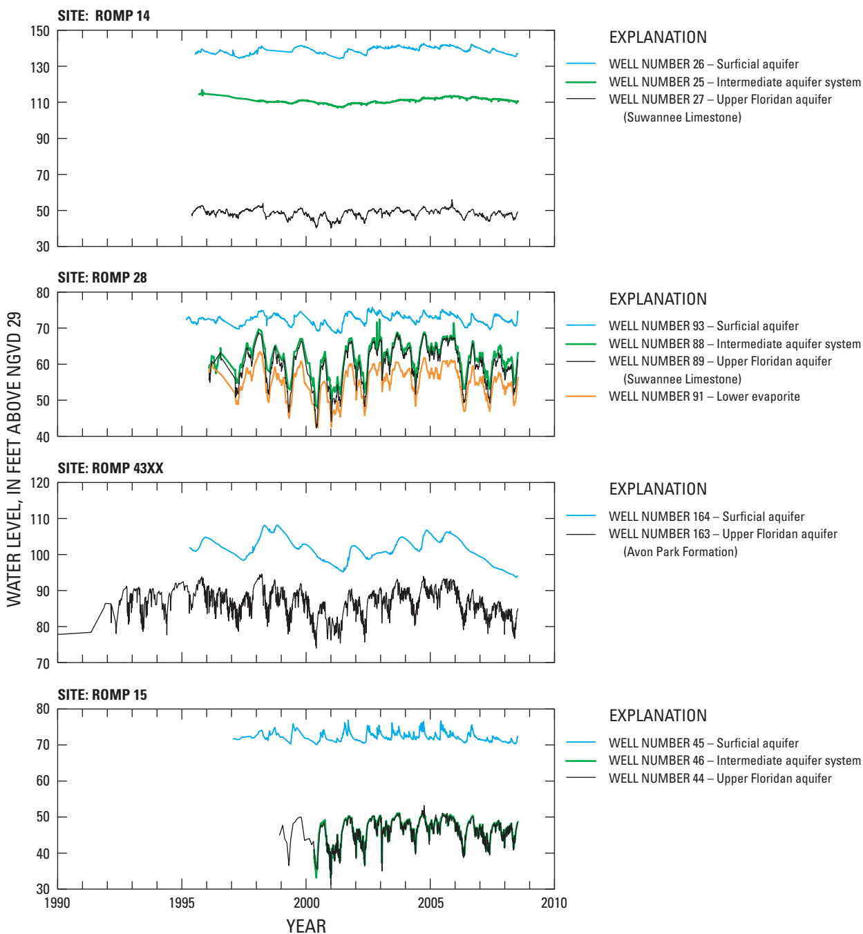
Figure 30. Water levels in selected wells open to the surficial aquifer, intermediate aquifer system, and Upper Floridan aquifer. Well locations shown in figures 1 and 11.
