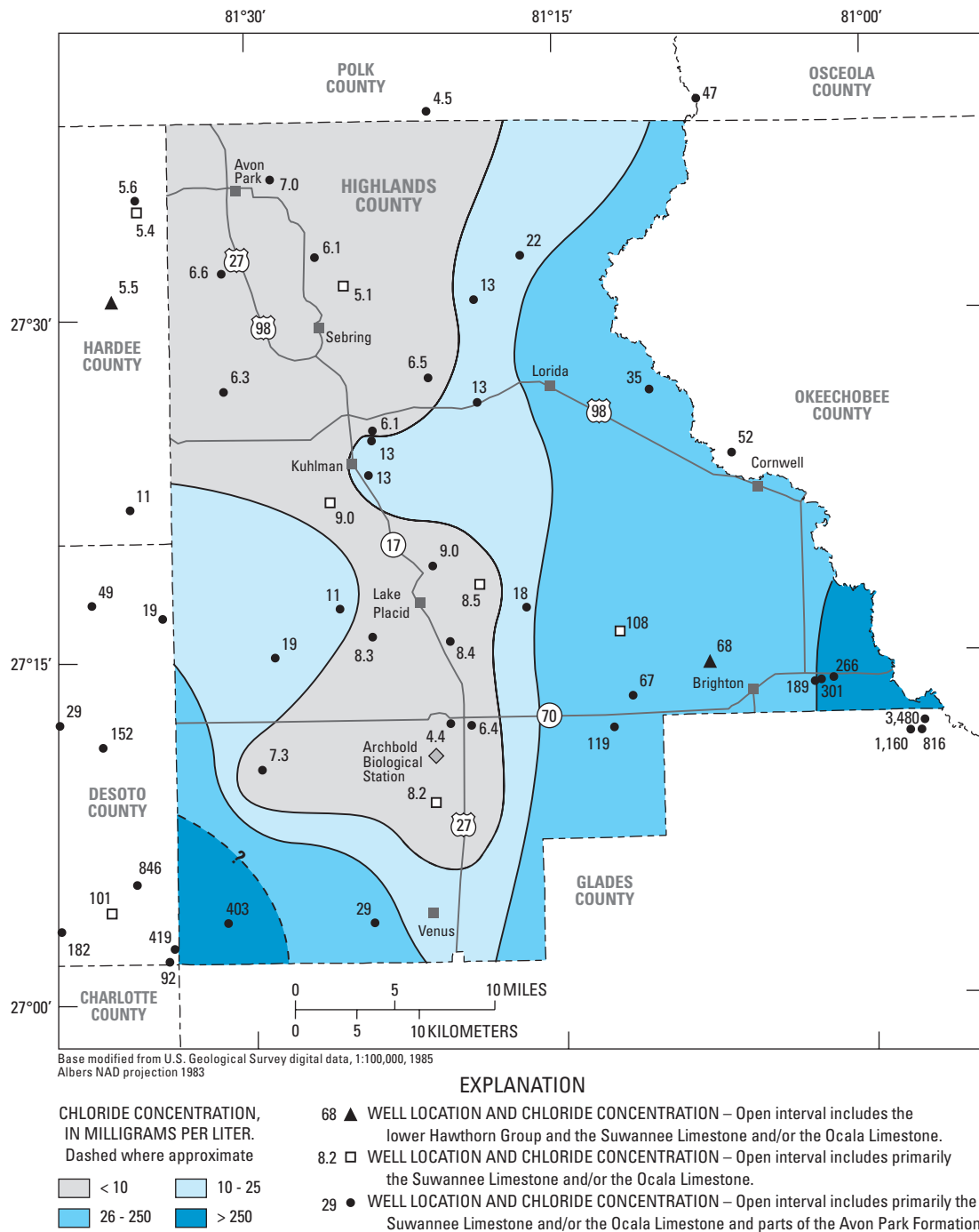
Figure 45. Generalized distribution of chloride concentrations in water from the Upper Floridan aquifer.
