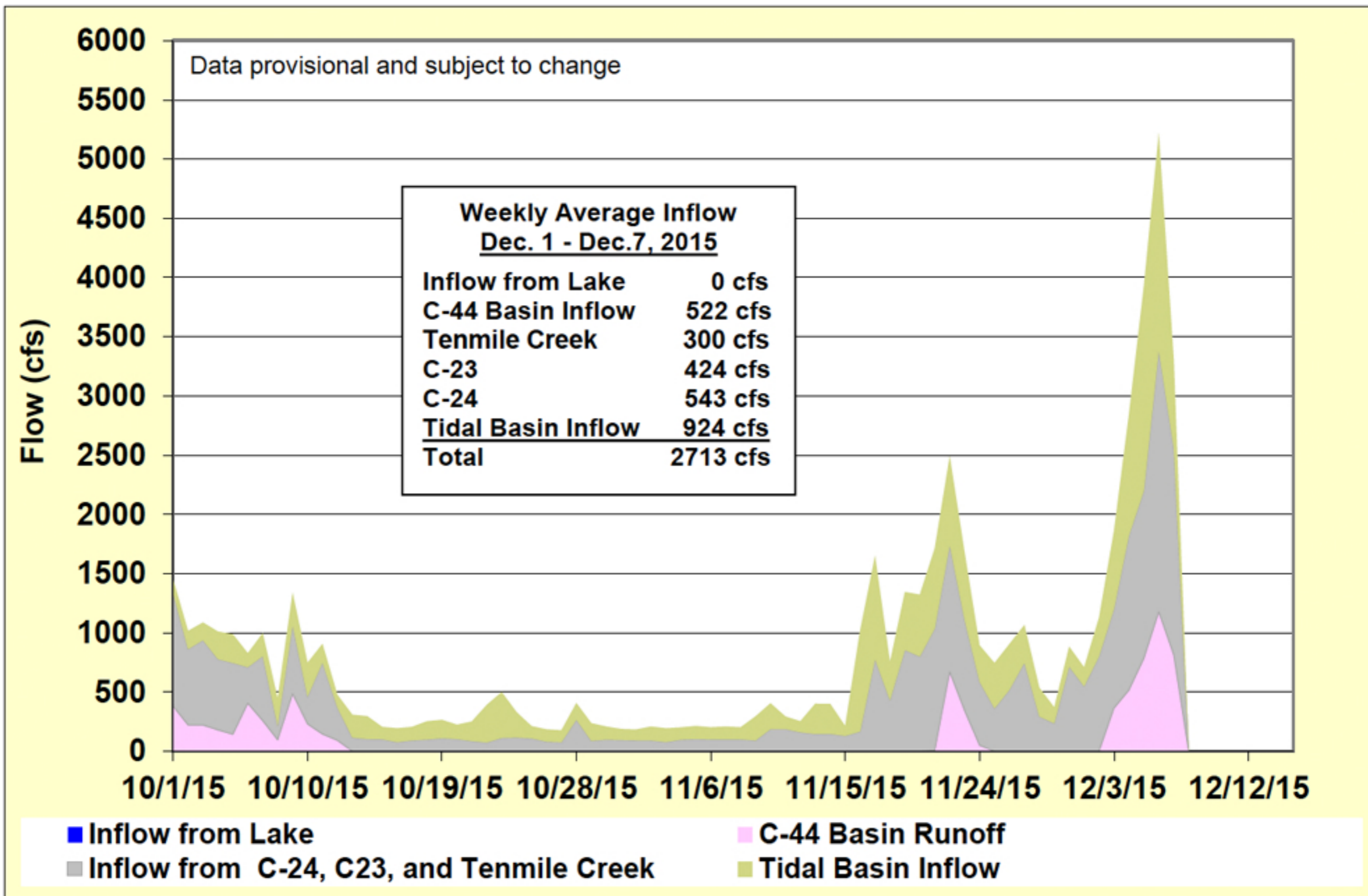
Figure 2. Estimated surface freshwater inflows from Lake Okeechobee and runoff from the C-44, C-23, C-24, Ten Mile Creek, and tidal basins into the St. Lucie Estuary.
