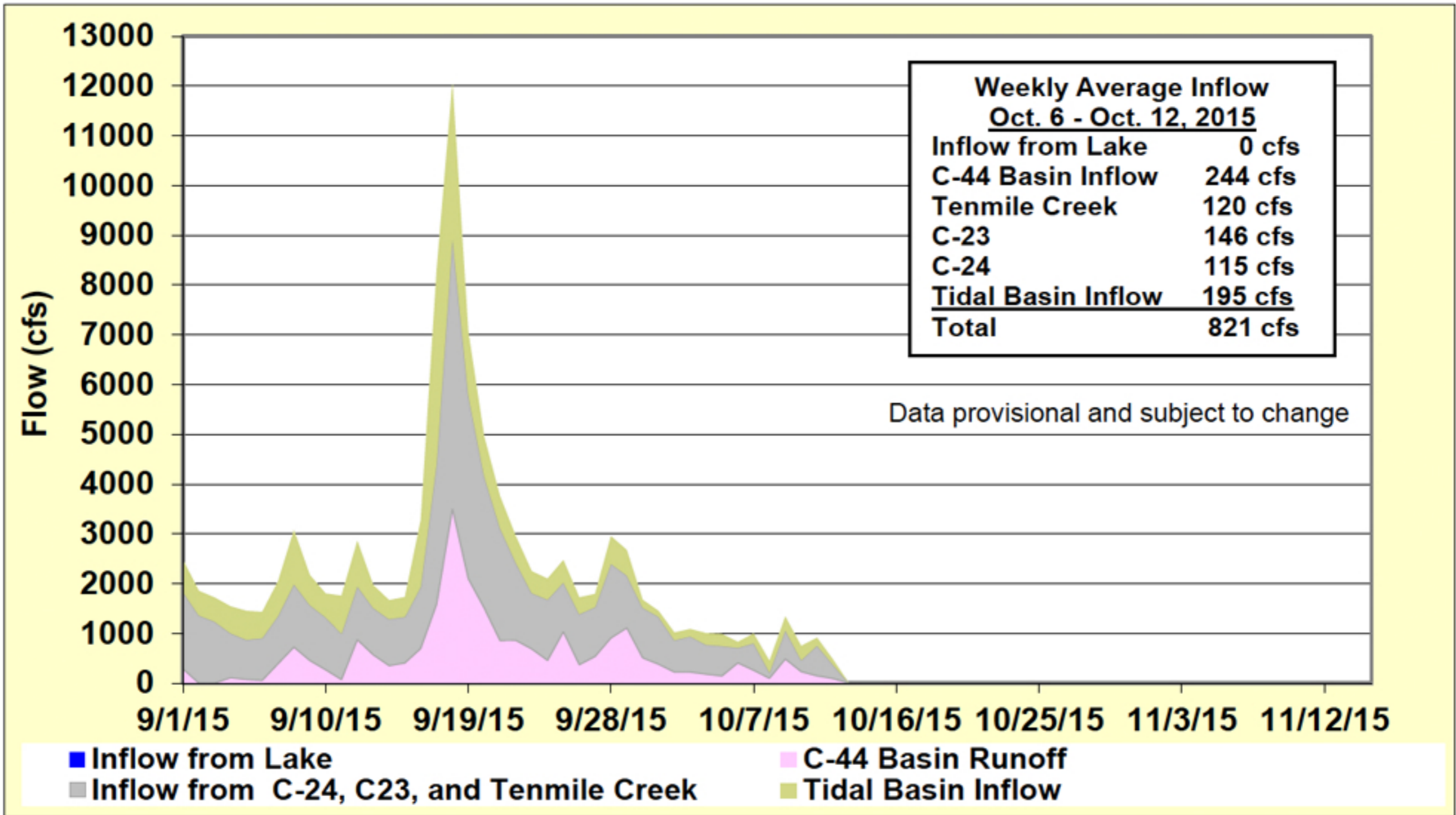
Figure 2. Estimated surface freshwater inflows from Lake Okeechobee and runoff from the C-44, C-23, C-24, Ten Mile Creek, and tidal basins into the St. Lucie Estuary.
