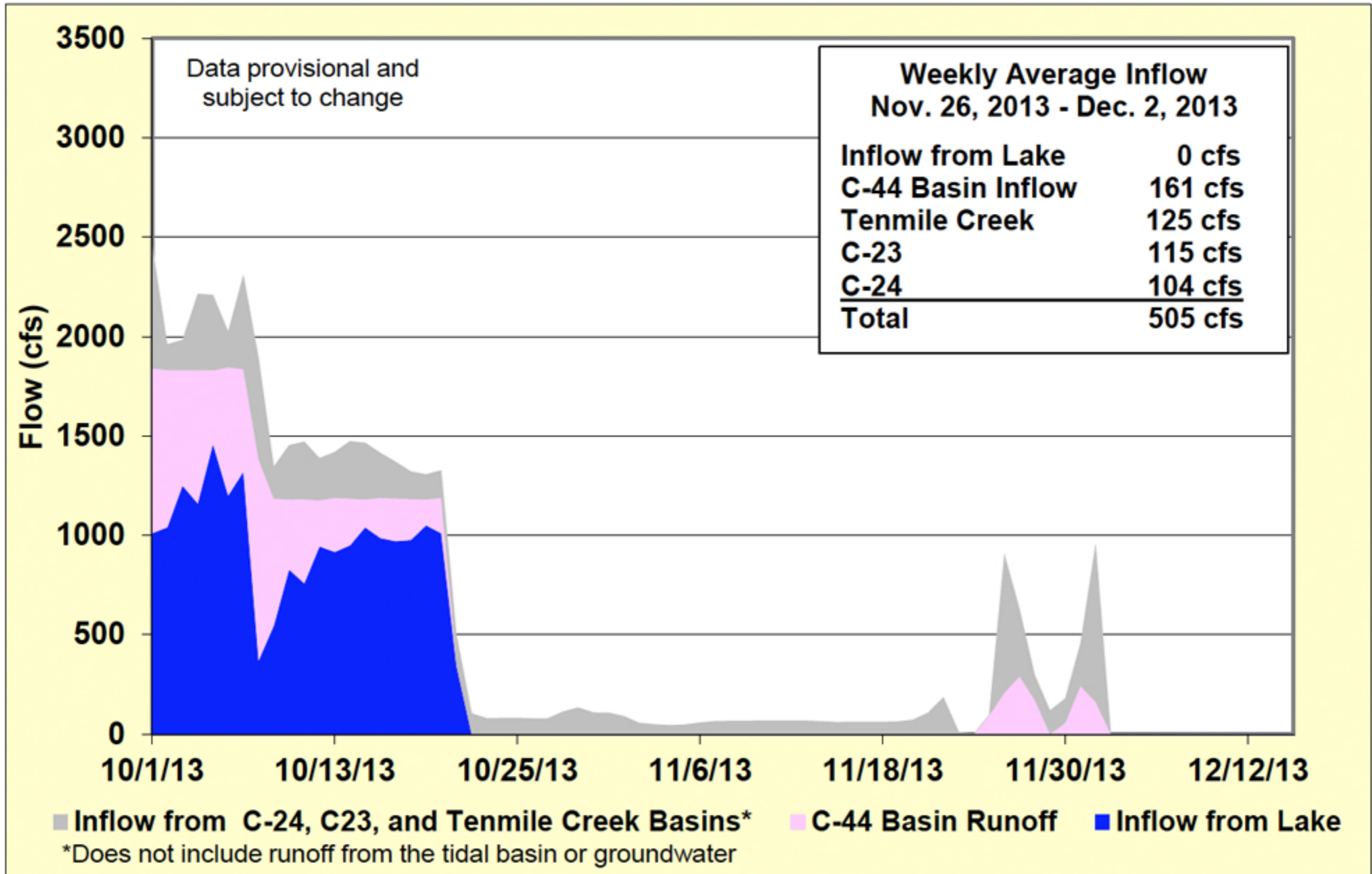
Figure 2. Estimated surface freshwater inflows from Lake Okeechobee, and runoff from the C-44, C-23, C-24 and Ten Mile Creek basins into the St. Lucie Estuary.
