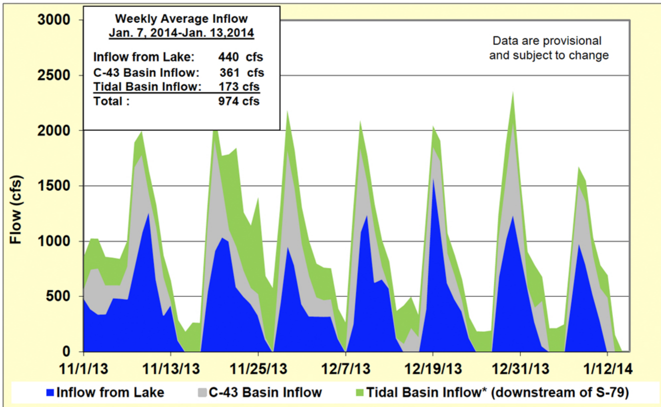
Figure 6. Surface freshwater inflows from Lake Okeechobee, runoff from the C-43 basin, and tributaries in the tidal basin into the Caloosahatchee River Estuary.
