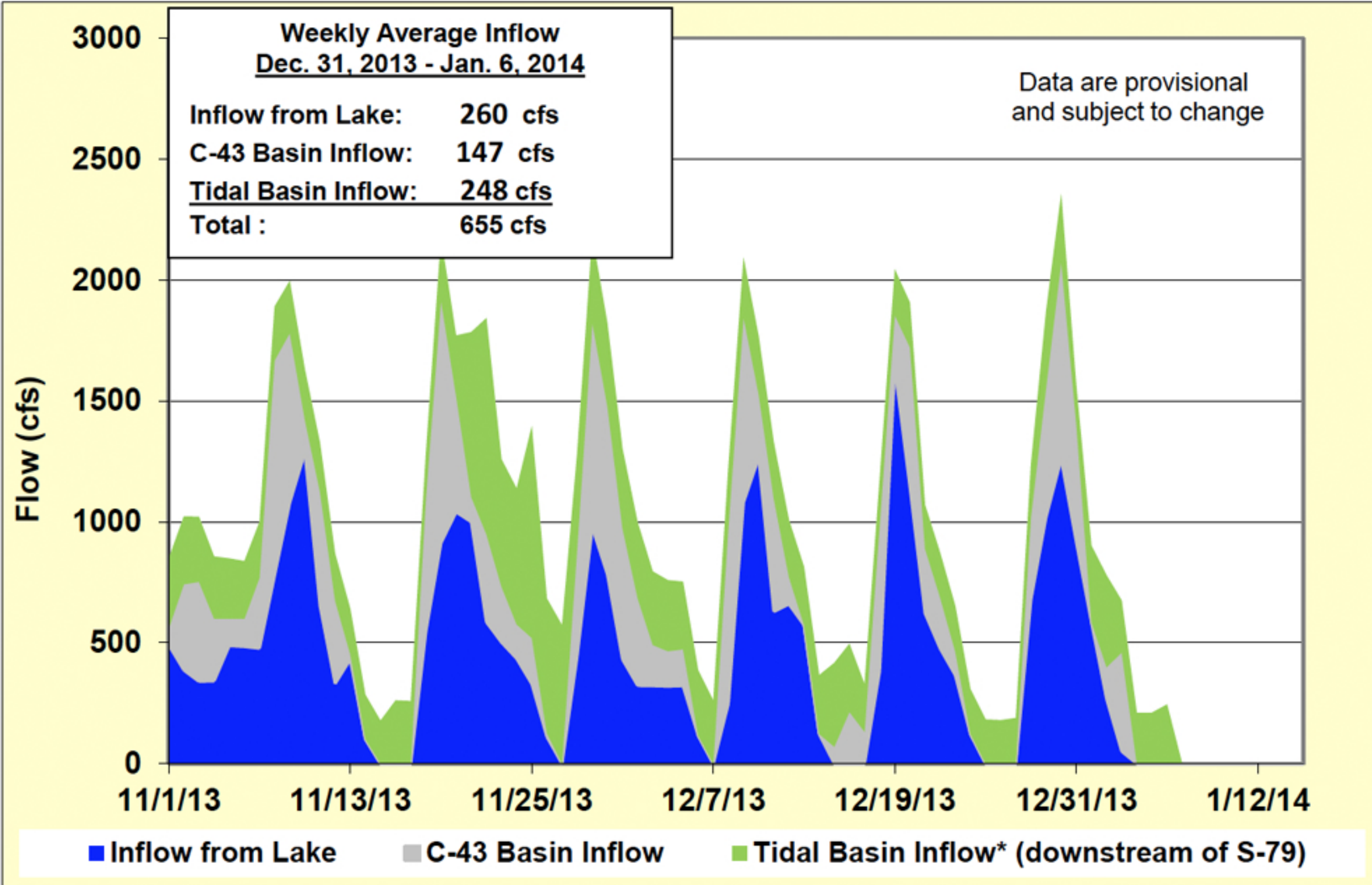
Figure 6. Surface freshwater inflows from Lake Okeechobee, runoff from the C-43 basin, and tributaries in the tidal basin into the Caloosahatchee River Estuary. *Does not include direct overland runoff from the tidal basin or groundwater.
