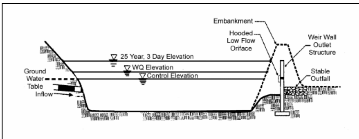
FIGURE 18 Wet detention pond design (SFWMD 2002b)
