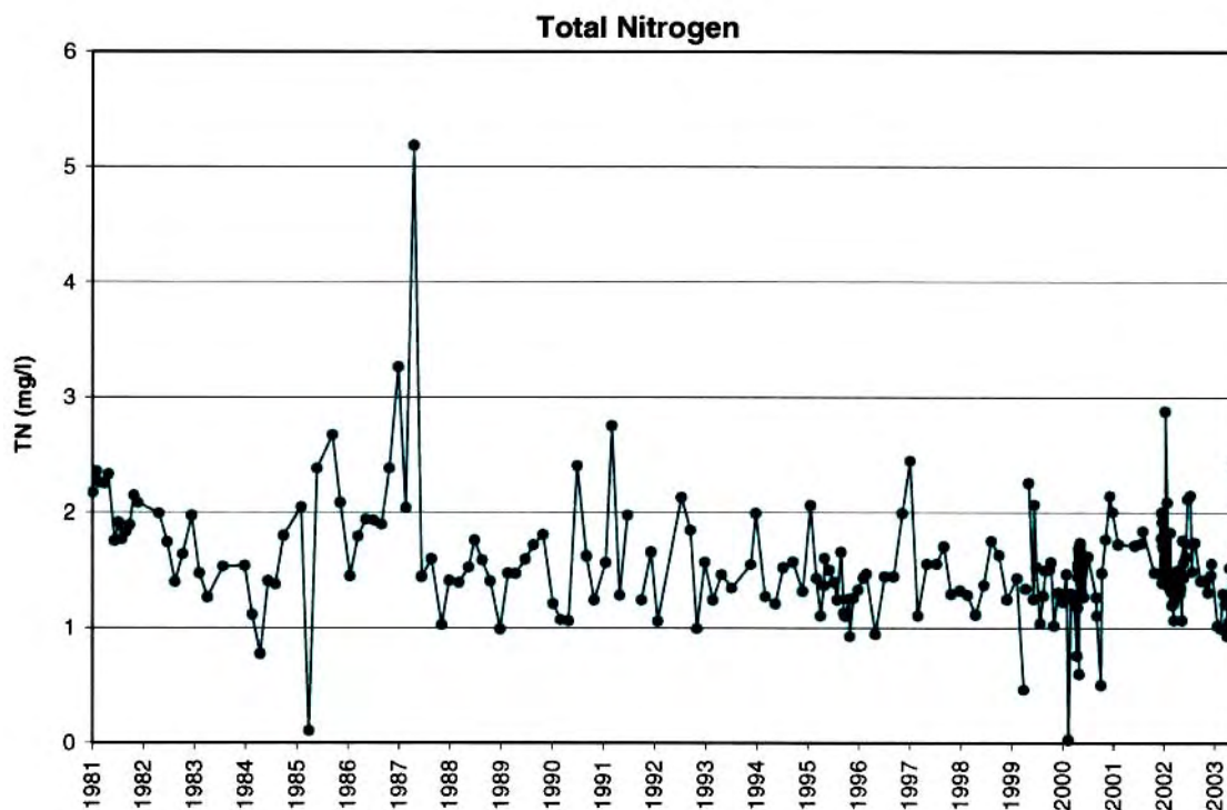
FIGURE A23 Concentration of Total Nitrogen (TN) in the freshwater discharge at S-79
