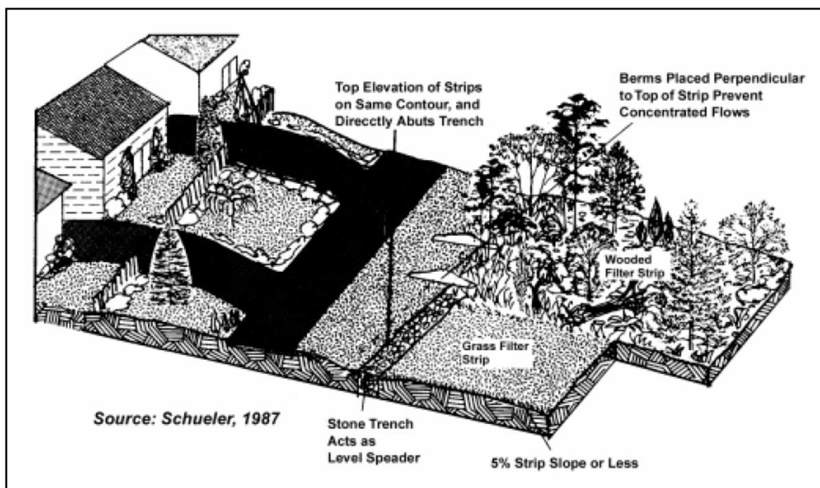
FIGURE 17 Buffer strip design (SFWMD 2002b)
