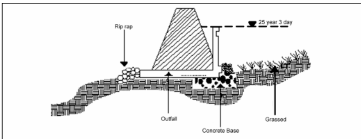
FIGURE 19 Retention basin design (SFWMD 2002b)
