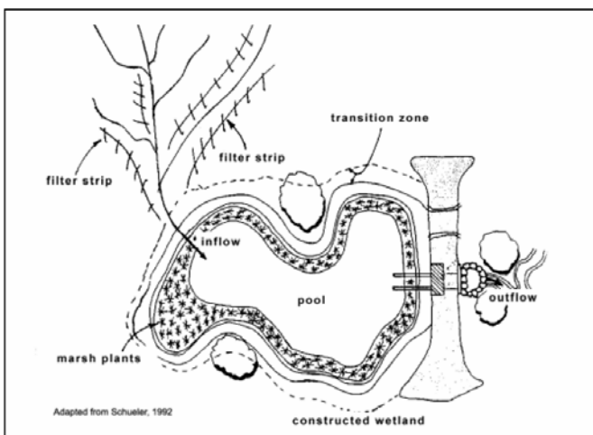
FIGURE 21 Treatment wetland design (SFWMD 2002b)
