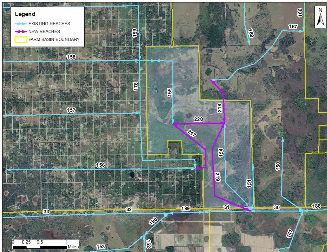
Figure 8.3: WAM Representation of the CCDD Impoundment
