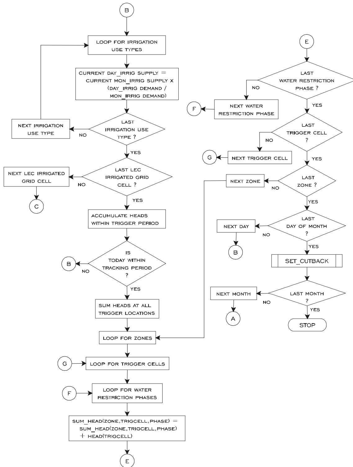
Figure F3 (cont.) Flowchart for Water Shortage Plan as Implemented in the South Florida Water Management Model
