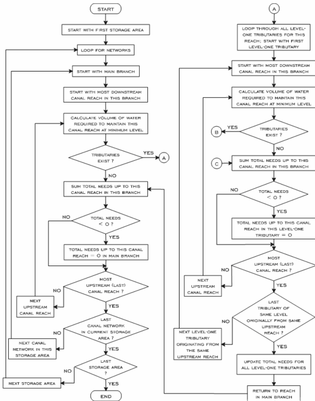
Figure F2 Flowchart for Calculating Water Supply Needs for the Lower East Coast as Implemented in the South Florida Water Management Model
