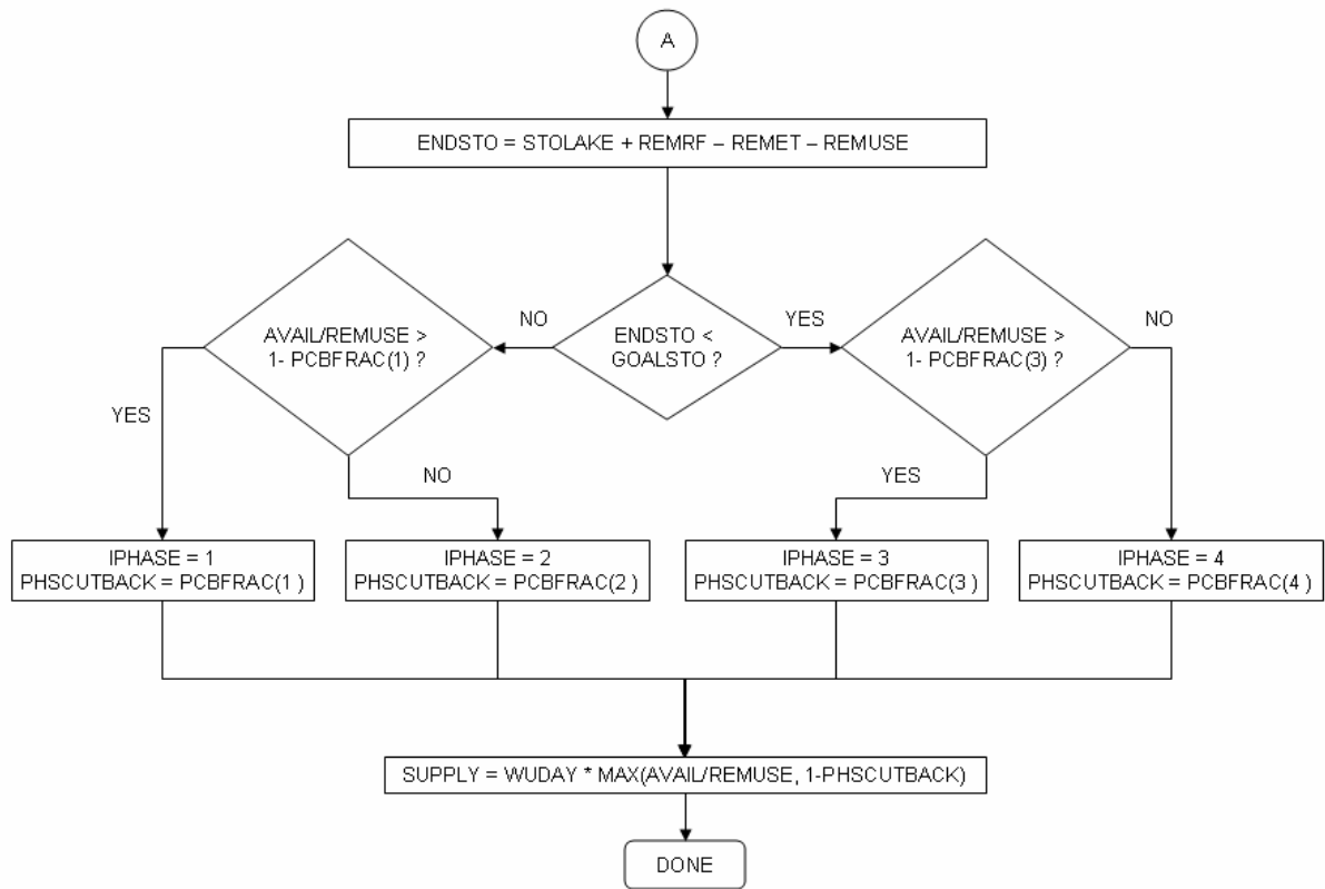
Figure F1 (cont.) Flowchart for Supply-Side Management as Implemented in the South Florida Water Management Model
