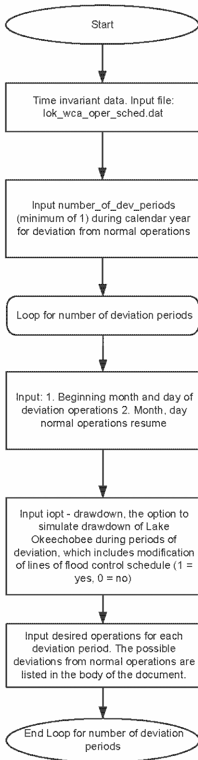
Figure F4 Methodology of Incorporating Operations Deviating from Normal for Lake Okeechobee Releases to Tidewater/Water Conservation Areas in SFWMM
