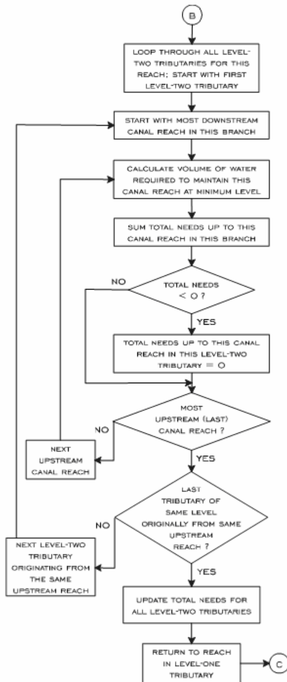
Figure F2 (cont.) Flowchart for Calculating Water Supply Needs for the Lower East Coast as Implemented in the South Florida Water Management Model
