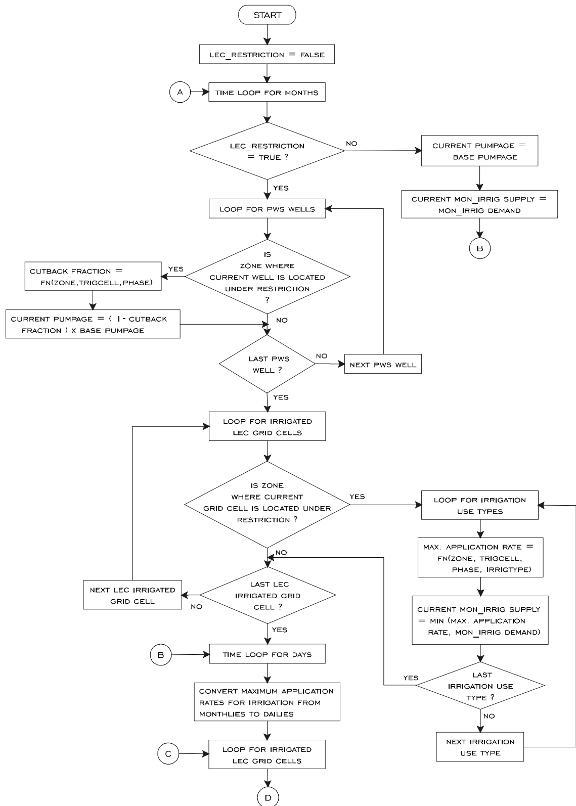
Figure F3 Flowchart for Water Shortage Plan as Implemented in the South Florida Water Management Model
