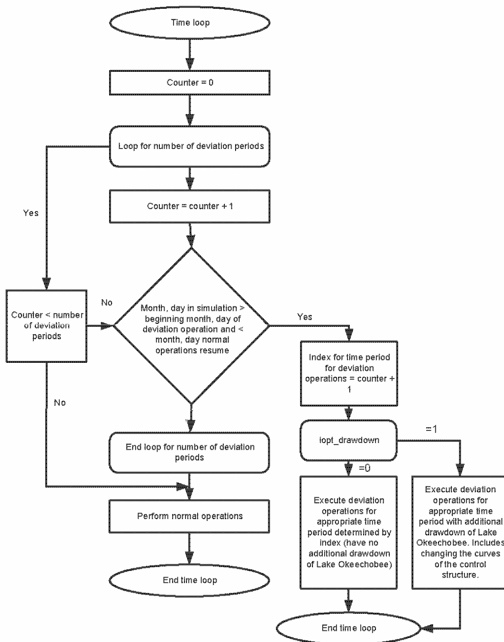
Figure F4 (cont.) Methodology of Incorporating Operations Deviating from Normal for Lake Okeechobee Releases to Tidewater/Water Conservation Areas in SFWMM.
