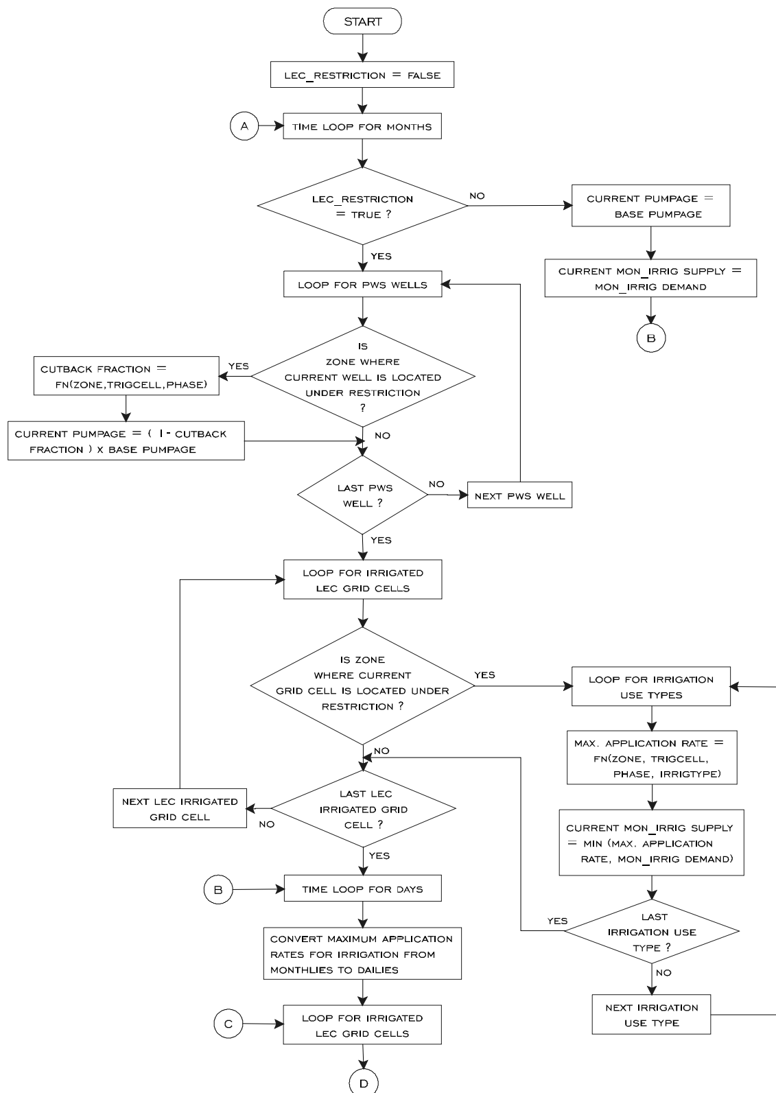
Figure F2 (cont.) Flowchart for Calculating Water Supply Needs for the Lower East Coast as Implemented in the South Florida Water Management Model
