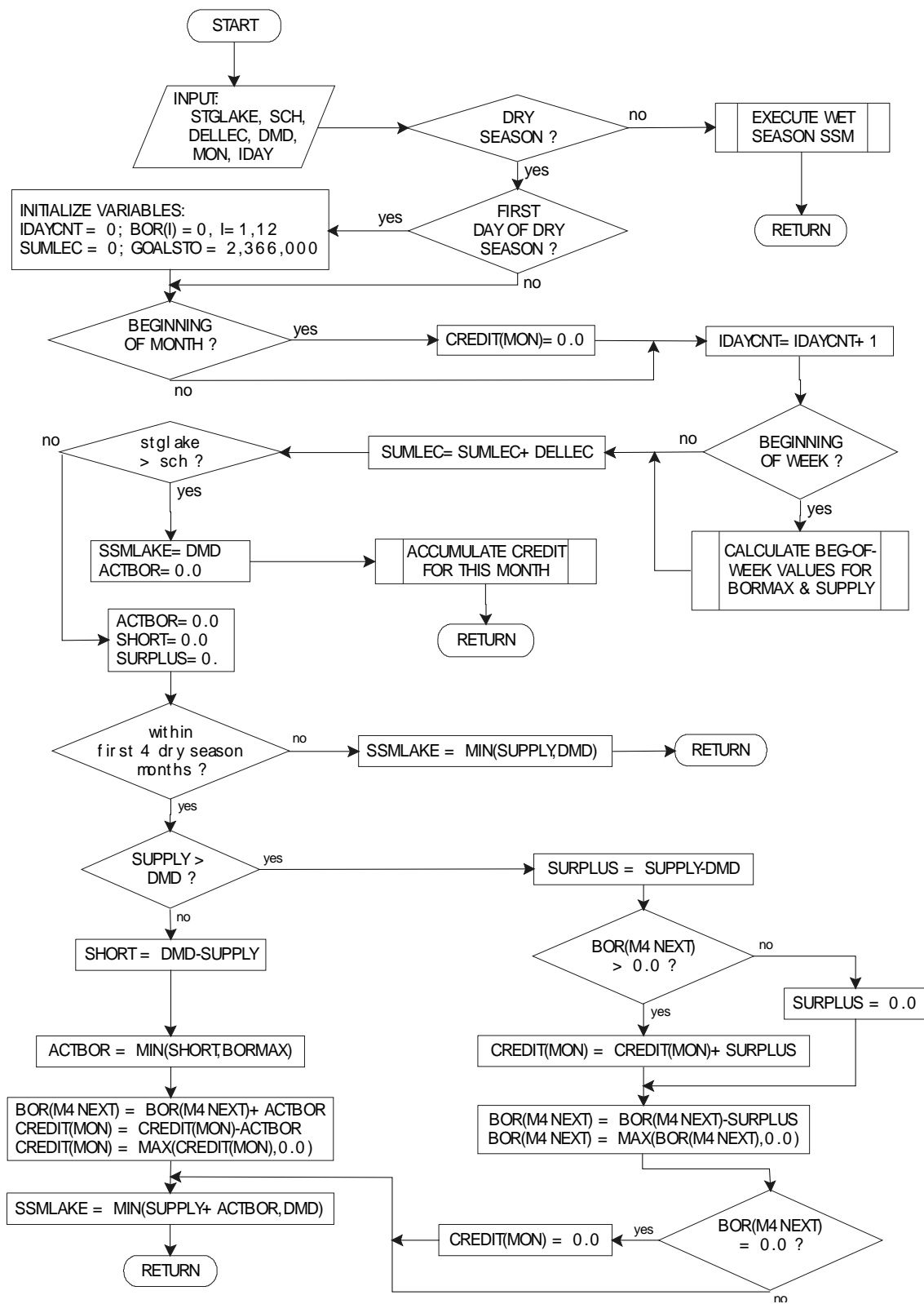
Figure F1 Flowchart for Supply-Side Management as Implemented in the South Florida Water Management Model
