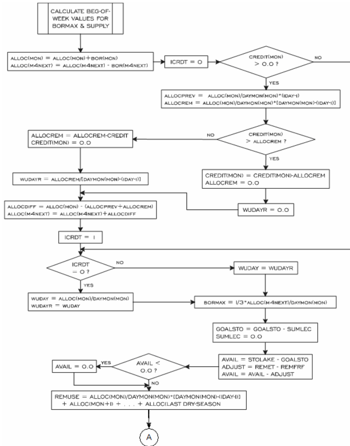
Figure F1 (cont.) Flowchart for Supply-Side Management as Implemented in the South Florida Water Management Model
