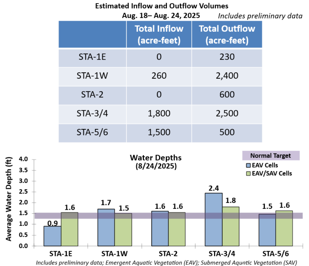
Figure S-1. STA depths and flow volumes
