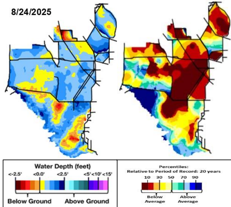
Figure EV-6. Present water depths (August 24, 2025) compared to the day of year relative to average (percentile) over the previous 20 years.
