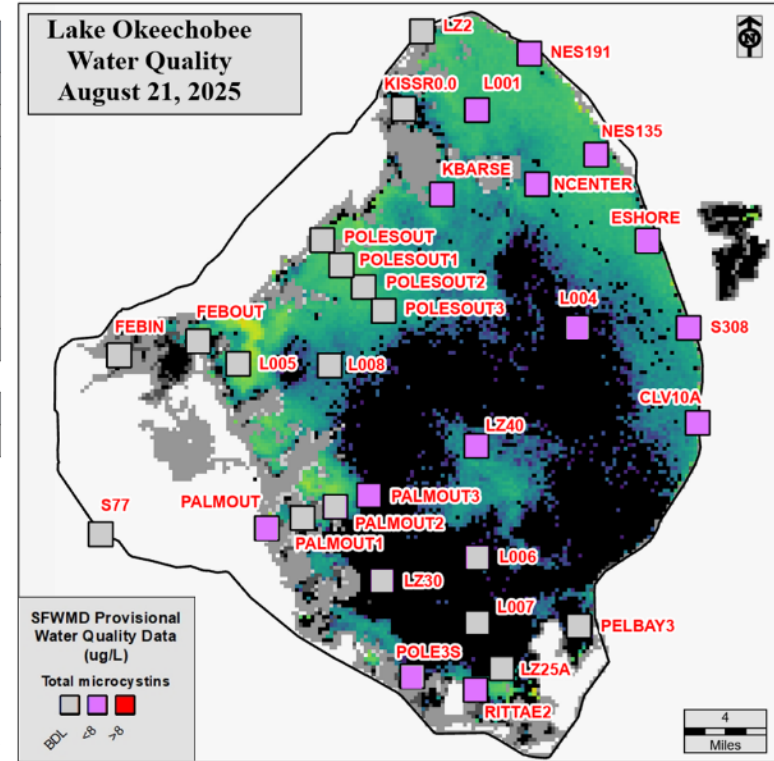
Figure LO-7. Dominant taxa, cyanotoxins (µg/L) and chlorophyll a (µg/L) concentration data from August 19 - 20, 2025. Sampling locations, chlorophyll a , and total toxin concentrations are overlaid on the August 21, 2025 image from NOAA's harmful algal bloom monitoring system. Gray color indicates cloud cover.
