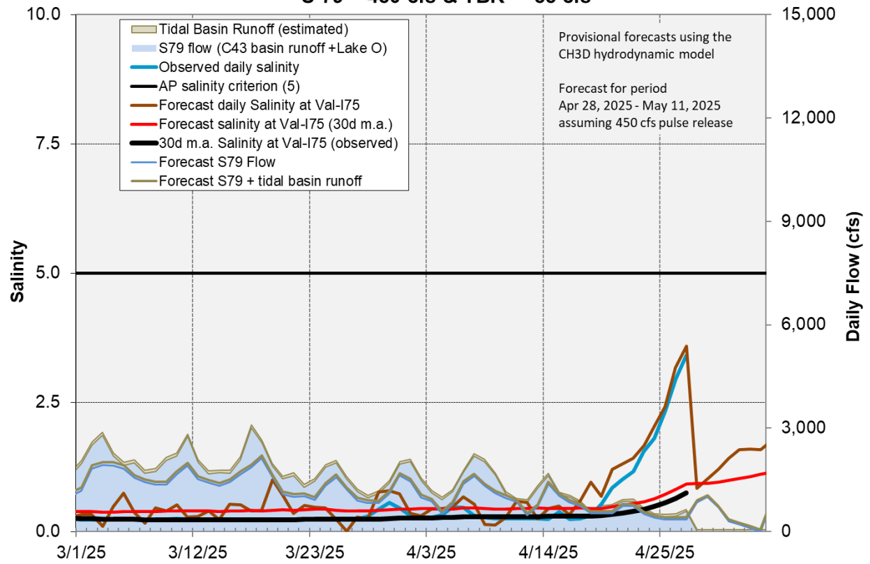
Figure ES-10. Surface salinity forecast at the Val I-75 site assuming a 450 cfs pulse release at S-79.
