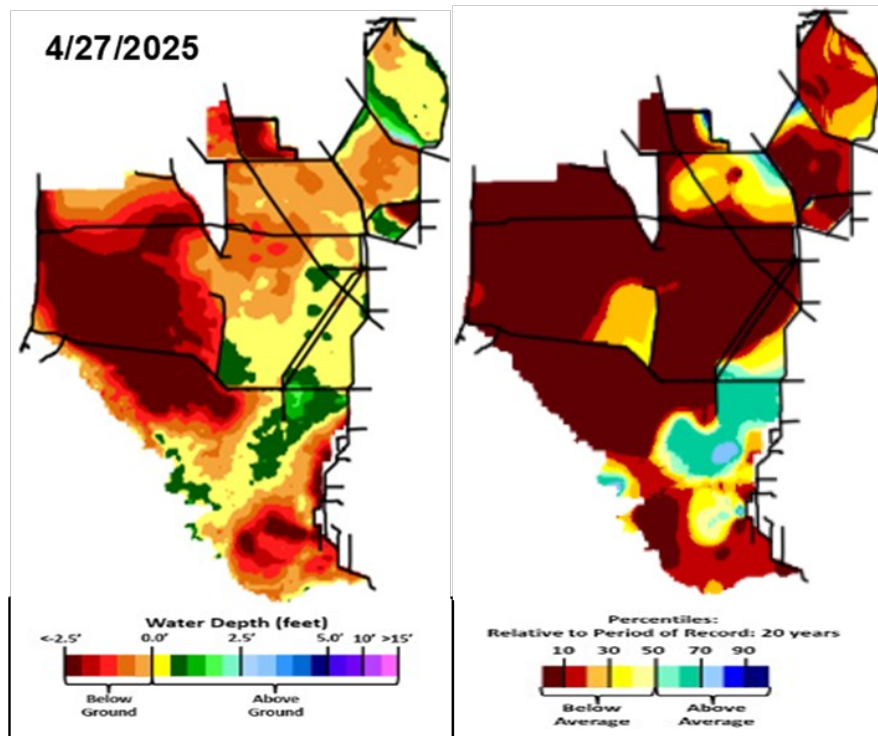
Figure EV-6. Present water depths (April 27, 2025) compared to the day of year average over the previous 20 years.
