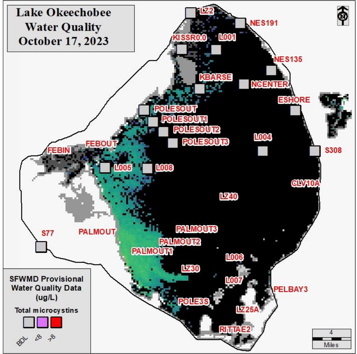
Figure LO-7. Total microcystins ( \mu\text{g/L} ) data from October 16 - 17, 2023 survey. Sampling locations are overlaid on the October 17, 2023, image from NOAA's harmful algal bloom monitoring system. Gray color indicates cloud cover.
