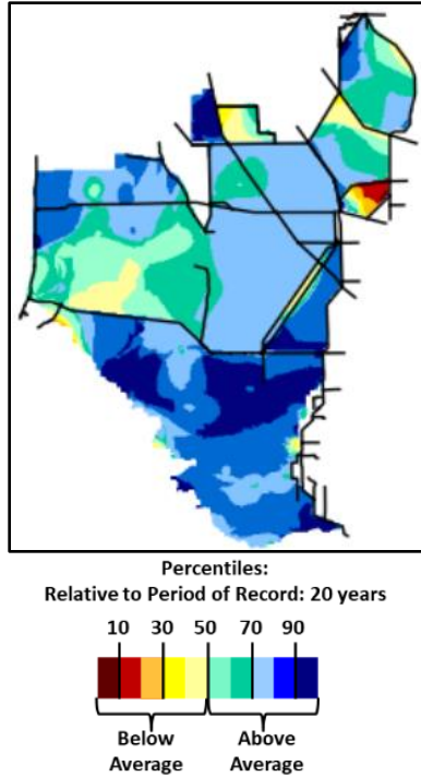
Figure EV-7. Present water depths (10/22/2023) compared to the day of year average over the previous 20 years.
