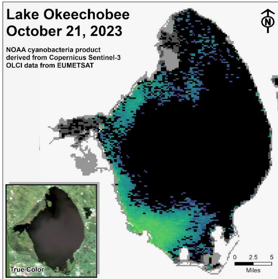
Figure LO-6. Cyanobacteria bloom index level on October 21, 2023, based on NOAA’s harmful algal bloom monitoring system. Gray color indicates cloud cover.
