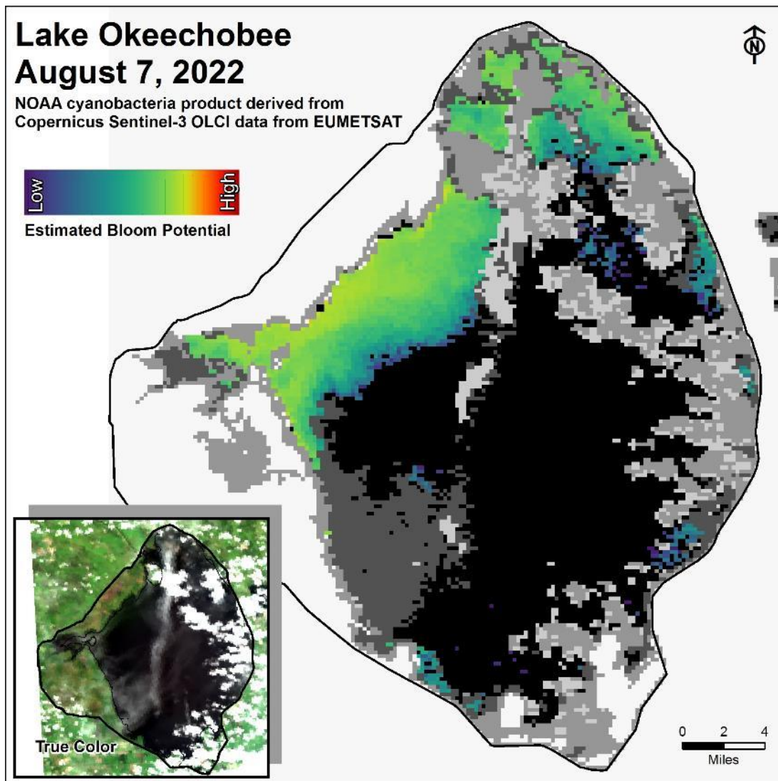
Figure LO-6. Cyanobacteria bloom potential on August 7, 2022 based on NOAA's harmful algal bloom monitoring system. Gray color indicates cloud cover.
