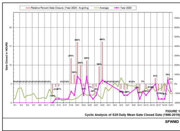
Figure 8-2: Relative Percent Gate Closure Times during the 2020 High Tide Season.
