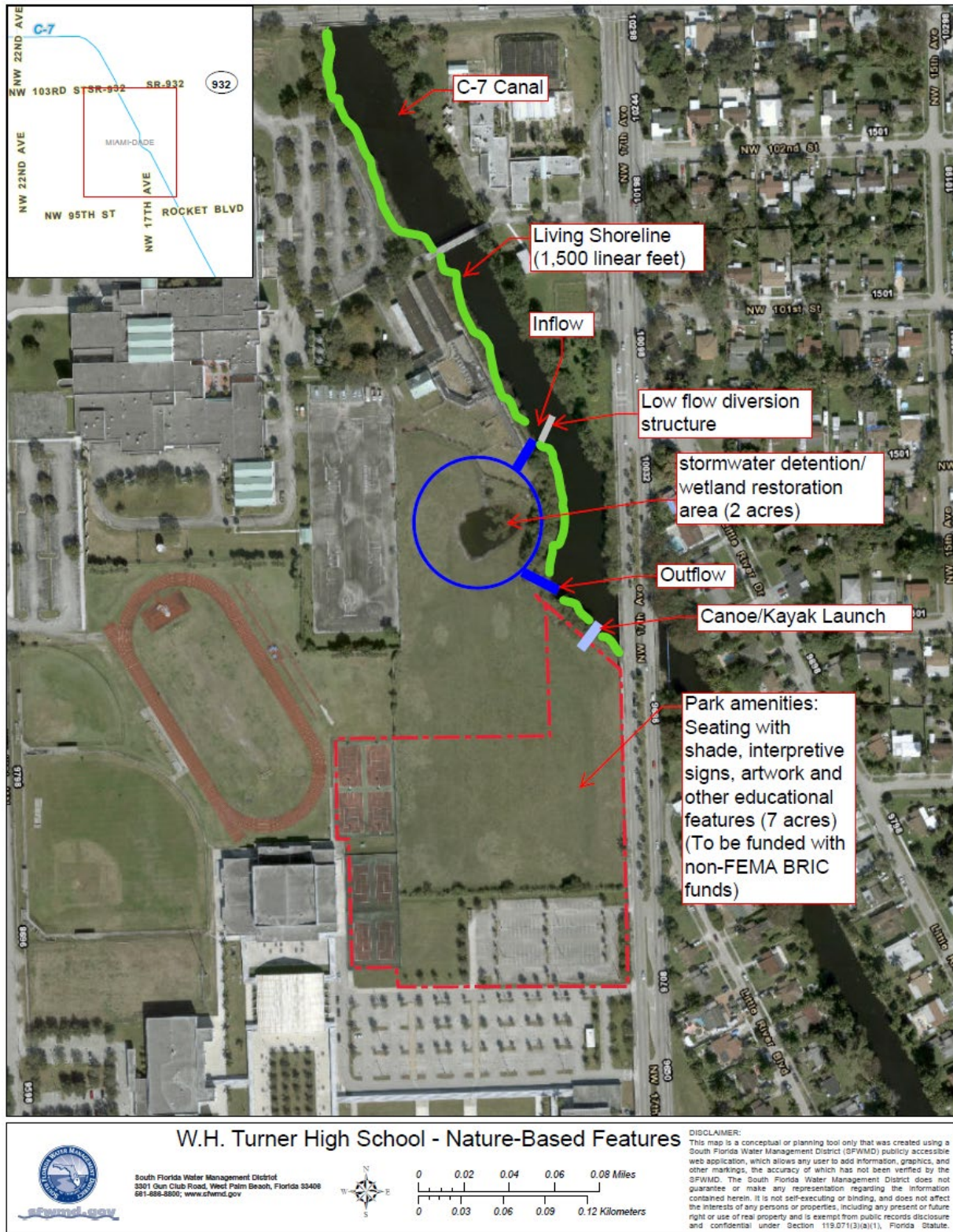
Figure 9-15: Nature-based features at W.H. Turner High School
