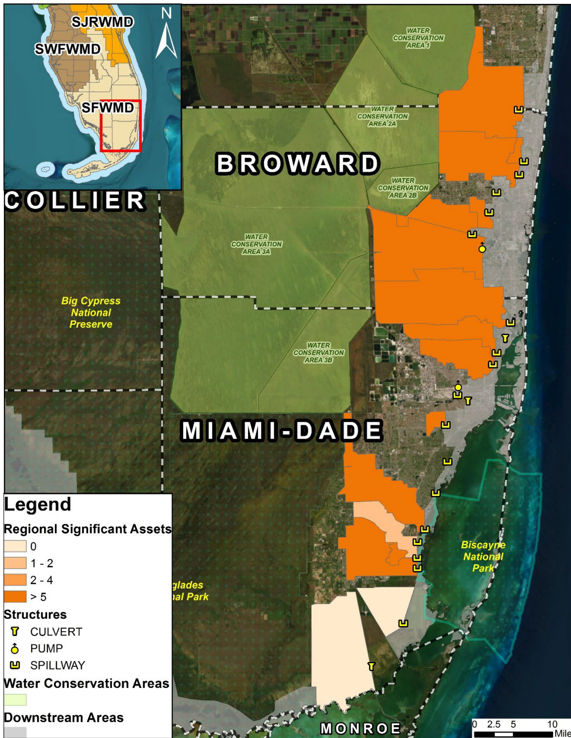
Figure 8-17: Regional Significant Assets per Coastal Structures Resiliency Project Impact Areas, utilized as part of the Resiliency Projects Ranking Criteria Set 2
