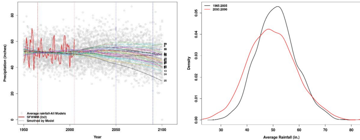
Figure 6. Time Series of gridded average rainfall for all climate models in the LOCA dataset. Also shown is the SFWMM (2x2) average rainfall and smoothed PRCPTOT for each model.
