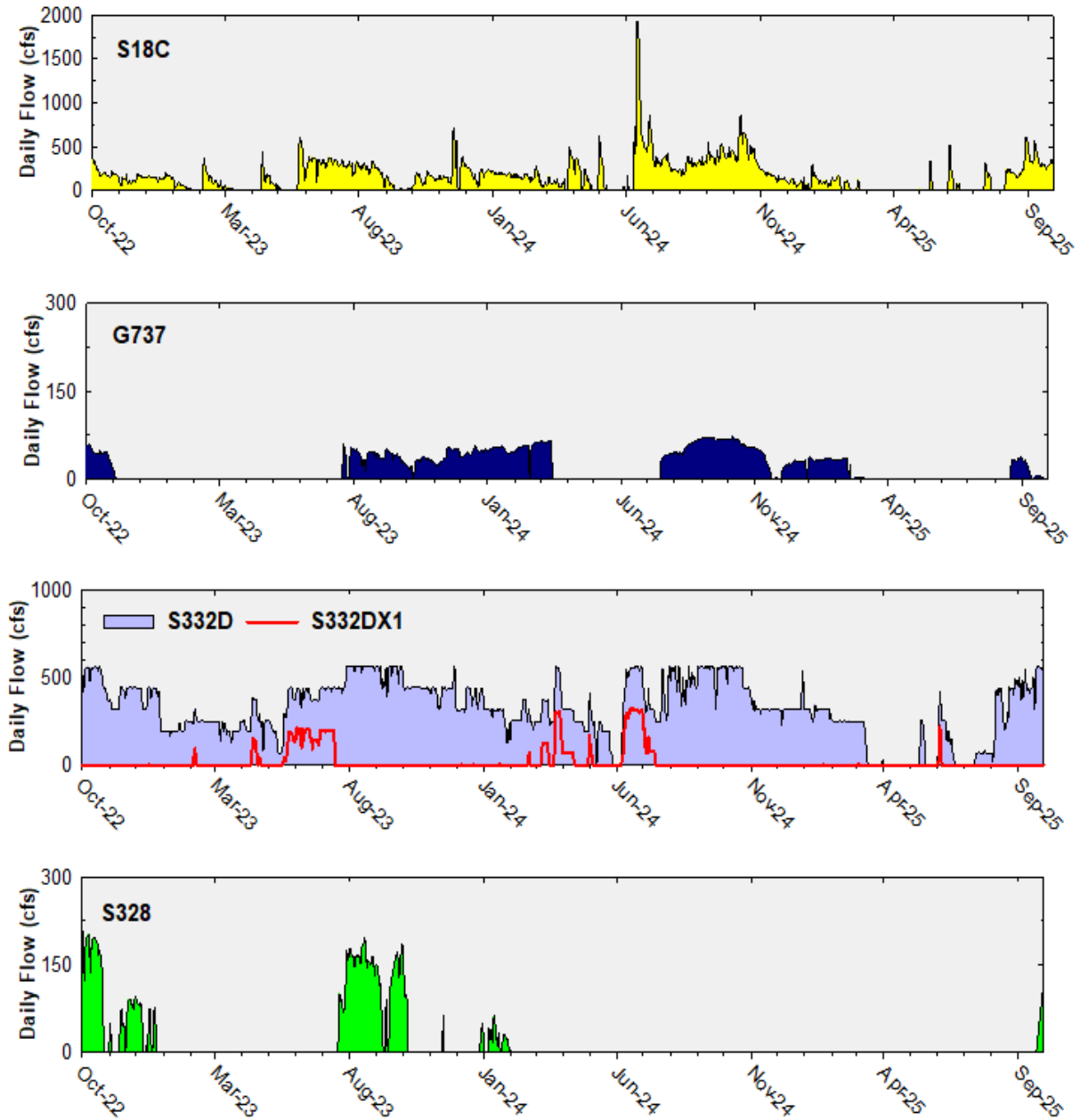
Figure 10. Daily flows in cubic feet per second (cfs) at individual Taylor Slough and Coastal Basins structures into ENP.
