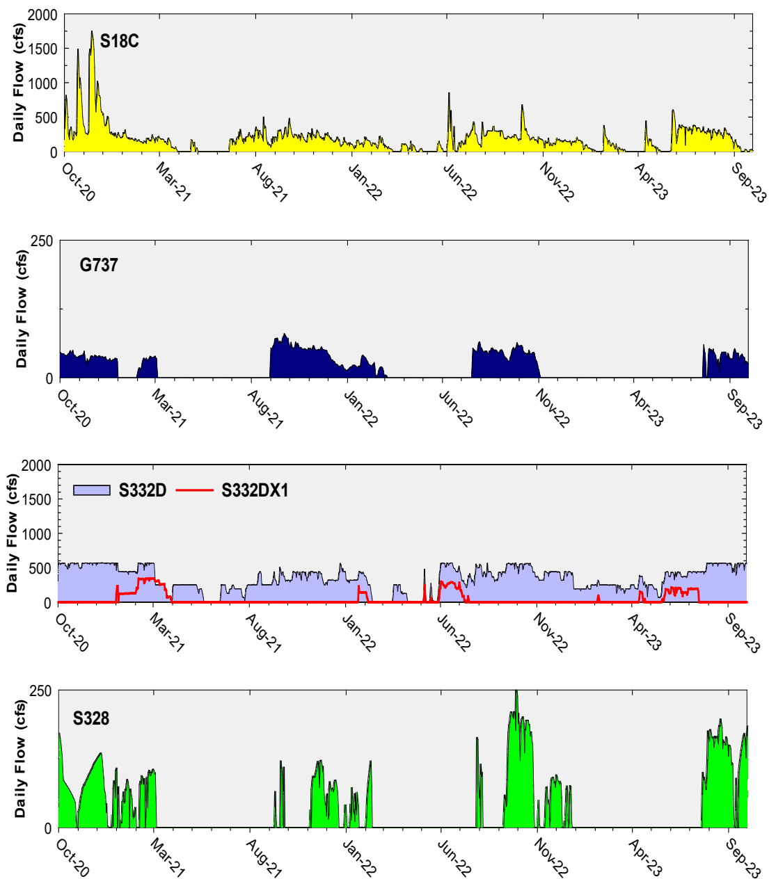
Figure 10. Daily flows in cubic feet per second (cfs) at individual Taylor Slough and Coastal Basins structures into ENP.
