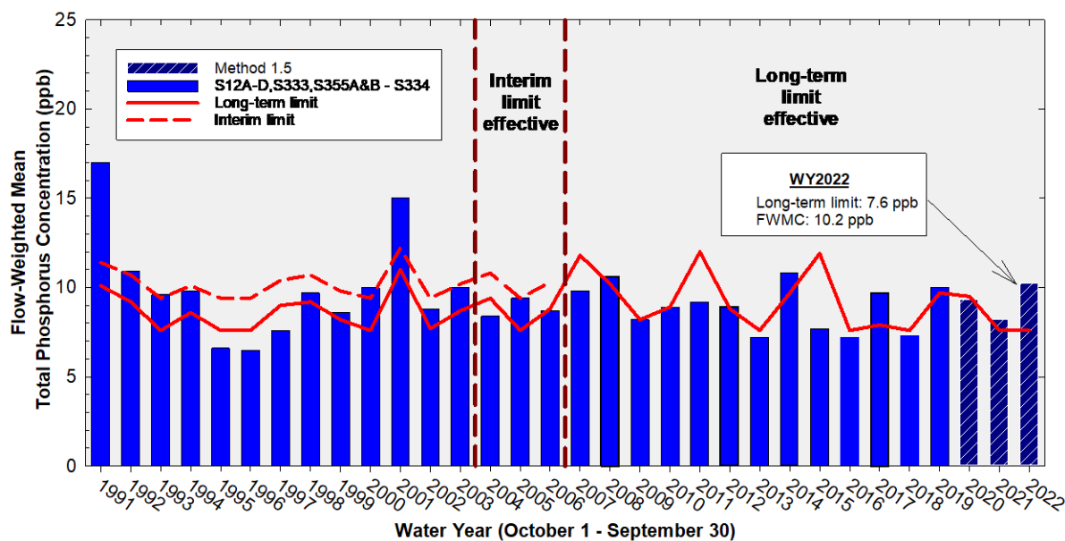
Figure 5. The 12-month TP FVMCs at inflows to ENP through Shark River Slough at the end of each water year compared to the interim and long term total phosphorus limits through WY2022.
