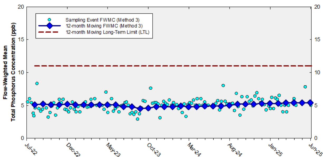
Figure 7. The 12-month tracking TP FVMCs in inflows to ENP through Taylor Slough and Coastal Basins at the end of each month and the sampling event TP FVMCs.
