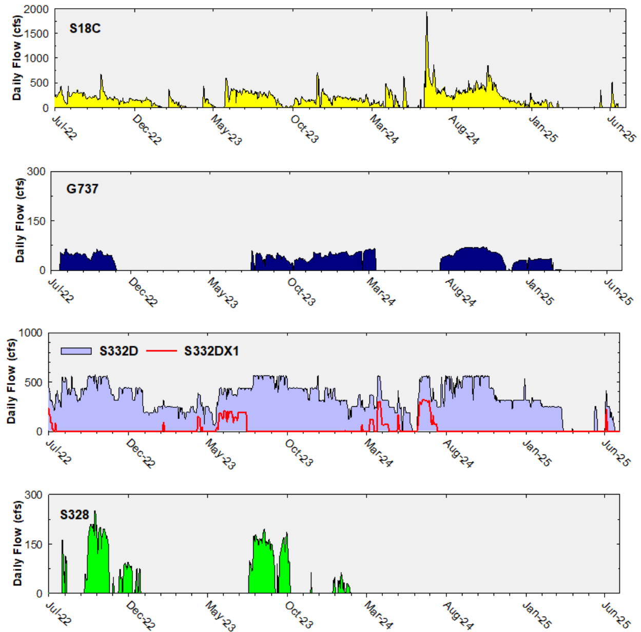
Figure 10. Daily flows in cubic feet per second (cfs) at individual Taylor Slough and Coastal Basins structures into ENP.
