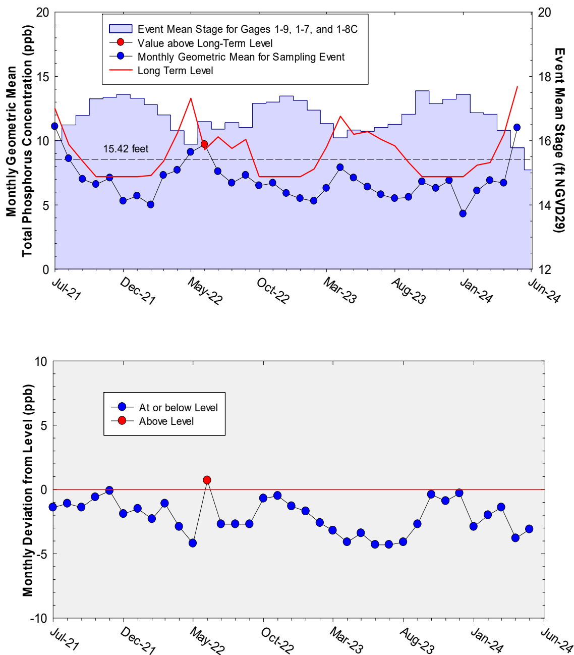
Figure 3. Top: Monthly TP geometric mean concentrations for the Refuge compared to calculated long-term levels, which are adjusted for fluctuations in stage. The geometric mean TP concentration was above the long-term level in June 2022. Bottom: Deviation of monthly geometric mean TP concentrations from calculated long-term levels. Negative values indicate that the geometric mean was lower than the long-term level.
