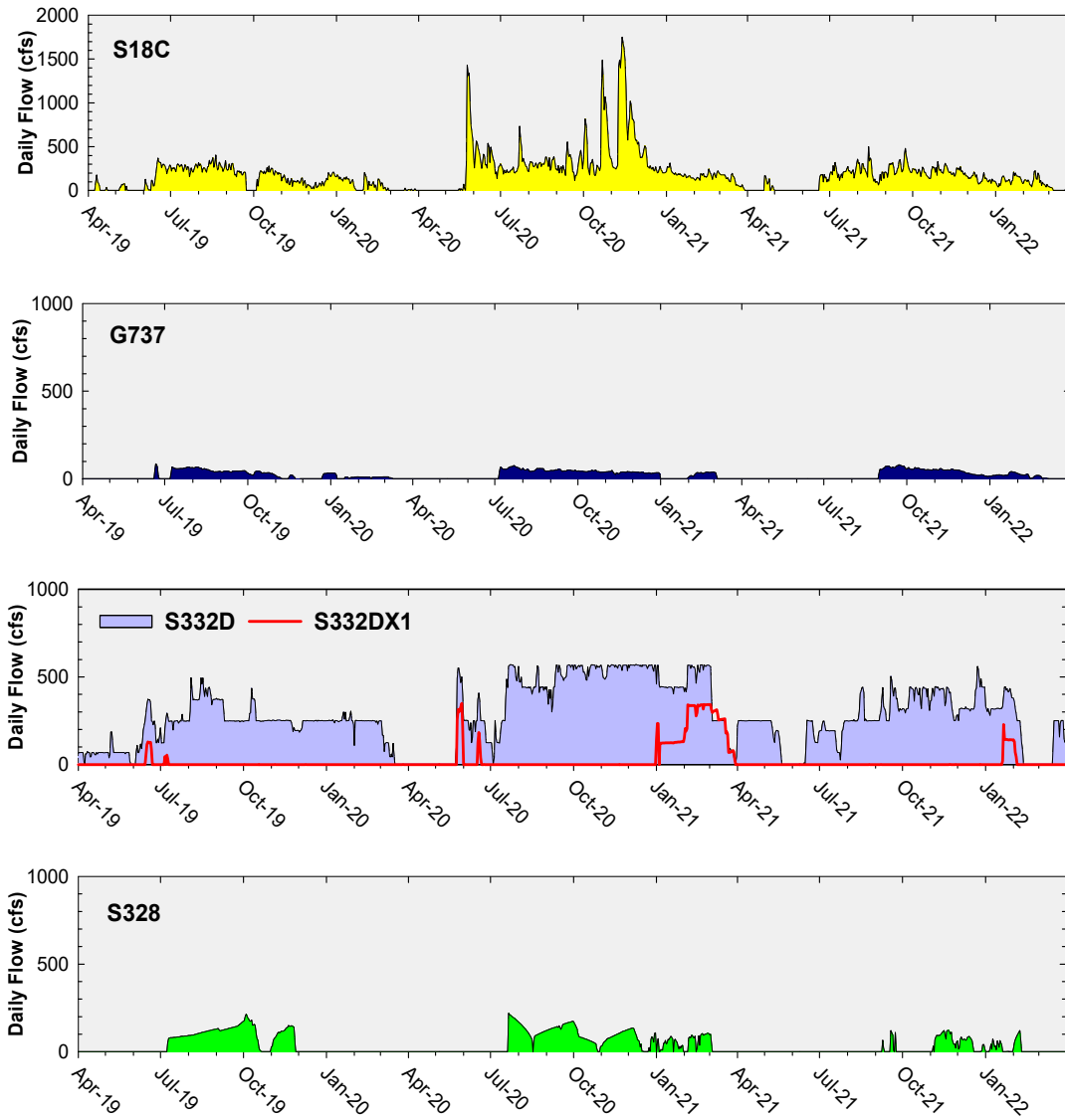
Figure 9. Daily flows in cubic feet per second (cfs) at individual Taylor Slough and Coastal Basins structures into ENP. G737 flow prior to October 1, 2018, is based on S200 pump flow on days when the G737 gates were open. Daily flow data are missing for S18C from September 23 to 30, 2019.
