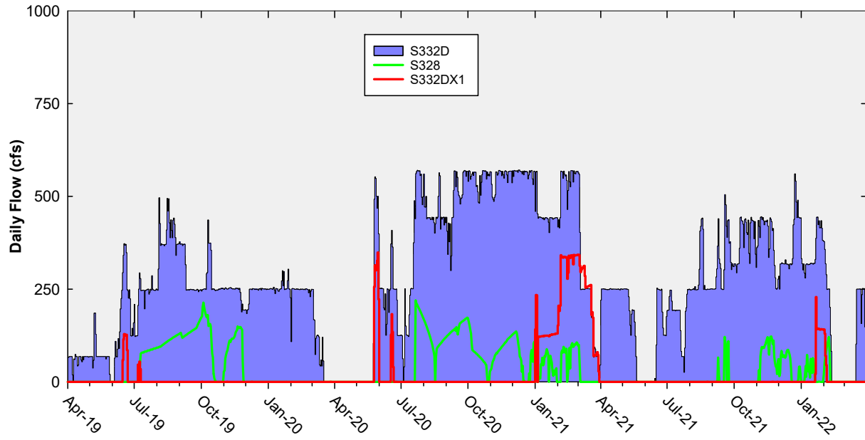
Figure 8. Daily flows into the detention area from the S332D pumps and monitored flow out of the detention area at two downstream structures.
