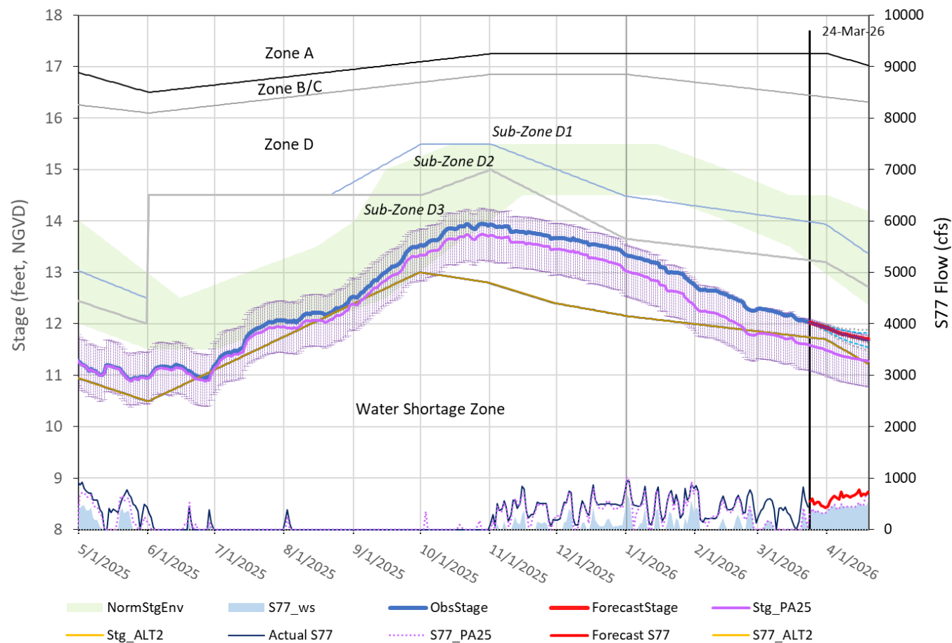
LAT-forecasted Lake Okeechobee stage and S-77 flows with 250 cfs target at S-79 and 0 cfs at S-80.
