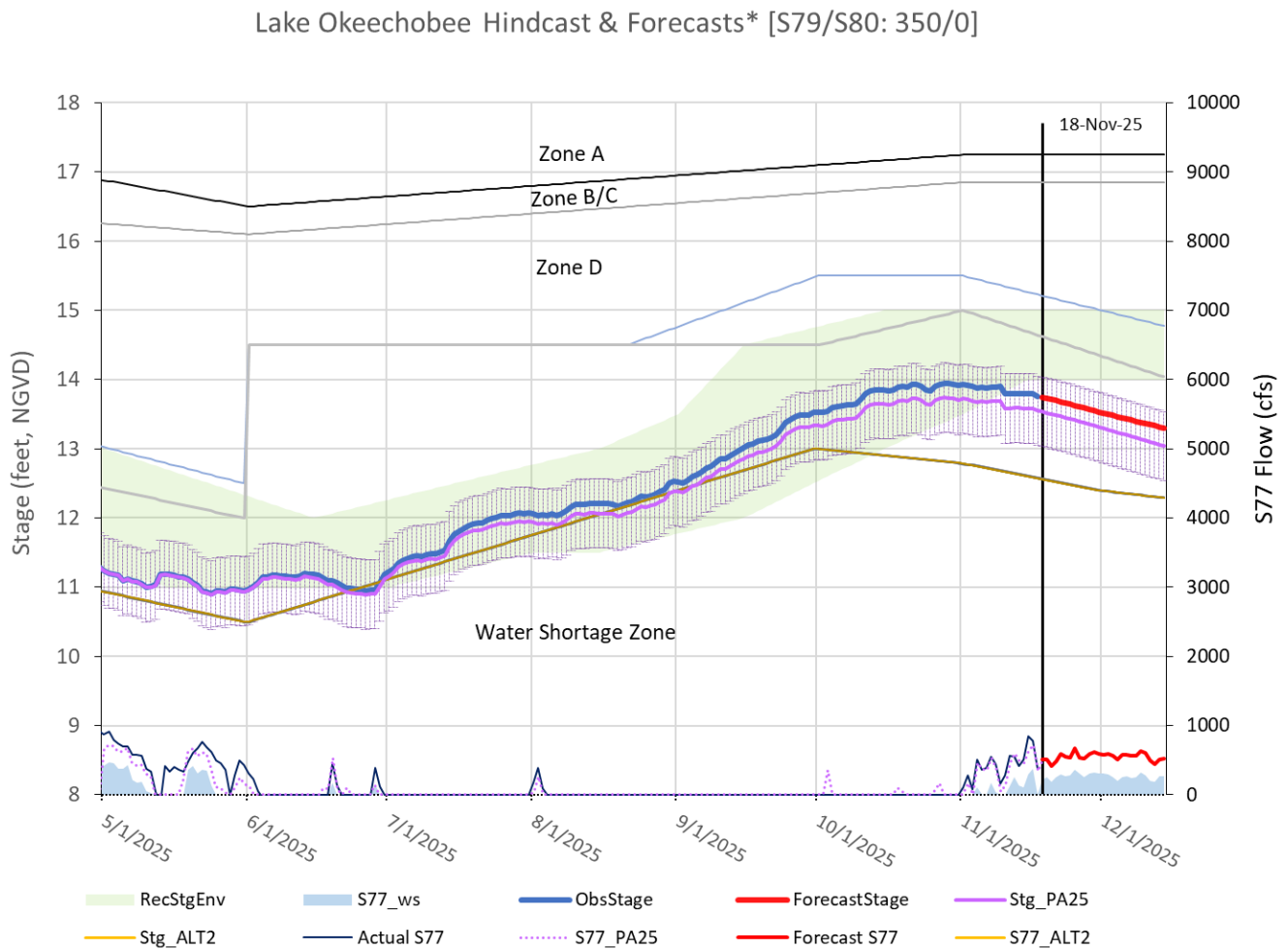
LAT-forecasted Lake Okeechobee stage and S-77 flows with 350 cfs target at S-79 and 0 cfs at S-80, without considering Recovery Operations in the PA25 simulation.
