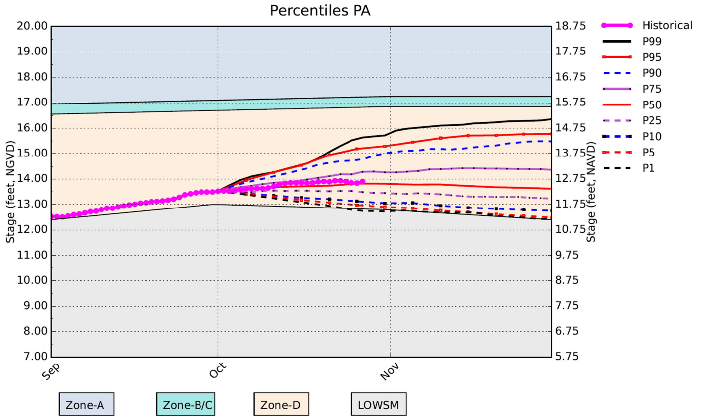
Lake Okeechobee Oct 01 Conditional Position Analysis (PrefSce)
