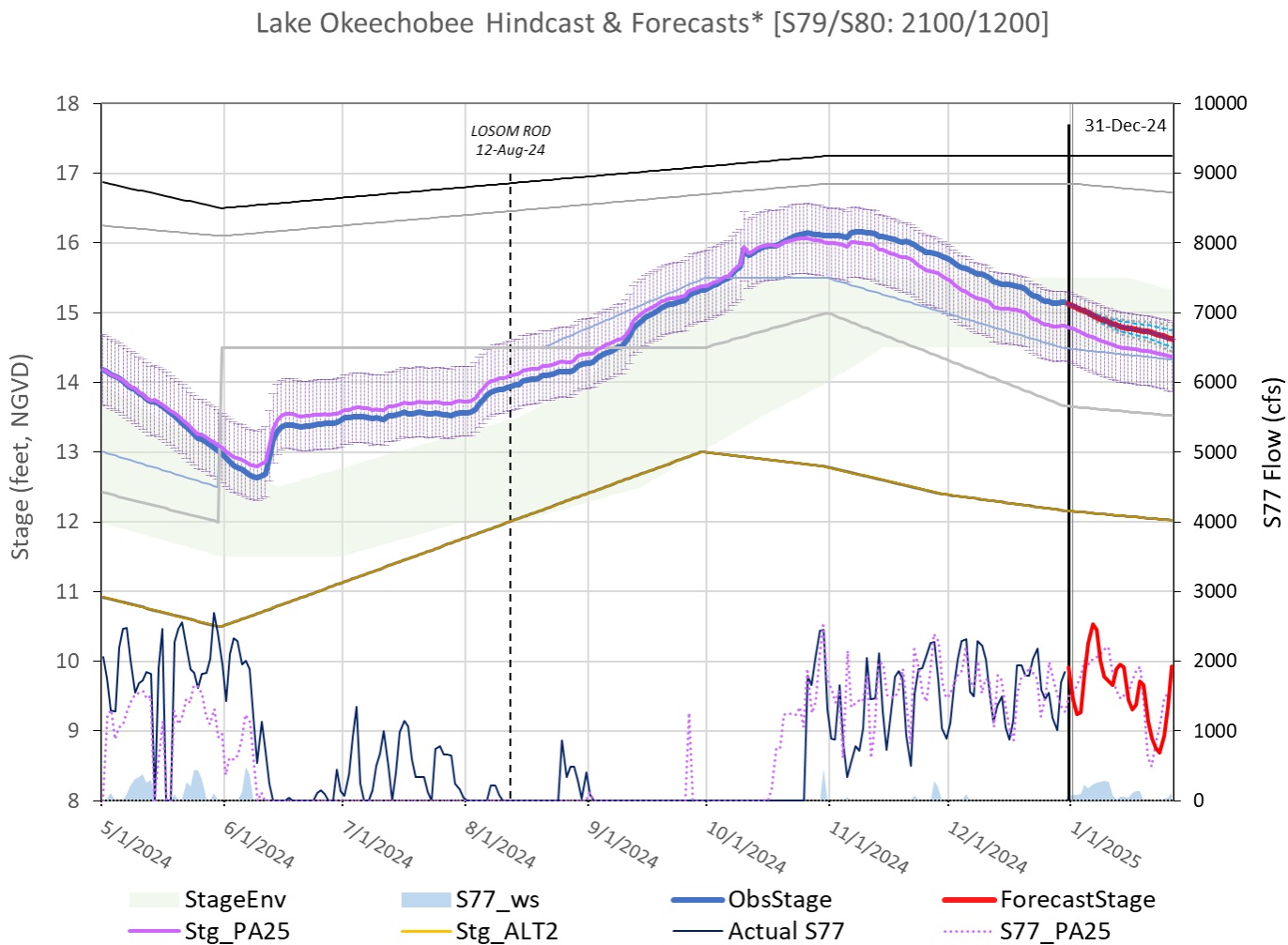
LAT forecasted Lake Okeechobee stages and S-77 flows with 2100 cfs flow target at S-79 and 1200 cfs flow target at S-80 consistent with recovery operations
