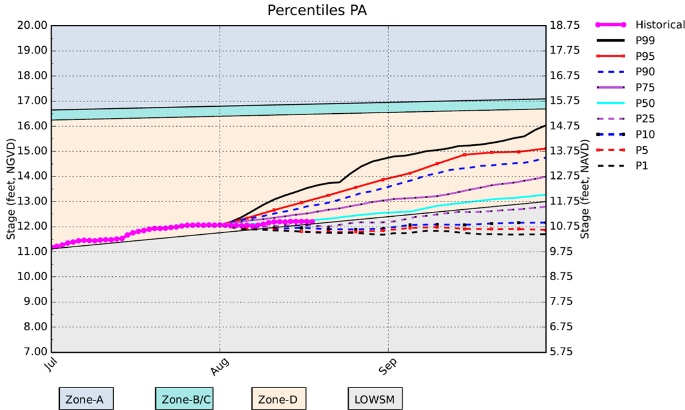
Lake Okeechobee August 01 Conditional Position Analysis (PrefSce)
