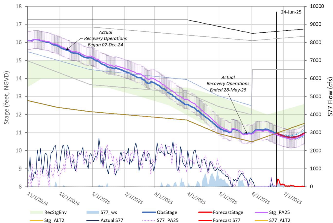
(a) LAT-forecasted Lake Okeechobee stage and S-77 flows with 350 cfs target at S-79 and 0 cfs at S-80, with Recovery Operations included in the PA25 simulation between 12/7/2024 and 5/28/2025.
