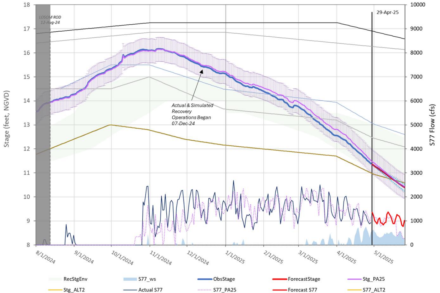
Lake Okeechobee Hindcast &amp; Forecasts* [S79/S80: 650/0]
