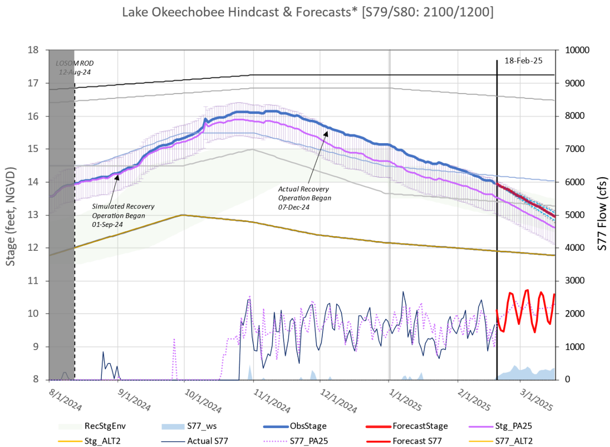
LAT forecasted Lake Okeechobee stages and S-77 flows with 2100 cfs flow target at S-79 and 1200 cfs flow target at S-80 consistent with recovery operations. PA25-simulated recovery operations are initiated on September 1 st , 2024, resulting in observed and forecasted stages tracking above the PA25 simulation line.
